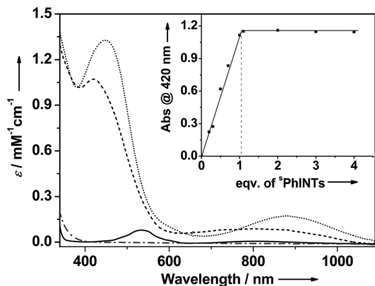
Fig. 1 Main: Electronic spectra of 1 (solid trace), 5 PhINTs (dash-dotted trace), 2 (dashed trace), and 2-Sc (dotted trace) in acetone at -40 °C. Inset: Plot of the absorbance of the 420 nm band of 2 against the equivalents of 5 PhINTs added to 1 . Notably, 2 and 2-Sc can also be generated in \text{CH}_2\text{Cl}_2 with \lambda_{\text{max}} [ \epsilon_{\text{max}} ] values identical to that observed in acetone.
