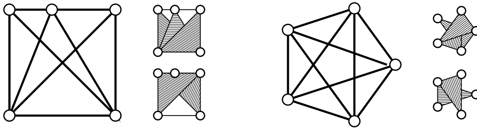
Figure 1: Constructing a set of n points with n maximum area triangles
