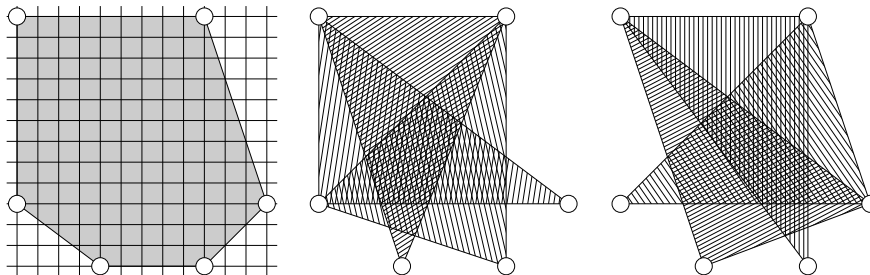
Figure 3: A nontrivial example with many maximum area triangles
