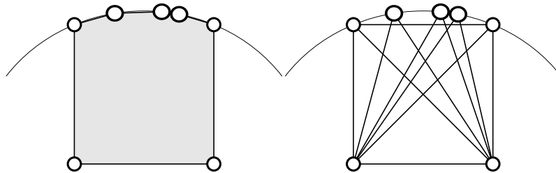
Figure 2: Constructing a set of n points with n maximum perimeter triangles
