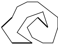
Figure 8: A cyclic merge which is simple but not angle consistent.
