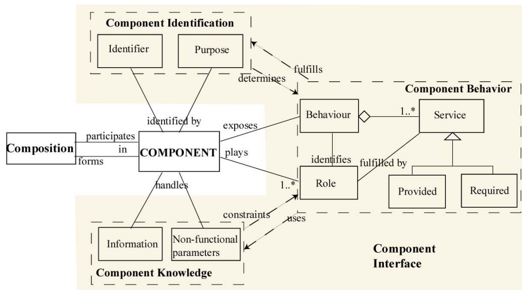
Figure 2. Component metamodel.
