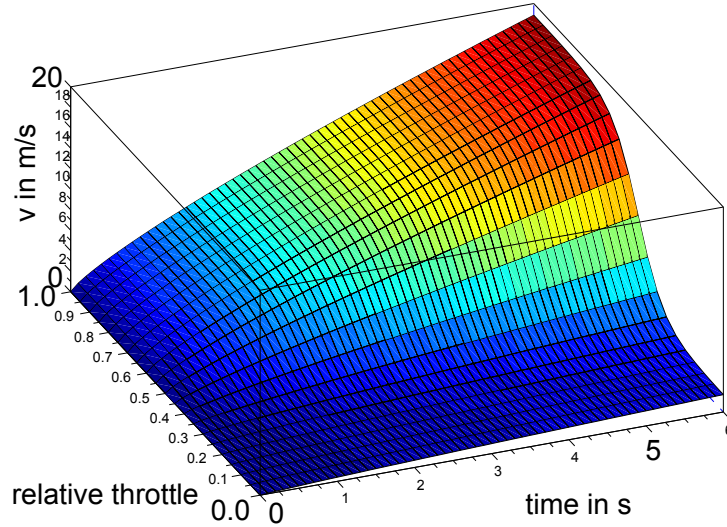
Fig. 18. Approximated velocity function over time and over relative throttle values.
