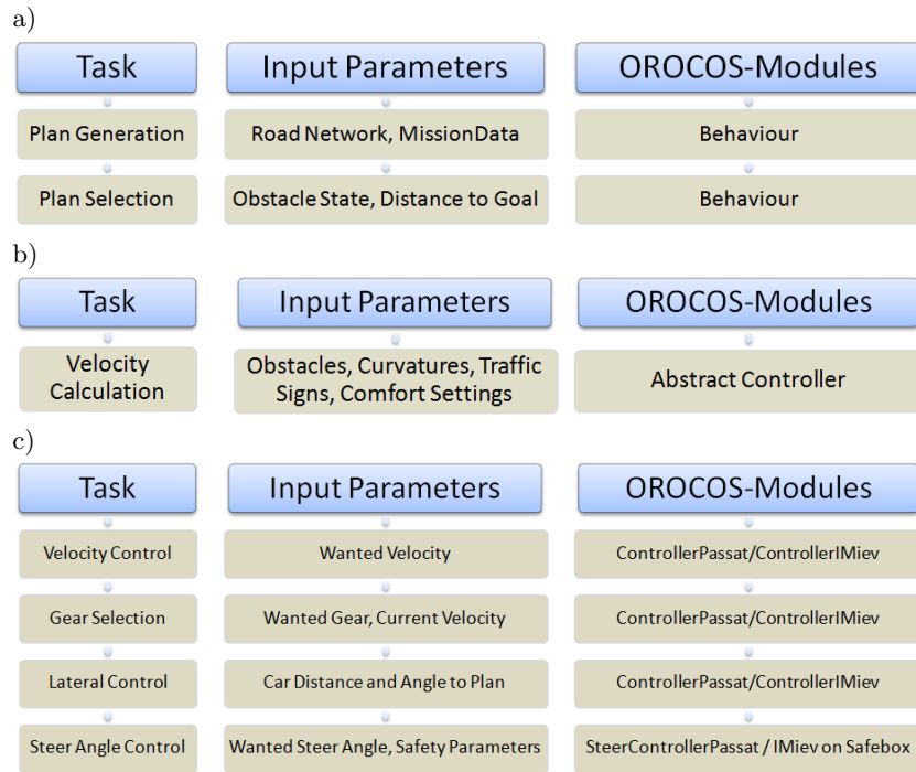
Fig. 2. Controller and behavior models. a) For these models, code and data are vehicle independent. b) Code is vehicle independent but not data independent. c) These modules are designed for a certain vehicle (VW Passat (MiG)).
