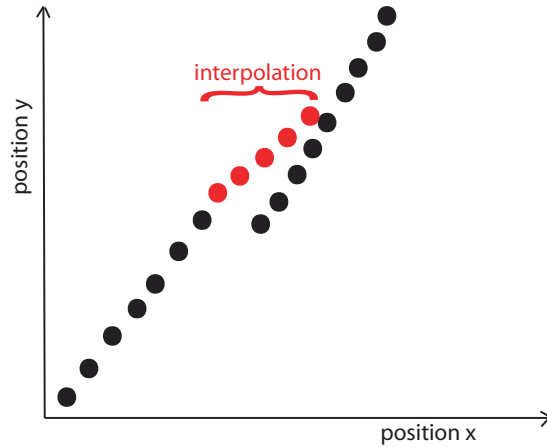
Fig. 9. Ego state over time from bottom left to top right. Suddenly an ego state jump occurred, was recognized by the controller. The jump in interpolated within a certain time, a useful value was t = 2s .
