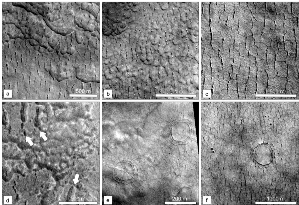
Figure 13.4.: Examples of landforms in western Utopia Planitia. [a] Polygonal terrain with preferred N-S orientation of pits along cracks. Asymmetric ("scalloped") small depressions have steep north-facing scarps (compare with figures 13.3a-b). MOC R11-00336, center at 45.47°N and 81.1°E. [b] Similar to figure 13.4a. MOC E11-02077, center at 45.4°N and 81.44°E. [c] Uniform polygons with preferred N-S orientation. MOC Mo4-02704, center at 44.08°N, 84.15°E. [d] Interior of 8.8-km impact crater. Note the N-S-oriented cracks, which are bounded by U-shaped troughs (arrows in upper left and lower right parts of image). See text for details. MOC R17-00802, center at 47.62°N and 82.57°E. [e] Polygonal pattern locally modified into concentric and radial pattern. The circular cracks in the mantling material might have formed by differential compaction (see Buczowski and Cooke (2004) , although these authors describe much larger craters), which creates a zone of structural weakness over crater rims. MOC Ro5-00393, center at 42.02°N and 80.95°E. [f] Similar as in figure 13.4e, concentric cracks might indicate position of mantled impact crater. MOC Eo4-01564, center at 41.63°N, 82.89°E.
