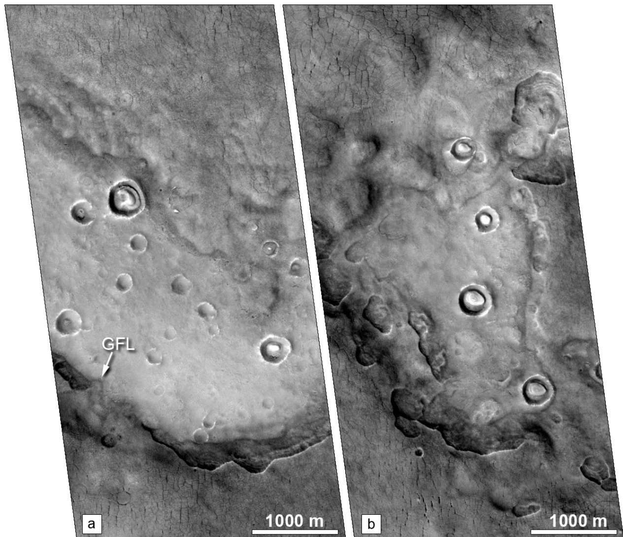
Figure 13.3.: Examples of landforms in western Utopia Planitia. [a] Asymmetric topographic depression with steep southern scarp and more gradually rising northern margin. The floor of the depression displays impact craters, which are partly filled by layered material. The mantling material is characterized by polygonal terrain. MOLA track (ap198261) shows that the mantling material is about 80 m thick. The degraded appearance of the southern scarp in the lower left part of the image might indicate a gelifluction lobe (GFL). MOC Eo4-01564, center at 41.46°N, 82.92°E. [b] Very similar asymmetric depression, with steep southern and gently rising northern margin. MOC Eo4-01564, center at 42.08°N, 82.81°E.
