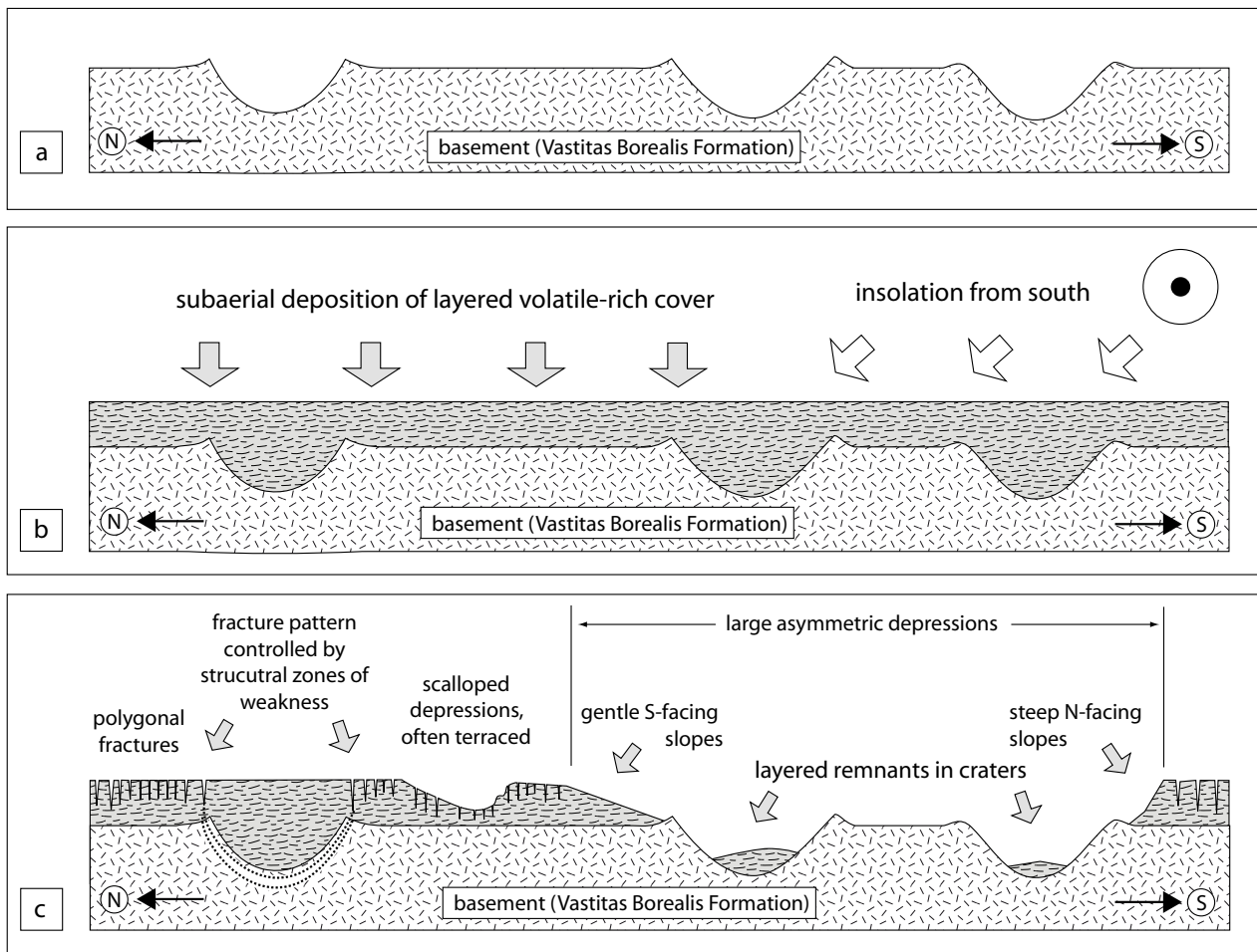
Figure 13.11.: Schematic model for landscape genesis in western Utopia Planitia. [a] Cratered basement, probably the Vastitas Borealis Formation (Tanaka et al. , 2005). [b] Subaerial deposition of a volatile-rich mantling material (ice-dust mixture). Insolation comes mainly from southern directions. [c] The sublimation of pore ice causes volume loss and the formation of polygonal crack patterns, smaller scalloped depressions, and larger depressions which affect the entire thickness of the mantling material. The depressions appear asymmetric in cross-sectional N-S profiles, since the increased insolation on south-facing slopes leads to enhanced disintegration of the ice-dust mixture and to slope failure.
