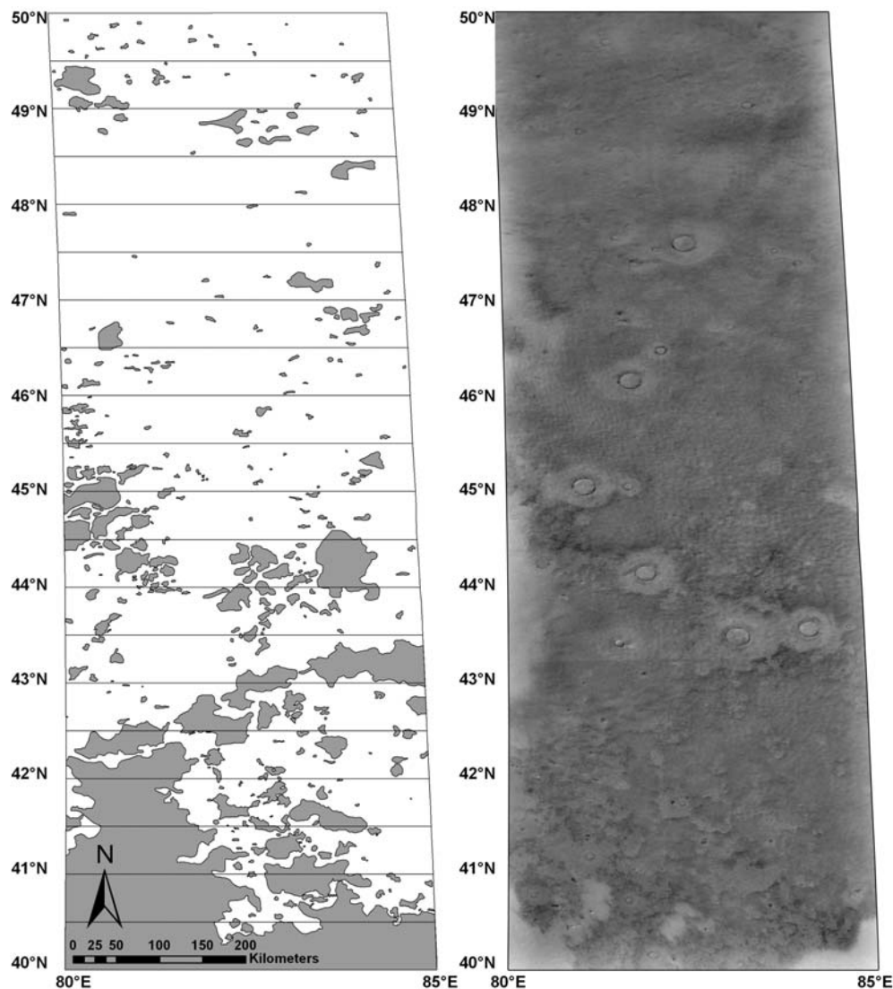
Figure 13.8.: GIS-based map of topographic depressions (gray areas) in mantling material. Our results indicate an increasing area of depressions (i.e., increasing degradation) from North to South, possibly indicating a climatic control of the degradation process; right: HRSC nadir scene of orbit 1530.
