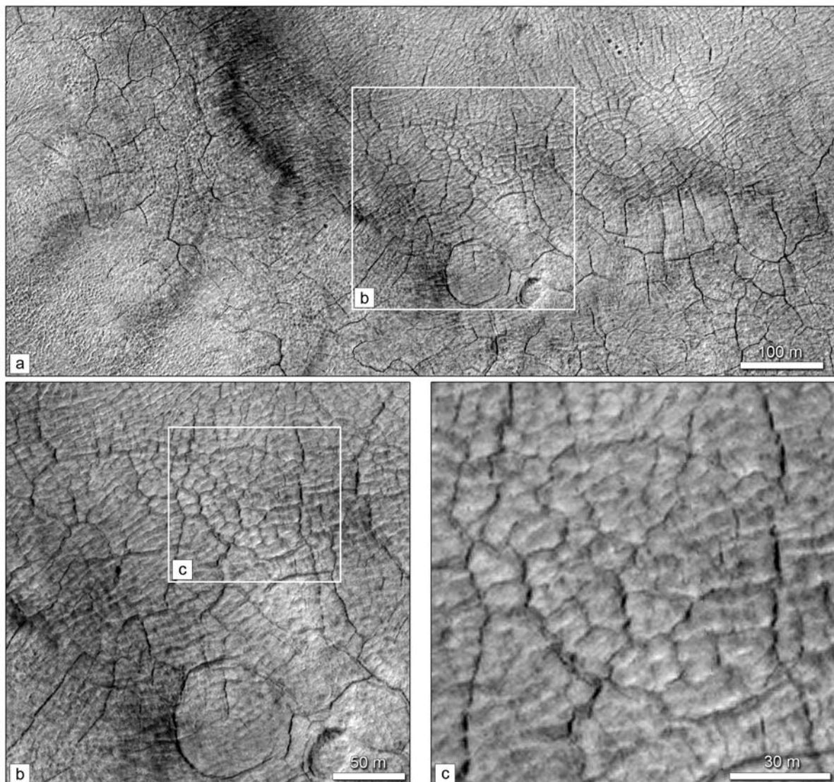
Figure 13.6.: High Resolution Imaging Science Experiment (HiRISE) image scene TRA_000823_1720_RED, 25 cm/pixel, sinusoidal map projection, located at 46°N and 92°E. Small-scaled polygons \leq 10 m inside scalloped depressions suggest different polygon generations when compared to other generations outside the scalloped depressions; polygon formation was probably (still) active after formation of depressions.
