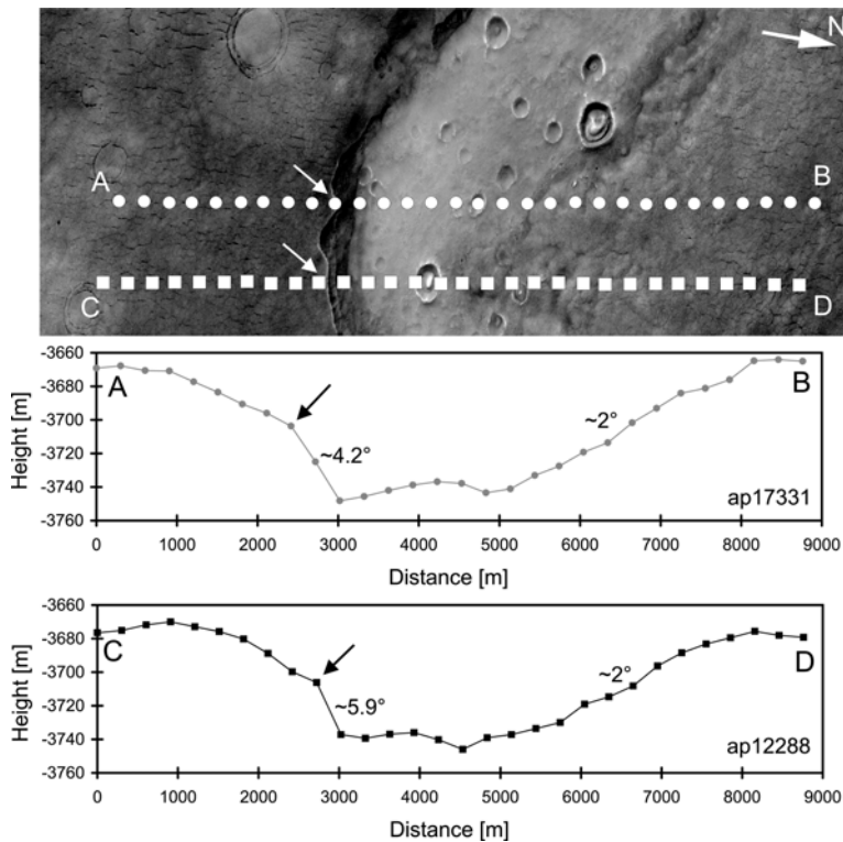
Figure 13.5: Two MOLA transects (ap17331 and ap12288) across a depression (MOC image Eo4-01564 at 41.46°N, 82.92°E; image height is 3.19 km). The top of the steeper southern scarp is labeled in the image and in the graphs with arrows. The slopes of the southern scarp are around 5°, in contrast to the more gradually rising northern margin with slopes up to ~2°.
