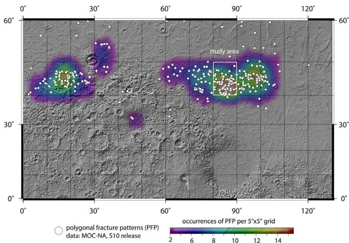
Figure 13.1.: Location of study area in the western Utopia Planitia area, white dots mark occurrences of polygonal fracture patterns suggestive of thermal contraction cracking, isodensities of occurrences are calculated in a 5^\circ \times 5^\circ grid. Note also occurrences of possible contraction features near to 30^\circ latitude, more south than anticipated earlier by other workers (Kuzmin and Zabalueva, 2003; Mangold et al., 2004).
