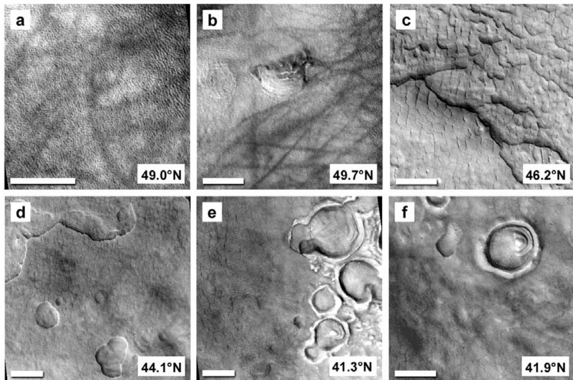
Figure 13.7: Latitude-dependent degradation features in western Utopia Planitia. Two typical examples are shown for the northern, middle, and southern parts of the study area, respectively. They show a gradual increase of the degradation intensity toward the south. The northern two examples [a-b] exhibit a surface that lacks depressions and is characterized by the "basketball terrain" described by Mustard et al. (2001) . The origin of the hill in [b] is unknown. In the center of the study area [c-d], scalloped depressions cut the surface, which is also dissected by polygonal cracks. The surface in the southern part of the study area [e-f] is only partly covered by the mantling deposit with the polygonal cracks, whereas the remaining parts reveal underlying and exhumed craters with subhorizontally layered remnants of the mantle. [a] Detail of MOC image Mo3-05440, [b] detail of MOC Ro4-02303, [c] detail of MOC R11-00336, [d] detail of MOC Eo5-03354, [e] detail of MOC Eo4-01564, [f] detail of MOC Ro5-00393. In all images, white scale bars represent 500 m and north is up.
