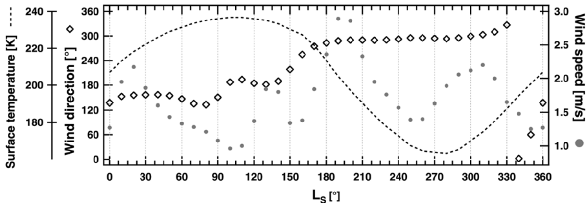
Figure 13.10.: Wind direction, wind speed, and surface temperatures over a full Martian year at the center of the study area at 82.5^{\circ}\text{E} and 45^{\circ}\text{N} . During the period of the highest surface temperatures (early summer; L_s \approx 100-110^{\circ} ), when sublimation rates are expected to be at their maximum, the wind comes from south to SSW (azimuth 180-195^{\circ} ). This is exactly parallel to the dominant crack orientation (e.g., figures 13.4a-c). An increased energy transfer into N-S-trending cracks might cause enhanced sublimation and degradation of their walls (data were derived from a General Circulation Model available at http://www-mars.lmd.jussieu.fr (e.g., Forget et al., 1999 ) and were kindly provided by Francois Forget and Ehouarn Millour).
