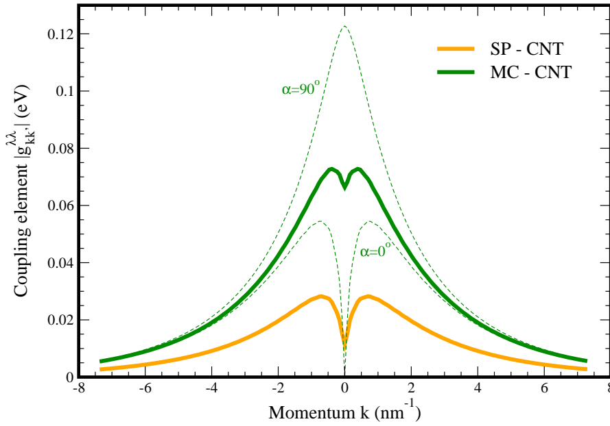
Figure 3. Absolute value of the intraband exciton-dipole coupling element g_{kk'=0}^{\lambda\lambda} as a function of the momentum transfer k for spiropyran- (SP-CNT) and merocyanine-functionalized carbon nanotube (MC-CNT). The dipole moment d and the dipole orientation \alpha (with respect to the CNT axis) are calculated in ab-initio calculations yielding d_{MC-CNT} = 9.7 D, \alpha_{MC-CNT} = 10.8^\circ and d_{SP-CNT} = 5.0 D, \alpha_{SP-CNT} = 32.8^\circ . The dashed line shows the coupling element for the two limiting cases of the parallel ( \alpha = 0^\circ ) and the perpendicular ( \alpha = 90^\circ ) dipole orientation.
