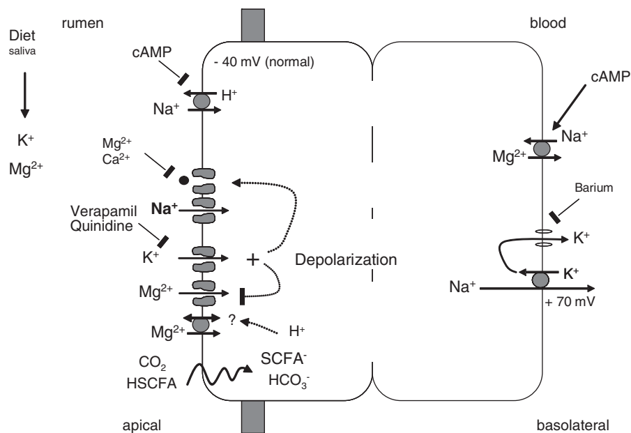
Figure 2 Model of ruminal K^+ and Mg^{2+} transport. Ruminants ingest large amounts of potassium with the diet (approximately 12 mol/day in cows). Both dietary intake and salivary flow contribute to the influx of K^+ into the rumen, which can accumulate to reach levels of 100 mmol/l in sodium-depleted animals. Both apical uptake and basolateral efflux of K^+ is mediated by channels, and accordingly, transport of K^+ across the rumen is passive and follows the electrochemical gradient. Transport is highest when the concentration gradient is high and drops when the transruminal potential rises. At low concentrations in the rumen, apical uptake of Mg^{2+} follows the electrochemical gradient across the apical membrane and is thought to occur via a channel. At higher concentrations, a second, transporter mediated pathway contributes to the total uptake. This pathway is stimulated by short chain fatty acids and CO_2 . Basolaterally, efflux of Mg^{2+} occurs coupled to the influx of Na^+ via a pathway that can be stimulated by cAMP. The channel-mediated uptakes of Na^+ , K^+ and Mg^{2+} are driven by potential and interact with each other in a complex fashion. Normally, the inside of the ruminal epithelium is negative v. the rumen. As the concentration of Mg^{2+} in the cell is similar to that of the rumen, this potential is essential to drive the uptake of this element into the epithelium. When ruminal K^+ rises, the potential difference across the apical membrane drops and the channel mediated uptake of Mg^{2+} is reduced. The pore of these channels is now free for the passage of Na^+ into the cytosol, driven by the concentration gradient, which is maintained by the basolateral Na^+ pump. The rising electrogenic transport of Na^+ will raise transruminal potential and thus, limit the efflux of K^+ from the rumen.
