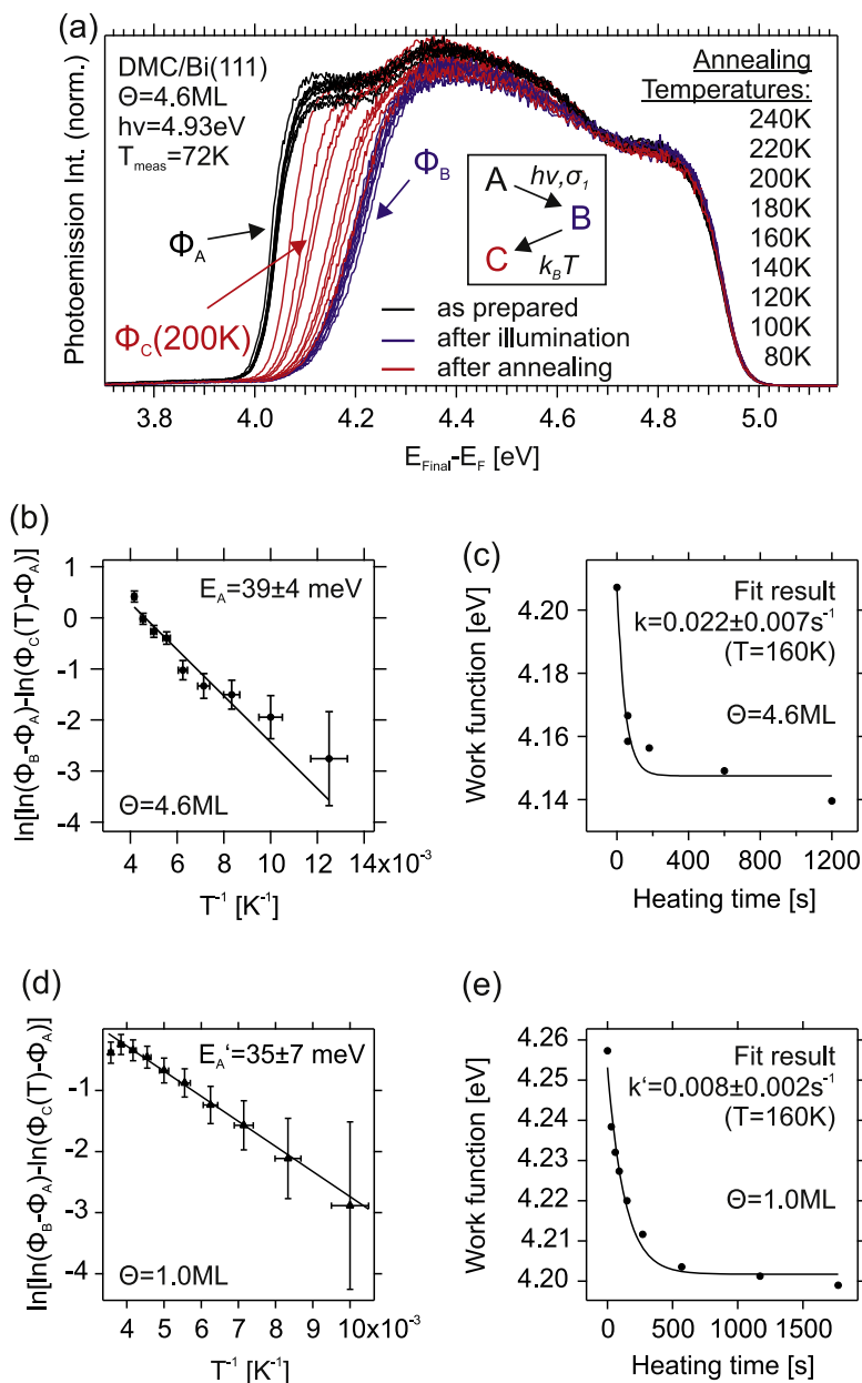
Figure 6. (a) Photoemission spectra of multilayer DMC after deposition (black), after illumination (blue) and after subsequent heating to a specific temperature (red, 5 min). All spectra were recorded at a sample temperature of 72 K. The inset schematically shows the involved reactions of DMC. (b) Arrhenius plot for the thermal reaction in the multilayer, resulting from the series shown in (a). A measure for the changes of the work function (see text for details) is plotted over the inverse annealing temperature. (c) Work function change as a function of annealing time at 160 K. A fit according to equation (2) yields the rate constant at this temperature. (d) Arrhenius plot analogous to (b) but for a DMC coverage of 1.0 ML. (e) Determination of the rate constant at 160 K for a coverage of 1.0 ML, in analogy to (c).
