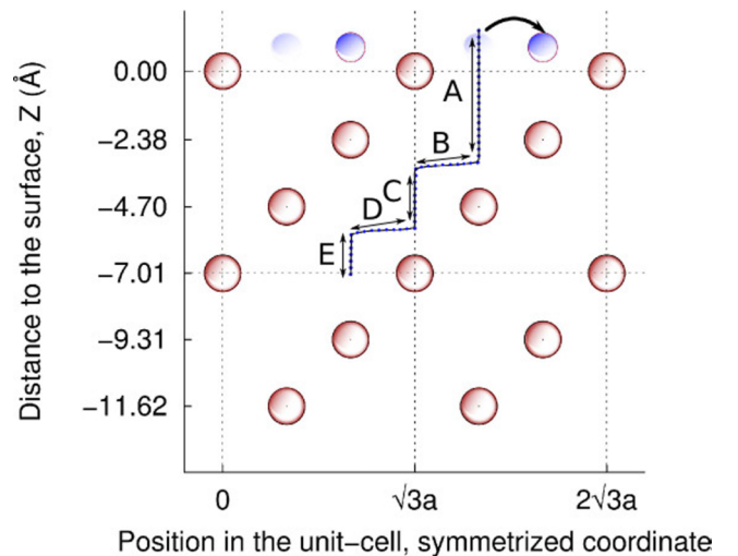
FIG. 1. Sketch of the staircase-shaped one-dimensional pathway for resurfacing of H atoms from bulk-like positions ( b , at z_H \sim 5.6 \text{ \AA} ) to the surface through the fcc hollow. In the case of a fcc - \Theta = 1 covered surface, the curved arrow indicates that the H-adsorbate is displaced to the hcp site by the repulsive interaction with the emerging atom.
