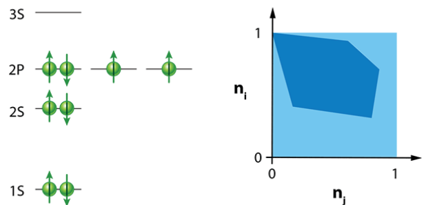
FIG. 1: (Left) The electronic configuration of an atom (oxygen is shown here) is based on Pauli's exclusion principle. (Right) A schematic showing that the generalized Pauli constraints restrict the natural occupation numbers n_i, n_j to the dark-blue polygon, significantly strengthening Pauli's exclusion principle (light-blue square). (APS/Alan Stonebraker; Image of polytope on homepage Wikimedia Commons/Maxim Razin)
