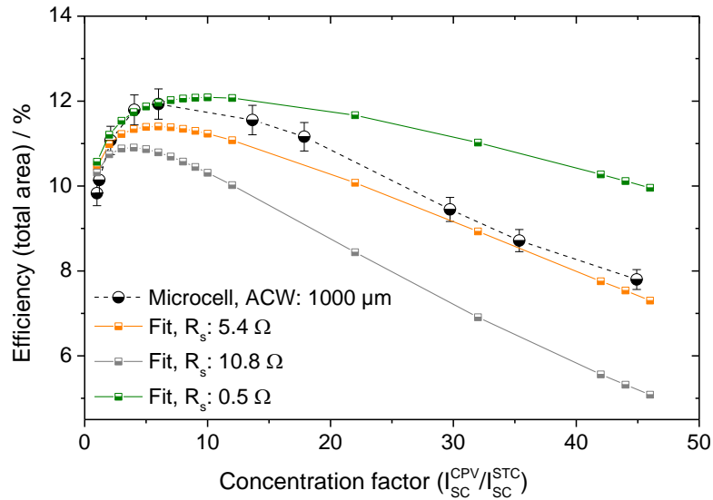
Figure 7: Simulation of the conversion efficiency based on the FF -model introduced in chapter 1.1 and 4.3. Experimental raw data of a lamellar microcell with 1000 \mu\text{m} ACW were used for the initial setup.
