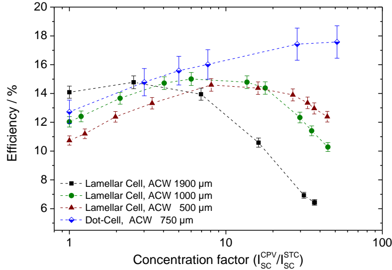
Figure 5: Plot of the active area based conversion efficiency of lamellar cells out of series C and of a 750 \mu m sized dot-shaped cell against the light concentration factor (log-plot). All efficiencies were corrected to 298.1 K.
