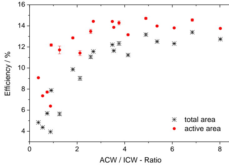
Figure 3: Plot of total and active area based conversion efficiencies of lamellar microcells against their geometrical ratio between active cell width (ACW) and interconnection zone width (ICW).
