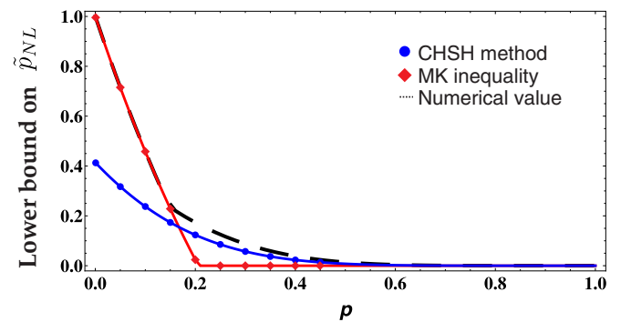
FIG. 1. (Color online) Lower bounds on the local content of the GHZ state under parallel dephasing, for N = 3 . (Red) The bound obtained from the MK inequality [38]; (blue) the new bound (19) from the CHSH method; and (black dashed) the value obtained through a numerical optimization described in the main text. For p > 0.18 , the nonlocal content is better described by the bound from the CHSH method.
