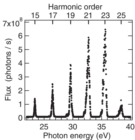
FIG. 3. A high-order harmonic spectrum generated in argon at 110 mbar by a 1.5 mJ, 40 fs pulse with a center wavelength of 785 nm. The spectrum was measured by recording the current from an XUV sensitive photodiode just before the sample position while scanning the monochromator grating. The slit size of the entrance and exit slits was adjusted for a monochromator resolution of 210 meV at harmonic 23. The FWHM bandwidth of harmonic 23 is 500 meV.
