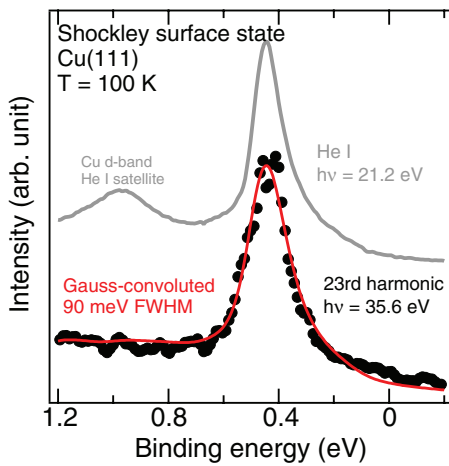
FIG. 4. Photoelectron spectra of the Cu(111) surface state at 100 K measured with the He I \alpha line at 21.2 eV photon energy (top) and with high-order harmonic radiation at 35.6 eV (bottom) with identical analyzer settings. The broad peak at \approx 1.0 eV binding energy stems from the Cu d-band excited with the He-I satellite. The He I \alpha data are limited by the analyzer resolution. The solid red line is a convolution of these data with a Gaussian (with the satellite removed), which gives an energy bandwidth of 90 meV (FWHM) for the high-order harmonic radiation.
