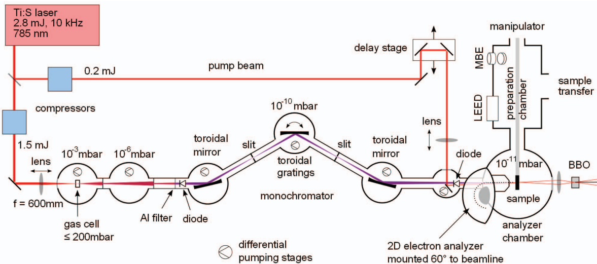
FIG. 2. Layout of the IR-pump – XUV-probe tr-ARPES experiment. Approximately 90% of the Ti:S laser output is used for HHG, while the remaining 10% is used for pumping the sample. Both beam paths have their own computer-controlled compressors for pulse duration control and a \lambda/2 -plate + polarizer combination for power control. HHG occurs in the gas cell, typically in Ar. XUV sensitive photodiodes are located just after the Al filter and after the second toroidal mirror. The IR pump beam is introduced into the beamline after the second toroidal mirror. A BBO crystal behind the analyzer chamber is used to find the temporal overlap of the pump pulse and an IR pulse allowed to pass through the beamline.
