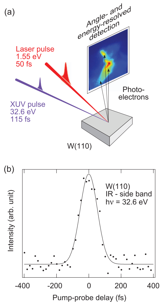
FIG. 5. (a) IR pump – XUV probe arrangement for tr-ARPES. The IR and XUV beams impinge on the sample with a small angle between them in the horizontal plane, which forms an angle of 60^\circ to the surface normal. Photoelectrons are detected along the surface normal. (b) Cross-correlation measurement between 50 fs IR and XUV at 32.6 eV. The monochromator was set to 150 meV photon-energy resolution. The vertical axis shows the population of electrons lifted transiently above the Fermi level of the W(110) crystal by side-band formation. It gives a cross-correlation of the IR and XUV pulses, which is fitted to a Gaussian of FWHM 125 fs (solid red line). Deconvolution from the IR pulse yields an XUV pulse duration of \approx 115 fs FWHM.
