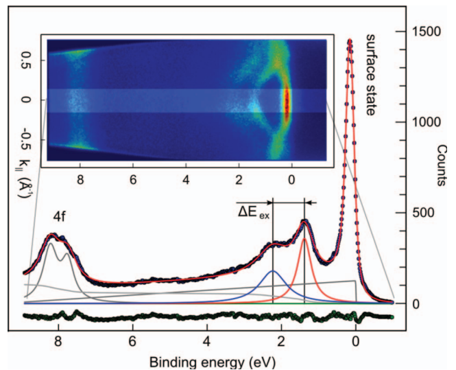
FIG. 6. Photoemission spectrum from a 10 nm thick Gd(0001) film on a W(110) substrate. The inset shows an ARPES image recorded for 5 min at one pump-probe delay using the 23rd harmonic at 35.6 eV. A photoelectron spectrum (blue points) is extracted by integrating over the highlighted stripe around k_{\parallel} = 0 . This is then repeated for all pump-probe delays. The energy bandwidth of the XUV was 150 meV. The electron analyzer, set to wide angle mode ( \pm 13^\circ acceptance angle) at a pass energy of 60 eV and an entrance-slit width of 0.5 mm, has a calculated energy resolution of 150 meV FWHM. The upper limit of the total energy resolution is given by the 260 meV FWHM of the Gd surface state. The individual components used to fit the data (solid lines) are explained in the text.
