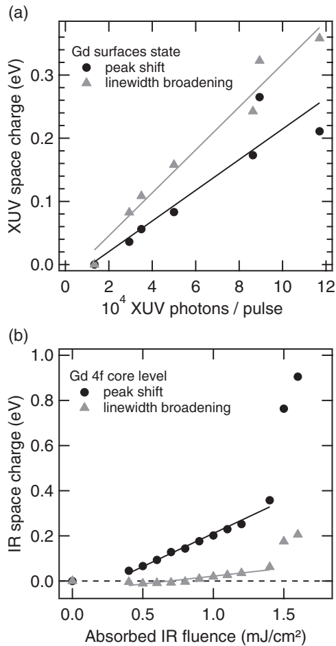
FIG. 9. Space-charge shift (circles) and broadening (triangles) of the spectra as measured from changes to the Gd(0001) surface state and the Gd 4f core level, (a) shows the probe pulse space charge of the harmonic radiation, (b) the pump-probe delay dependent contribution of the IR pump pulse, here at 4 ps pump-probe delay where it reaches a maximum.
