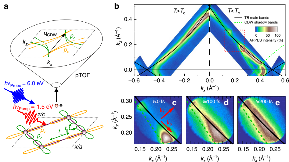
Figure 1 | Time-dependent Fermi surface map. (a) Experimental scheme and TB model. The Te-5p x/2 orbitals in the Te-layers of \text{RTe}_3 (bottom) are coupled by t_{||} and t_{\perp} describing interactions parallel and perpendicular to the Te chains and lead to a diamond-shaped Fermi surface in reciprocal space, which we access by our position-sensitive time-of-flight photoelectron spectrometer (pTOF) (top). Nesting leads to shadow bands translated along \mathbf{q}_{\text{CDW}} (dashed lines). (b) Static FS of \text{HoTe}_3 for T = 300 \text{ K} > T_c (left) and T = 180 \text{ K} < T_c (right). Main and shadow TB bands are indicated by solid and dashed lines, respectively. In the CDW phase, energy gaps open on the Fermi surface where main and shadow bands overlap. The red square indicates the region investigated in panels (c–e). (c–e) Time-dependent FS of \text{DyTe}_3 for various pump-probe delays at T < T_c . The gapped FS transforms within 200 fs into a continuous, metallic state. Arrows in c indicate directions perpendicular ( k_1 ) and parallel ( k_2 ) to the FS, respectively. The weak intensity in the upper left corner in c stems from a partially twinned crystal domain.
