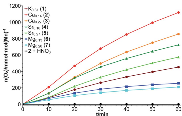
Fig. 6 Traces for \text{O}_2 evolution from experiments on water-oxidation-catalysis by different M-birnessites. Oxides 1–7 (1 mg \text{mL}^{-1} ) were suspended in solutions of \text{Ce}^{\text{IV}} (0.25 M) and filled into septum vials. The progress of the reaction was then analysed by headspace gas chromatography to detect and quantify the \text{O}_2 product. No oxygen evolution could be detected for suspensions of oxides 1–7 in \text{HNO}_3 (pH \sim 1.7 ), as shown for 2 + \text{HNO}_3 as an example (black trace).
