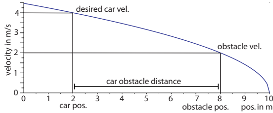
Fig. 7. Velocity function over position. The resulting car velocity is calculated from the current car position, the followed car's position and the followed car's velocity.
