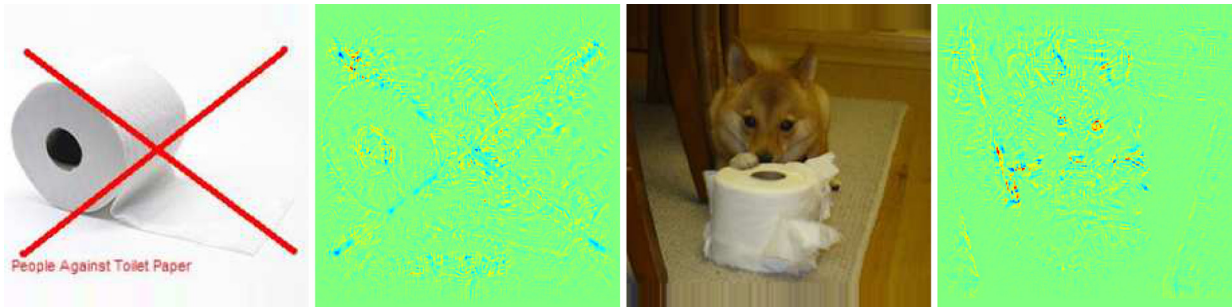
Fig 26. Failure examples for the pixel-wise decomposition. Left and Right: Failures to recognize toilet paper. The decompositions computed by Formula (58) with stabilizers \epsilon = 0.01 The neural net is the pre-trained one on ILSVRC data from the Caffe package [60]. The computing methods for each column are the same as in Fig 25 . Pictures in order of appearance from Wikimedia Commons by authors Robinhood of the Burger World and Taro the Shiba Inu.
