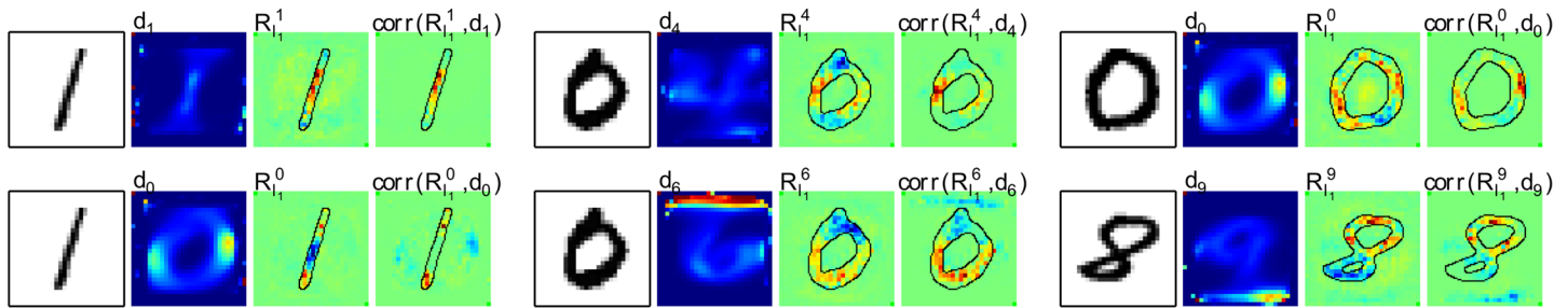
Fig 13. Each quadruple shows: on the leftmost the input digit; on the middle left the class specific pixel-wise density ratios d_k (Eq (65)) for the digit class k for which the pixel-wise decomposition is computed; on the middle right the pixel-wise decomposition R_i^{(1)} for that digit and the digit class k ; on the rightmost the correlation between d_k and the pixel-wise decomposition R_i^{(1)} . When considering a digit from class i and a pixel-wise decomposition from class k \neq i , it is observable that the pixel-wise decomposition shows frequently highly positive activations on pixels of the digit from class i which have high relative density d_k for the digit class k \neq i .
