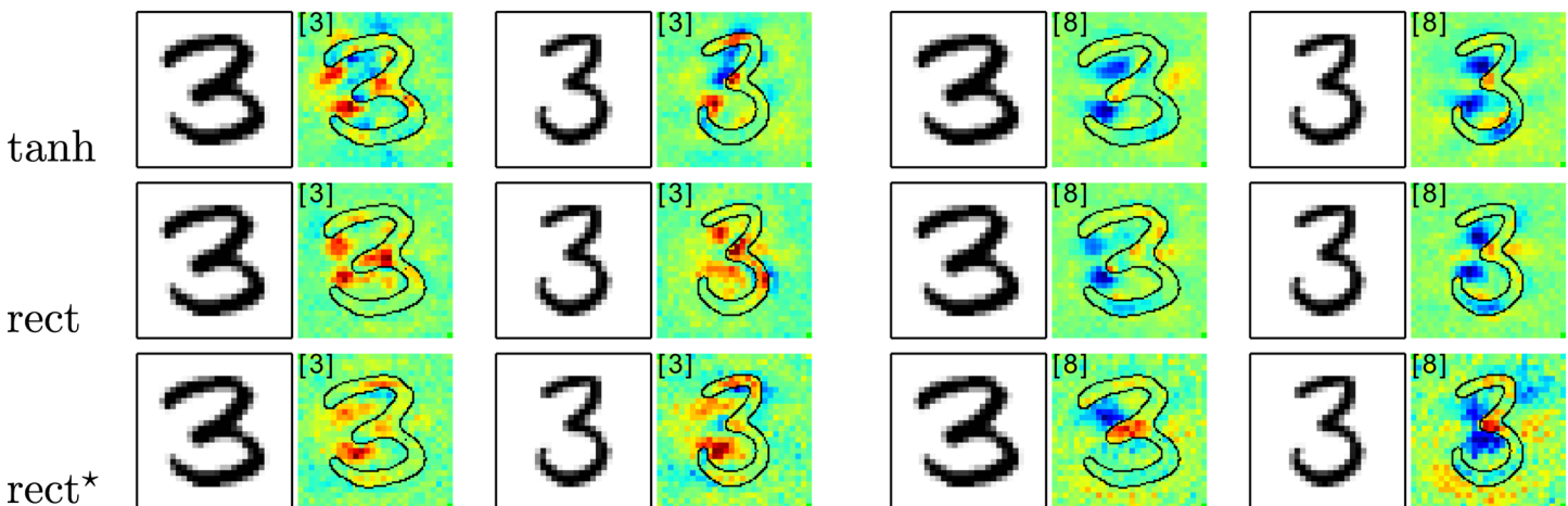
Fig 16. Evidence for a handwritten digit being a “3” or a “8”. Classifying as “3” is supported by the middle horizontal stroke featured in this digit and the absence of vertical connections on the left of the image. Evidence for being a “8” feature again the middle horizontal stroke, however, the absence of connections on the left side of the digit constitutes negative evidence. Explanations are again stable for various models and samples.
