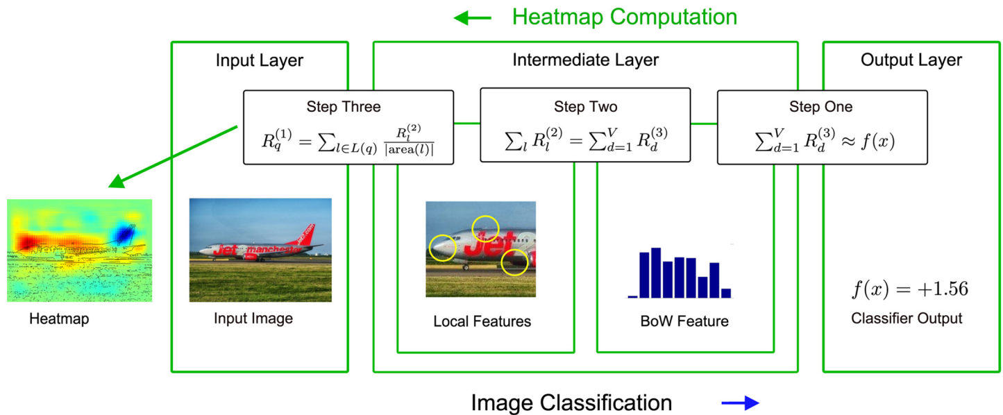
Fig 4. Local and global predictions for input images are obtained by following a series of steps through the classification- and pixel-wise decomposition pipelines. Each step taken towards the final pixel-wise decomposition has a complementing analogue within the Bag of Words classification pipeline. The calculations used during the pixel-wise decomposition process make use of information extracted by those corresponding analogues. Airplane image in the graphic by Pixabay user tpsdave.
