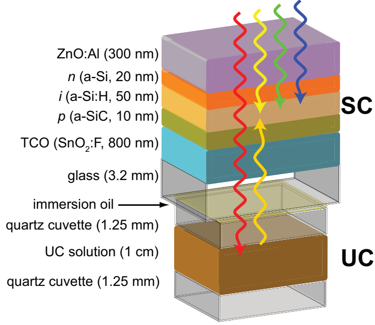
FIG. 3. A cartoon of the integrated a-Si:H p - i - n /UC device. Low energy (shown in red) photons pass through the p - i - n structure and excite dye molecules in the upconversion unit, which subsequently returns photons of a shorter wavelength (yellow).
