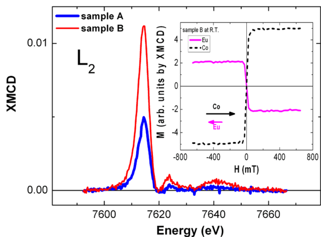
Figure 2 | Normalized XMCD spectra recorded at R.T. at the Eu L_{2} edge for samples A and B. Significant polarization of Eu in EuS is revealed. Inset: Element-specific magnetization curves by XMCD at R.T. for sample B. Eu is always antiferromagnetically oriented to Co.
