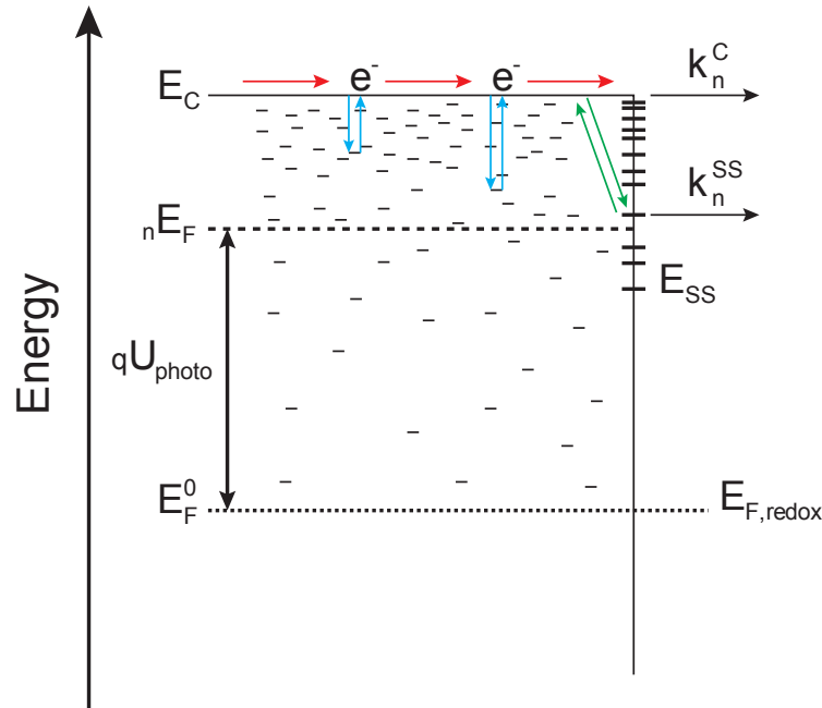
Figure 2.5: Scheme presenting the processes involved in the recombination between electrons in TiO 2 and the oxidized form of the redox couple. E_F^0 is the position of the Fermi level in the dark, equilibrated with the redox potential E_{F,redox}^0 . nE_F is the quasi Fermi level of electrons which defines the photovoltage U_{photo} . E_C is the conduction band energy and E_{SS} are surface states in the TiO 2 . The following processes can occur: Electron transport in the conduction band with rate k_n^C , trapping and release in localized states in the bulk of semiconductor nanoparticles, trapping and release by surface states, electron transfer through surface state with rate k_n^{SS} . Adapted from [146].
