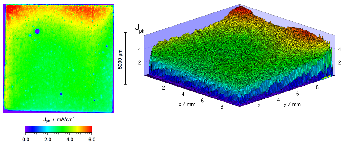
Figure 4.15: Spatially resolved photocurrent image of a NSCSC with an electrolyte film deposited from a 5 M LiI / 50 mM I 2 solution; step width: 40 μm; laser intensity: 130 mW/cm 2 ; spot diameter: 25 μm and average photocurrent density: \overline{J_{ph}} \approx 3.5 mA/cm 2 .
