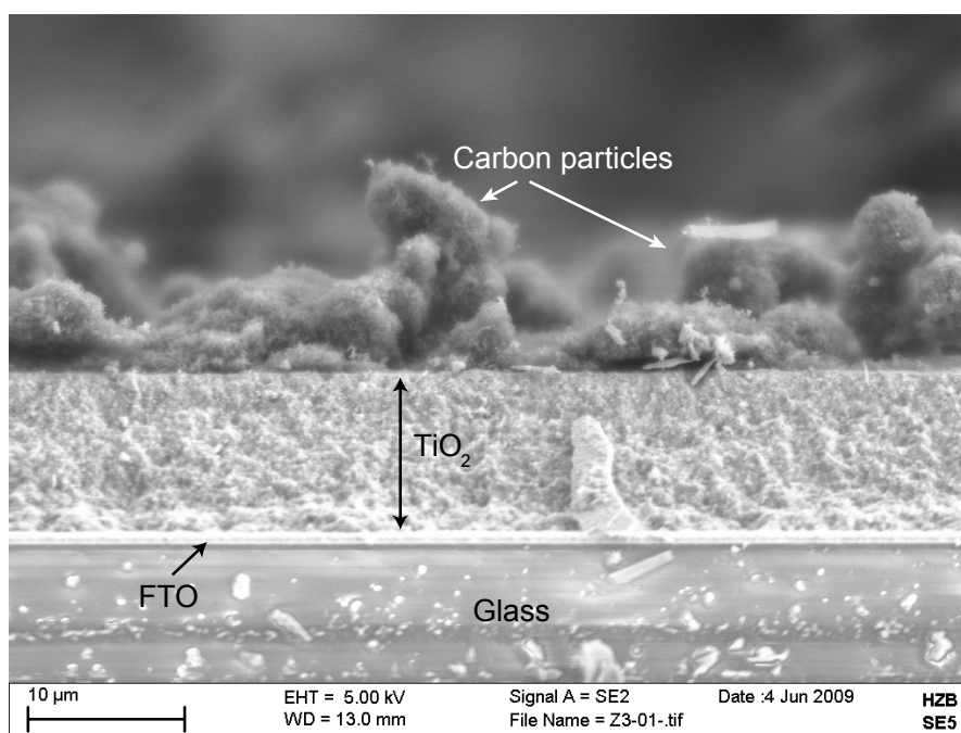
Figure 3.6: SEM image of a carbon layer on top of the screen-printed \text{TiO}_2 film.
