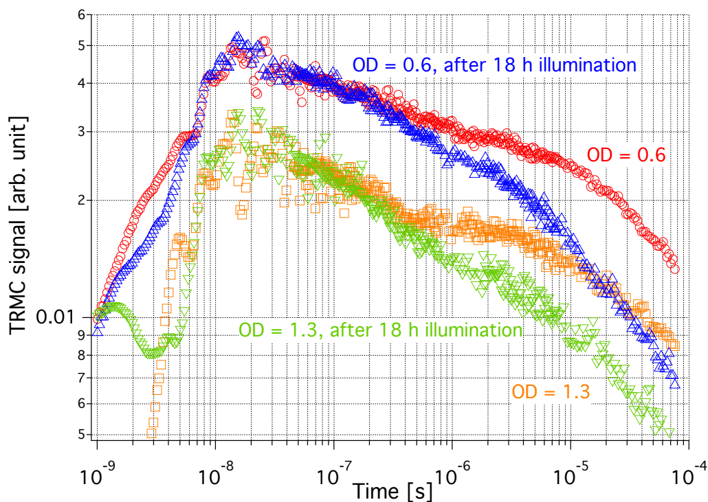
Figure 4.1: TRMC signals of a quasi-solid-state dye-sensitized solar cell in a double-logarithmic plot induced by laser pulses at 532 nm and excitation densities of 20 \text{ mJ/cm}^2 ( \text{OD} = 0.6 ) and 5 \text{ mJ/cm}^2 ( \text{OD} = 1.3 ).
