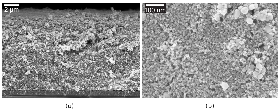
Figure 4.22: SEM cross section image of a screen-printed, mesoporous TiO 2 layer on FTO glass.
