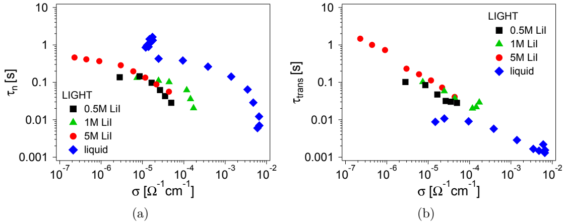
Figure 4.19: Effective electron lifetime \tau_n and transit time \tau_{trans} of electrons in \text{TiO}_2 for NSCSC with a different concentration of the redox couple in the electrolyte film and a liquid DSC, as indicated. The data is plotted versus the electron conductivity in the \text{TiO}_2 .
