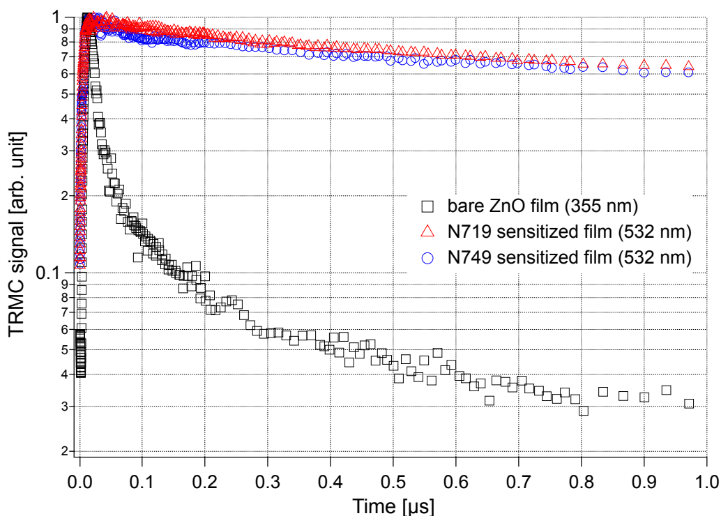
Figure 4.37: Normalized TRMC signals of bare and sensitized ZnO films induced by laser pulses at 355 and 532 nm. Sensitizers were the Ru-dyes N719 and N749 ("black dye"). Laser intensity: 0.6 mJ/cm 2 and 0.8 mJ/cm 2 , respectively.
