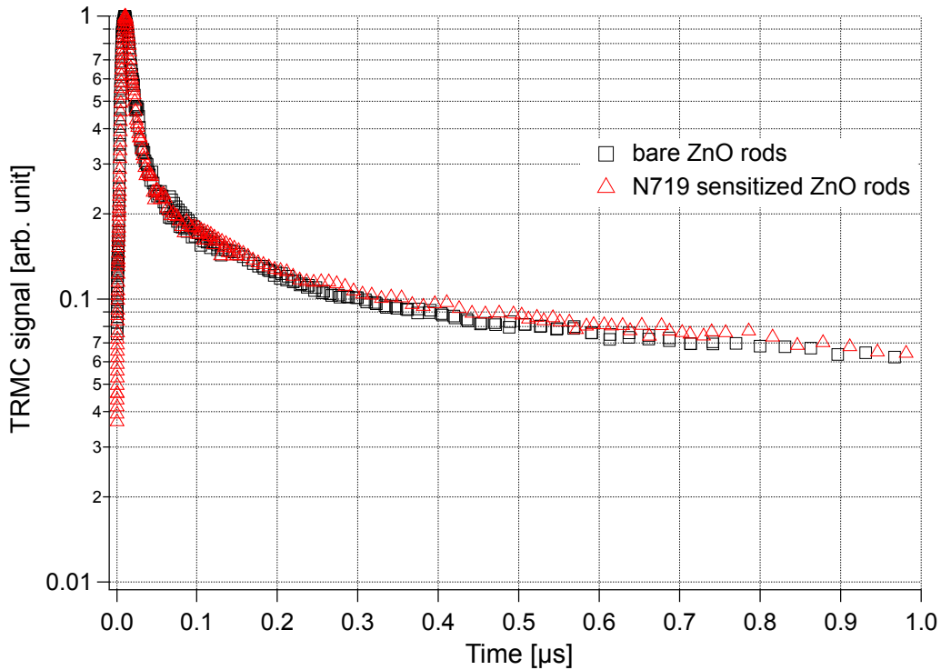
Figure 4.42: Normalized TRMC signals of bare and sensitized \text{ZnO} nanorods induced by laser pulses at 355 nm. Laser intensity: 140 \mu\text{J}/\text{cm}^2 .
