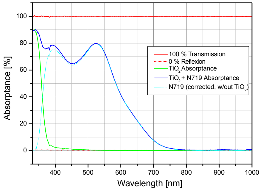
Figure 3.5: UV/Vis absorbance spectrum of the N719 dye on a TiO 2 layer.
