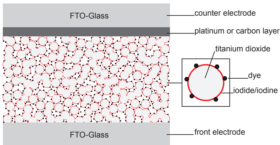
Figure 2.3: Scheme outlining the cell concept of a quasi-solid-state Nano Surface Conductivity Solar Cell (NSCSC). The mesoporous TiO 2 layer is covered by a film of iodide/iodine in a supersaturated state acting as the hole transporting medium towards the counter electrode. No additional solvent is present and the cell is in equilibrium with the ambient atmosphere.
