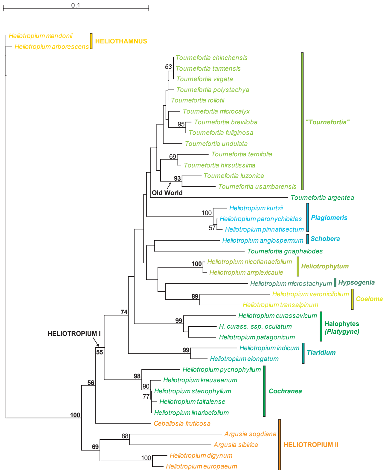
Fig. 6-6. (b) Neighbor-joining tree of the analyzed species of the HELIOTROPIUM I clade. Important clades are indicated. The numbers above the branches are bootstrap percentages (1000 replicates, percentages <50% are not shown, scale bar 10% distance).
