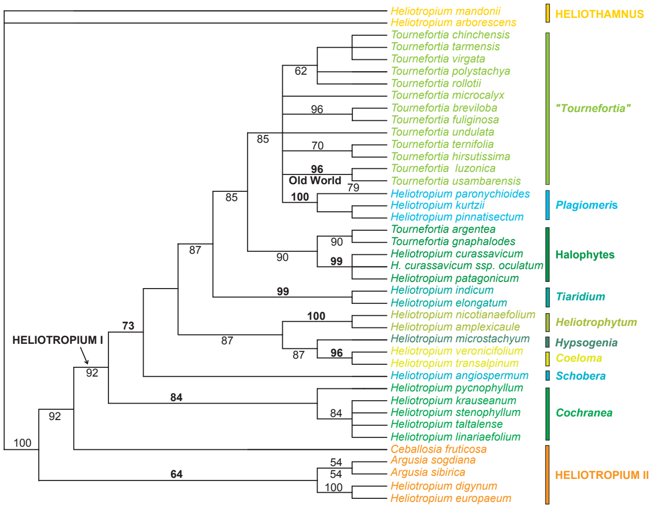
Fig. 6-6. (a) Majority-rule consensus tree, computed from the 4,317 most parsimonious trees of the ITS1 dataset ( l=460 steps, CI=0.724 , RI=0.743 , HI=0.276 ). Important clades are indicated. The numbers above the branches are bootstrap percentages. Percentages <50\% are not shown. The numbers below the branches are majority percentages <100\% .
