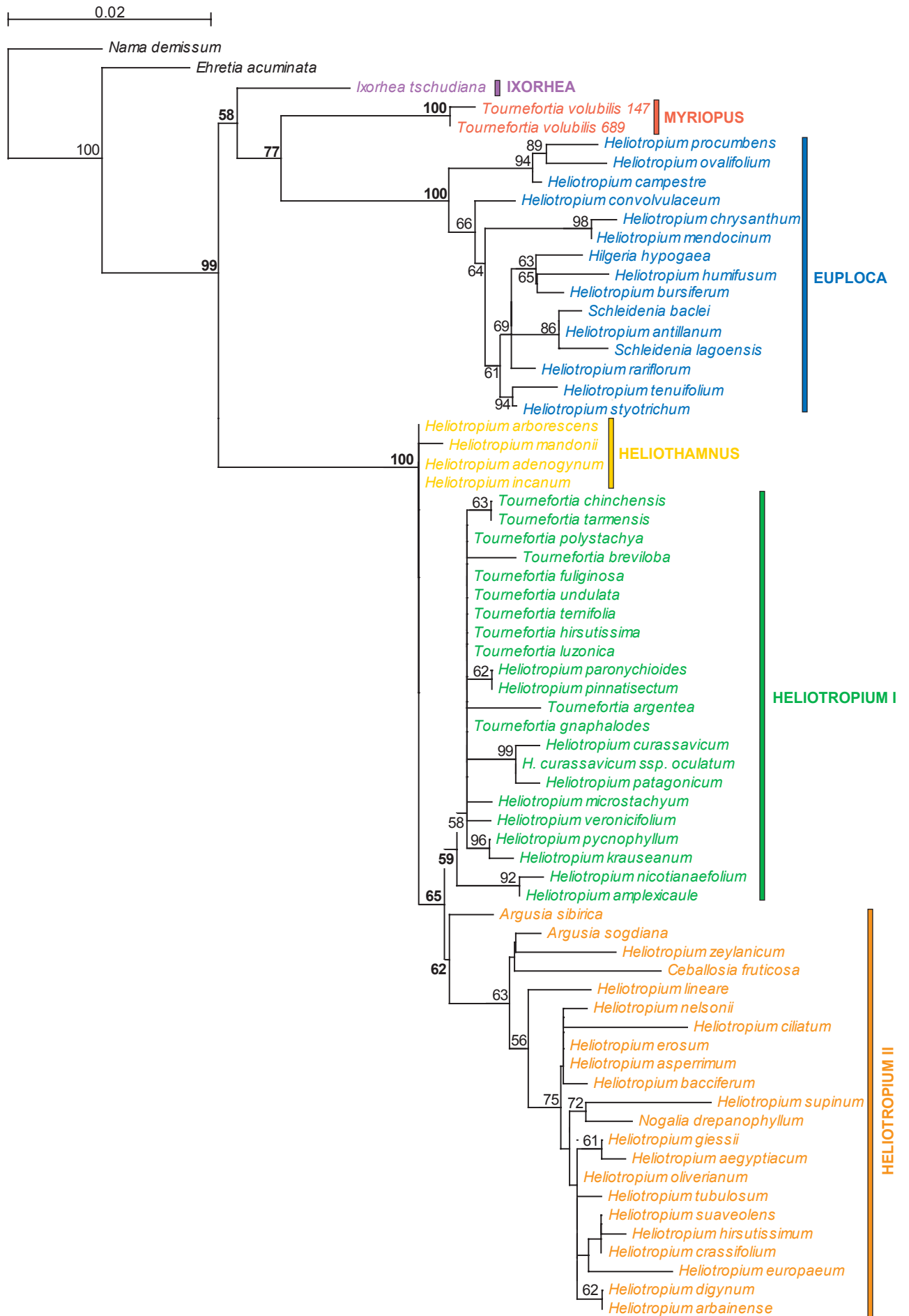
Fig. 6-2. Neighbor-joining tree of the analyzed species of Heliotropiaceae of the trnL dataset. Important clades are indicated. The numbers above the branches are bootstrap percentages (1000 replicates, percentages <50% are not shown, scale bar 2% distance).
