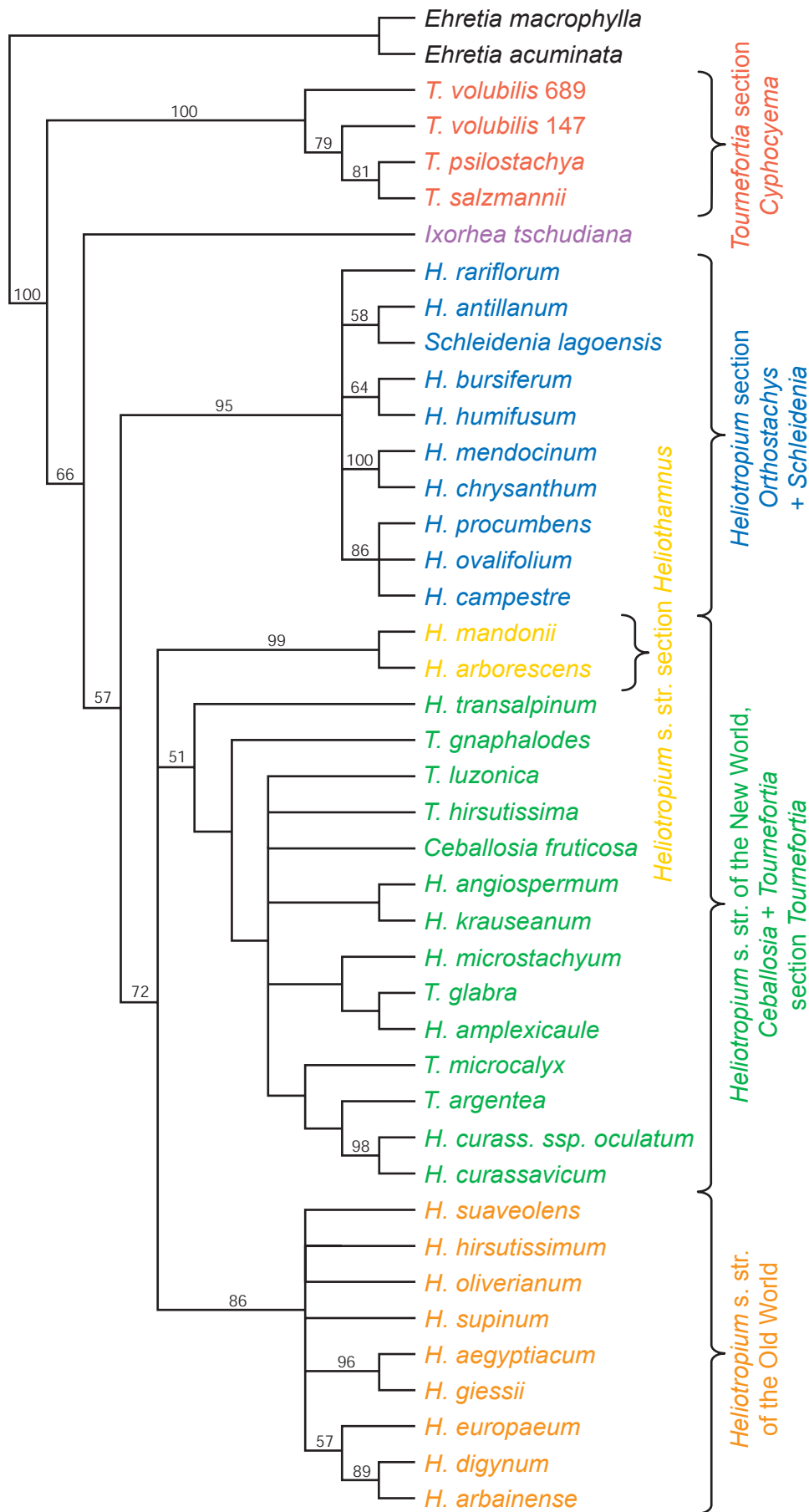
Fig. 2-1. Strict consensus tree of the analyzed species of Heliotropiaceae, computed from the 426 most parsimonious trees (L [tree length] = 460, CI [consistency index] = 0.60, RI [retention index] = 0.75). Important taxa are indicated. The numbers above the branches are bootstrap percentages. Percentages under 50% are not shown.
