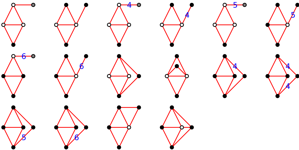
Figure A.3: Graphs constructed from K_4 - e .
