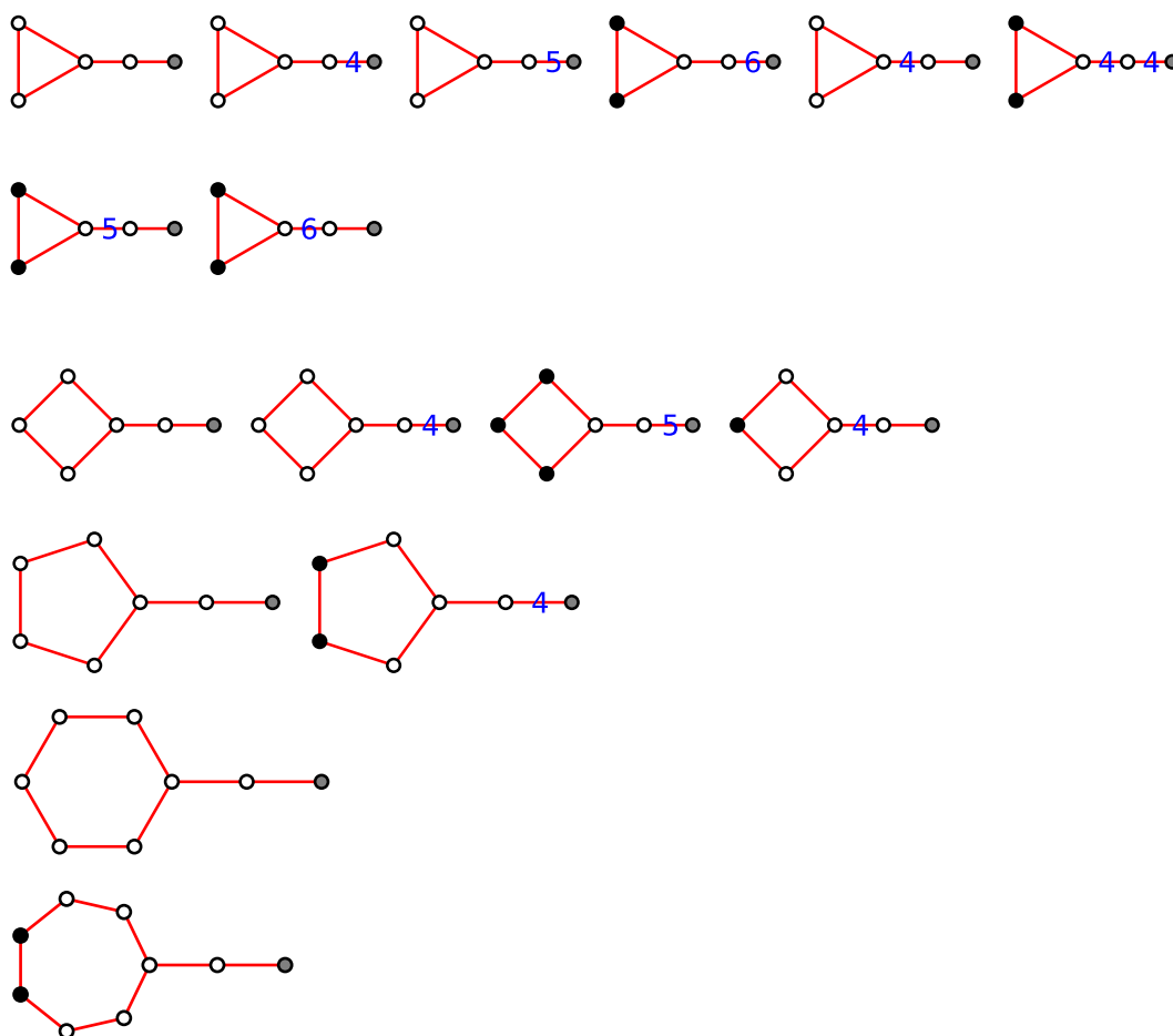
Figure A.9: Cycles with one tail of length 2.
