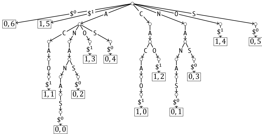
Figure 2.4: Generalized suffix trie of the string collection S = \{ANANAS\$^0, CACAO\$^1\} .
