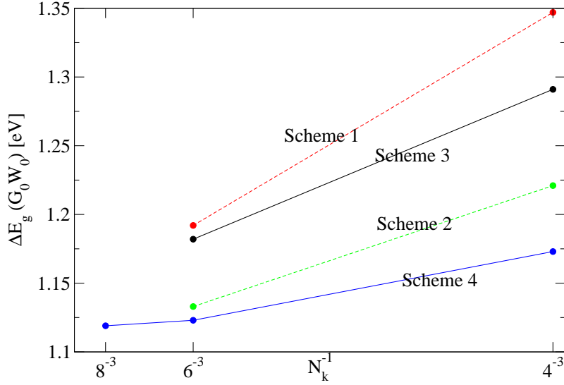
Figure 6.6: Convergence of the G_0W_0 correction to the fundamental band gap with respect to N_{\mathbf{k}}^{-1} in GaAs using different schemes. Same as what we found in Si, using the same mesh for everything gives the best convergence behavior.
