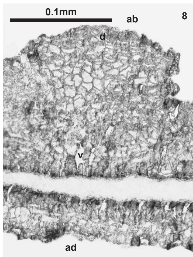
Figures 7-6 to 7-8: † Ehretia hedericarpa . 7-6: Variability of the fossils examined; left row: abaxial view; right row: adaxial view; red arrows: submarginal furrow. 7-7: Transverse sections of an endocarpid at different levels; red arrow: position of the submarginal furrow. 7-8: Transverse section of a single abaxial ridge with cellular pattern. ab: abaxial; ad: adaxial; d: dorsal; v: ventral.
