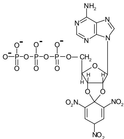
TNP-ATP
