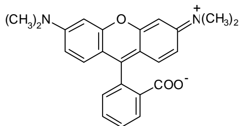
Tetramethylrhodamine
