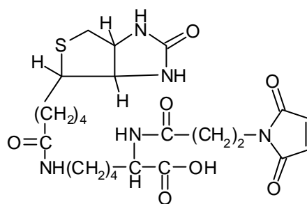
Biocytin-maleimide
