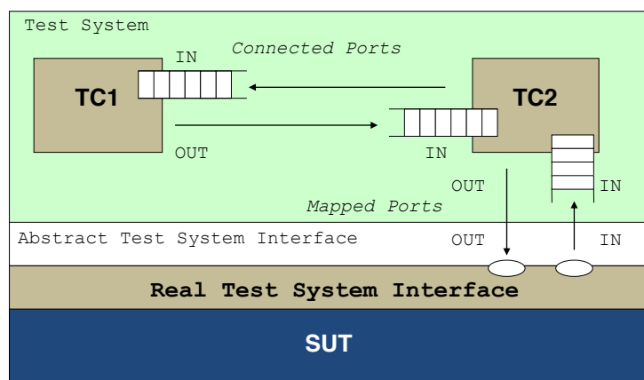
FIGURE 3.1: Conceptual View Of A TTCN-3 TS [2]
