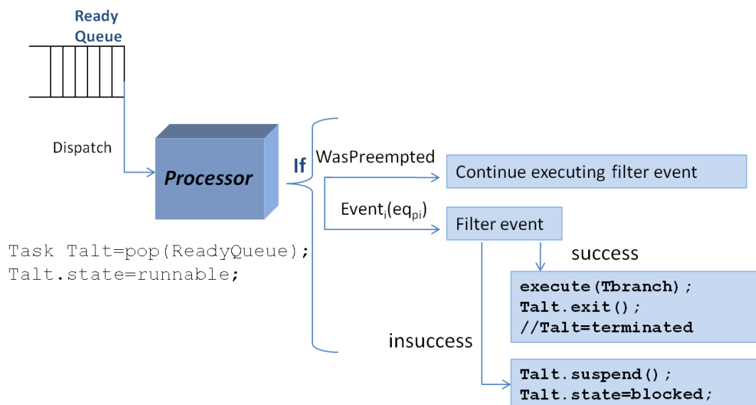
FIGURE 5.13: Behavior Of Alt Task When Running [6]
