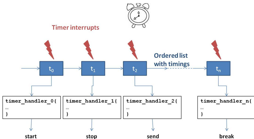
FIGURE 5.5: Generating Timer Event [6]
