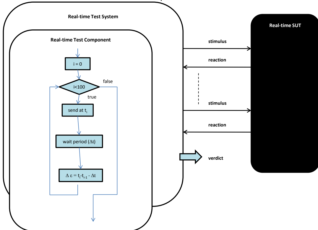
FIGURE 7.9: Test System For Evaluating The send Operations With Strict Timings
