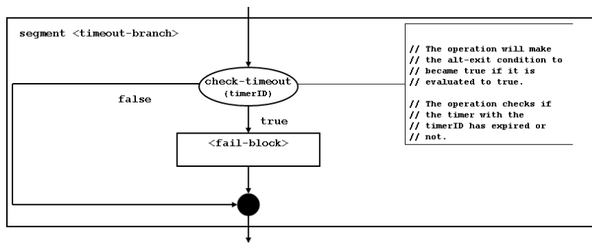
FIGURE 4.22: Flow Graph Segment For A Timeout Branch Of An \langle \text{alt-stmt} \rangle Statement [5], [4]
