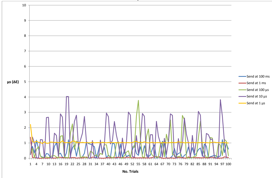
FIGURE 7.10: Latency Margins For The send Operation With Strict Timing
