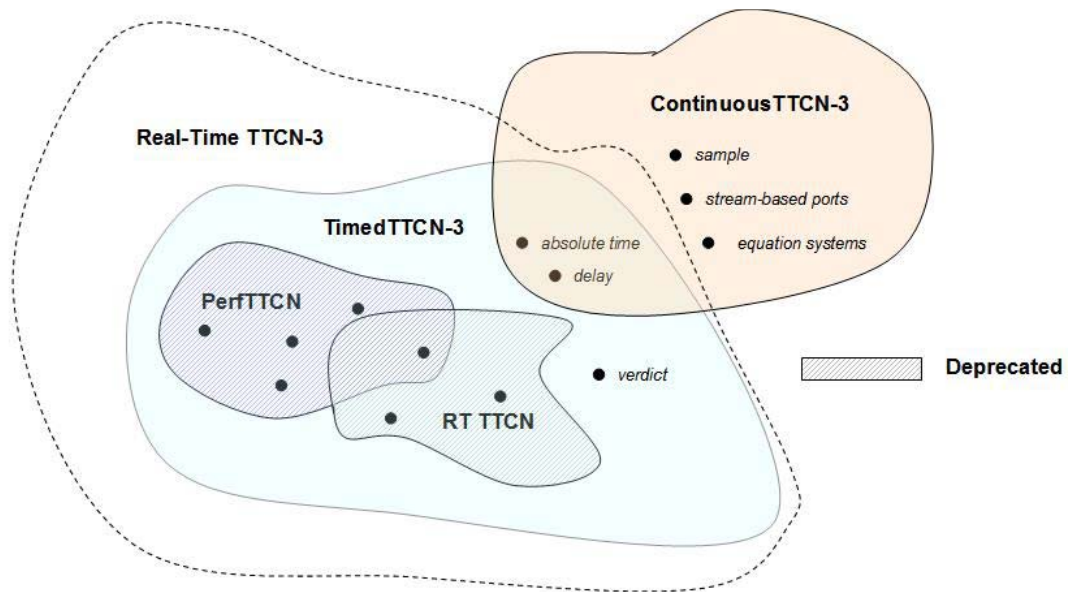
FIGURE 3.3: TTCN-3 Overview Of Proposed Extensions [3]
