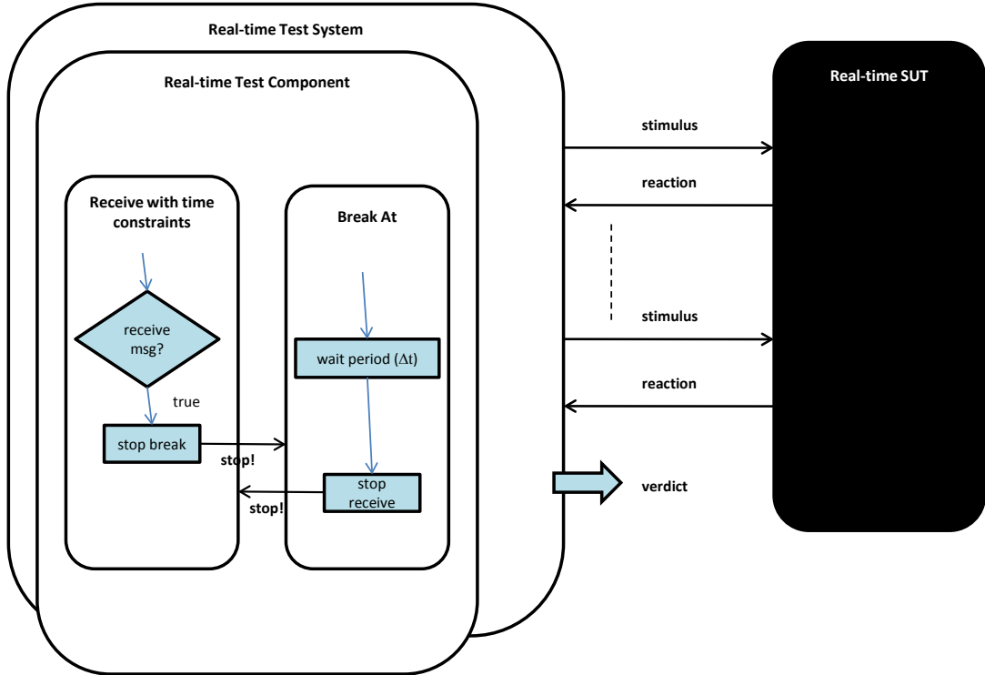
FIGURE 7.14: Test System Structure For receive...break Evaluation
