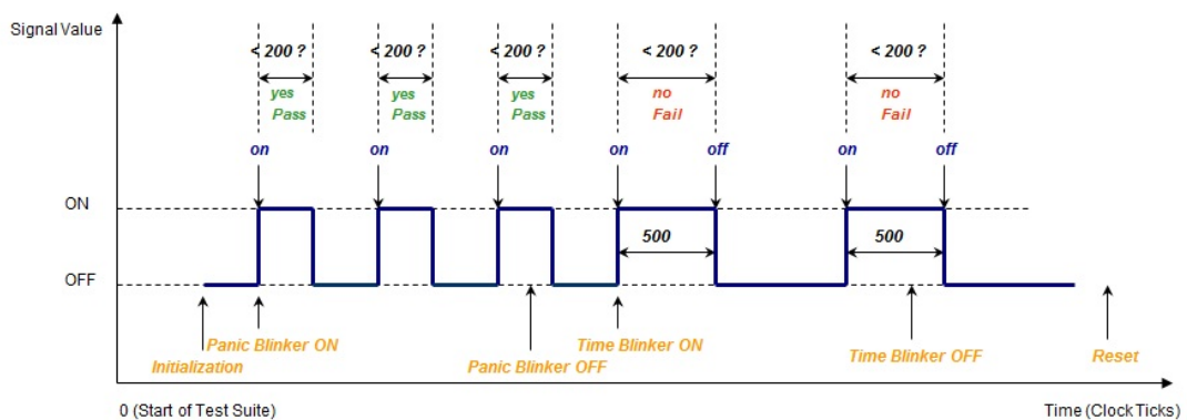
FIGURE 7.19: Another Possible Flash Light Signal Flow
