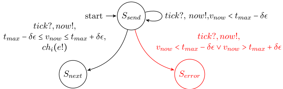
FIGURE 4.14: Timer For send State With Time Constraint.
