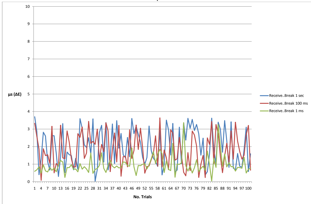
FIGURE 7.15: Latency Margins For The break Instruction
