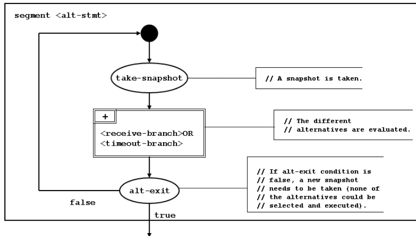
FIGURE 4.20: Flow Graph Segment For <alt-stmt> Statement [5], [4]
