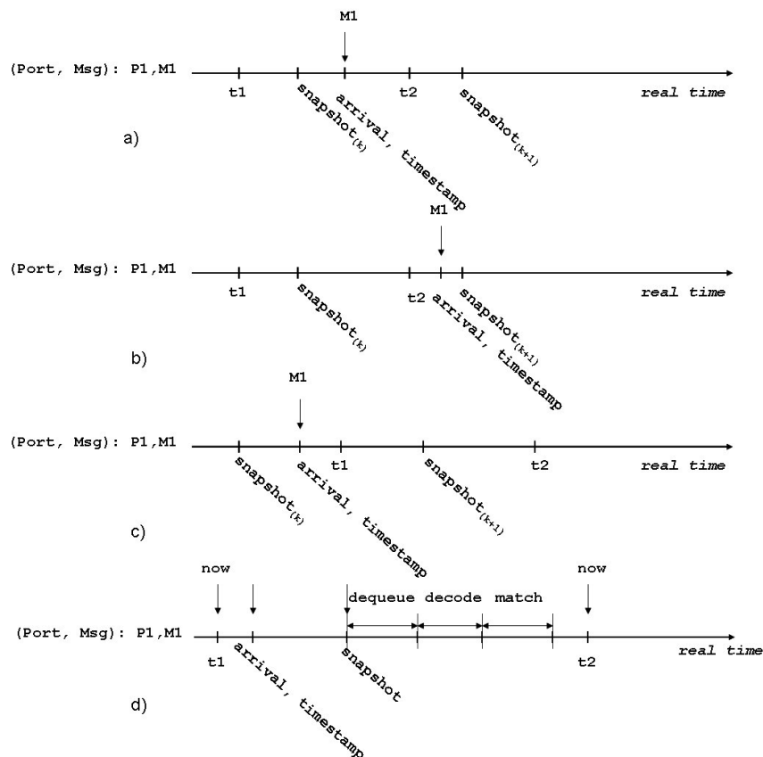
FIGURE 4.23: Events And Operations Over Time [4]
