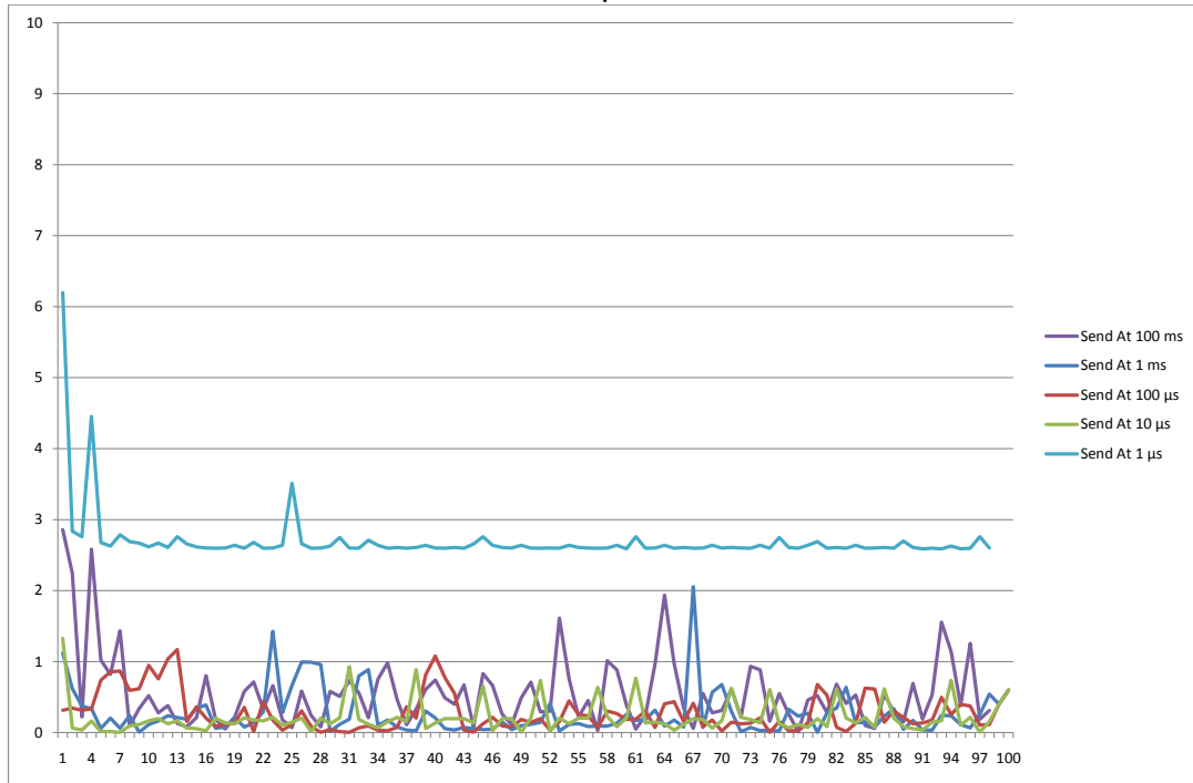
FIGURE 7.11: Latency Margins For The send Operation For The Implementation Using Timers
