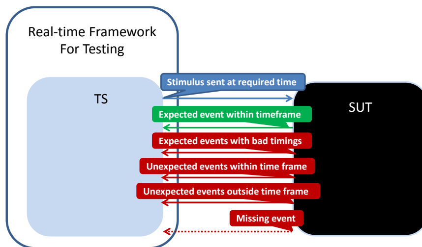
FIGURE 2.2: Black-box Testing For A Real-time System
