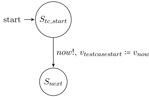
FIGURE 4.6: Testcasestart.
