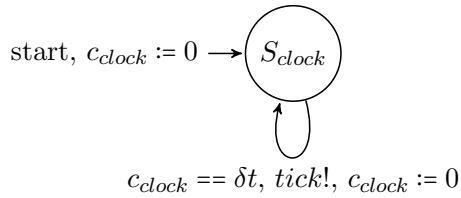
FIGURE 4.3: Logical Clock.
