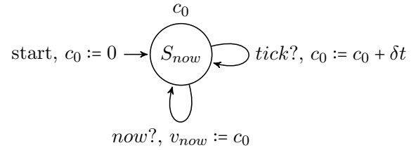
FIGURE 4.4: Now State.
