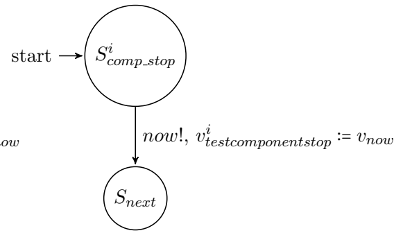
FIGURE 4.8: Testcomponentstop.
