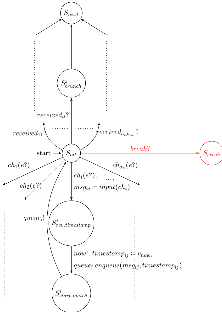
FIGURE 4.15: alt Automaton.
