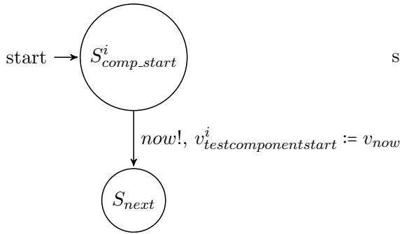
FIGURE 4.7: Testcomponentstart.
