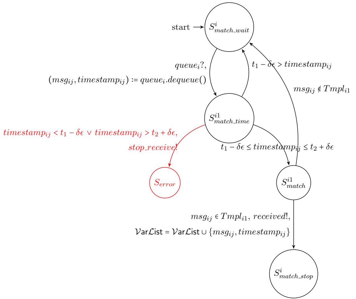
FIGURE 4.13: Match automaton.
