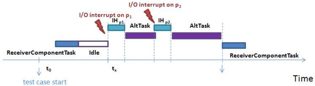
FIGURE 5.16: (a) Possible Flow Of Events [6]
