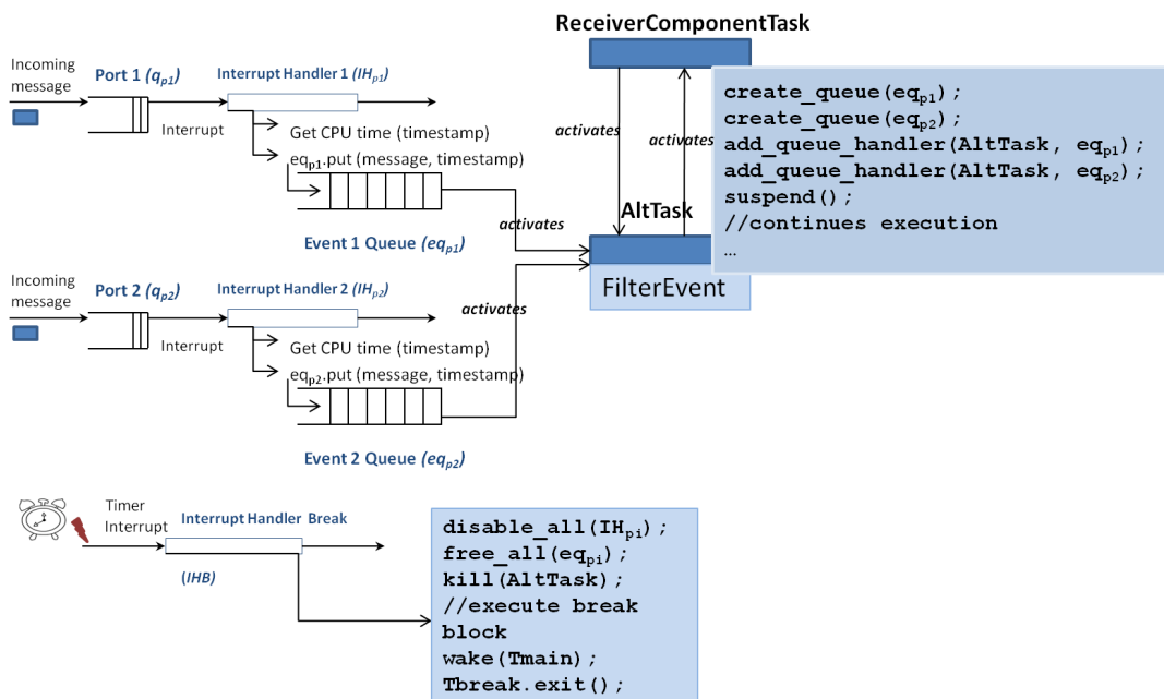
FIGURE 5.15: Task Interactions For An Alt Statement [6]
