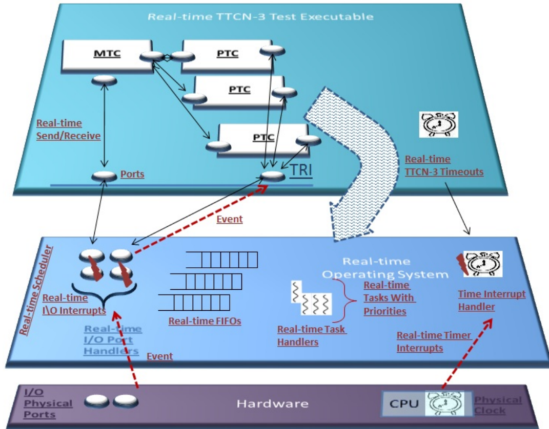
FIGURE 5.4: Implementation Design For A Real-time TTCN-3 Platform
