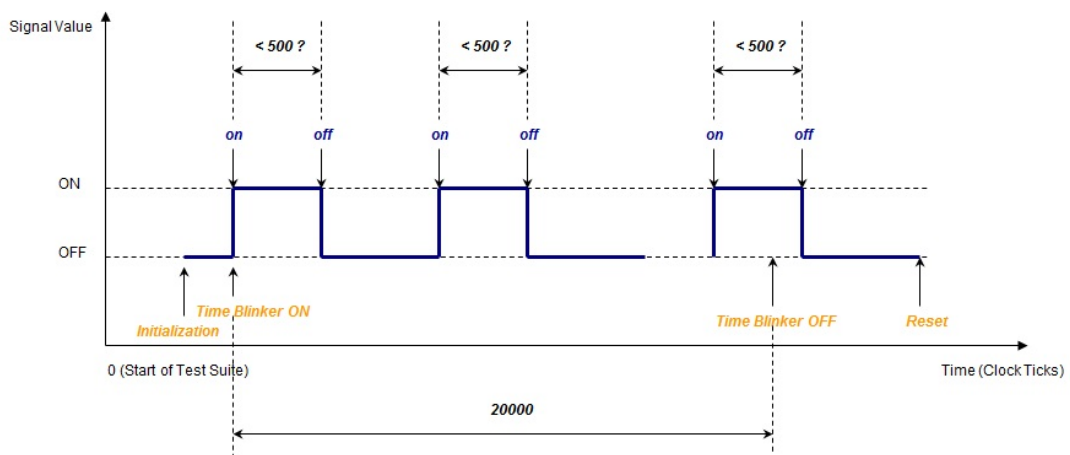
FIGURE 7.17: One Possible Flash Light Signal Flow
