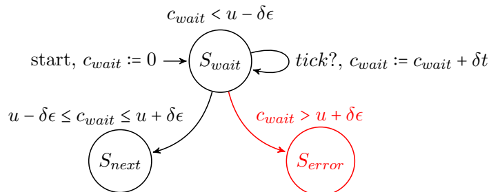
FIGURE 4.5: Wait State.
