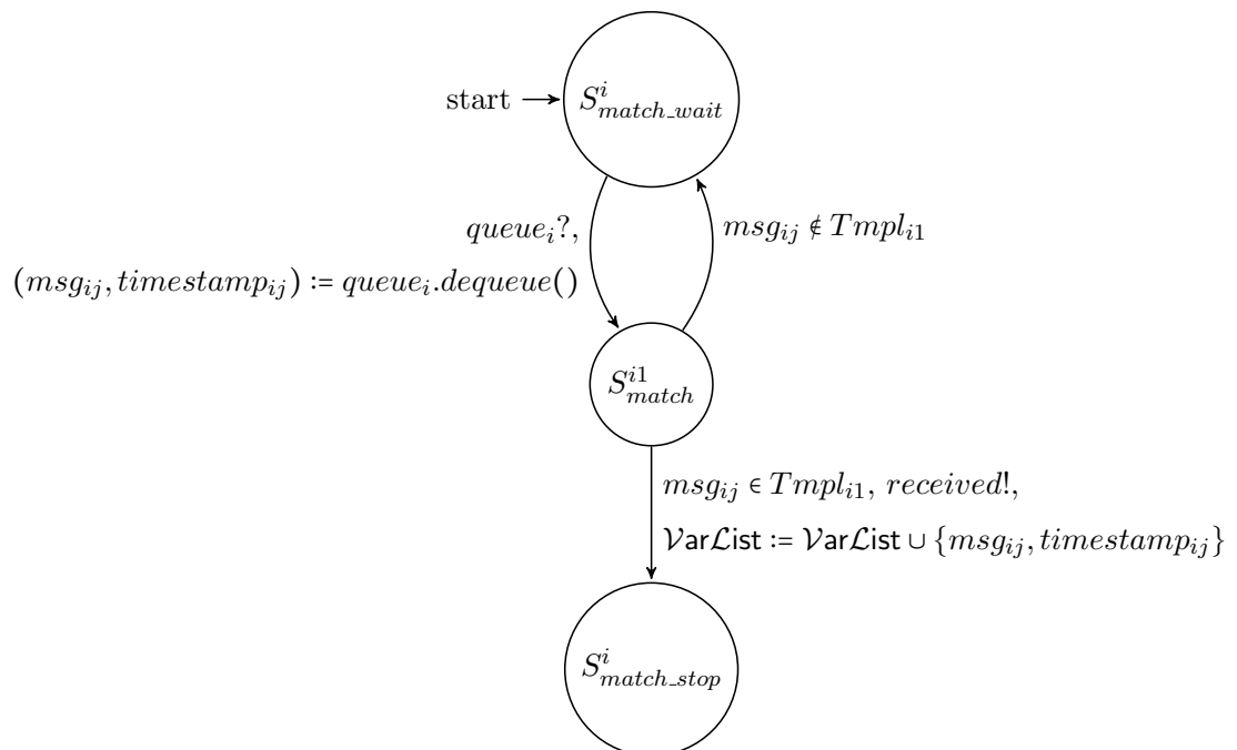
FIGURE 4.10: Match Automaton.
