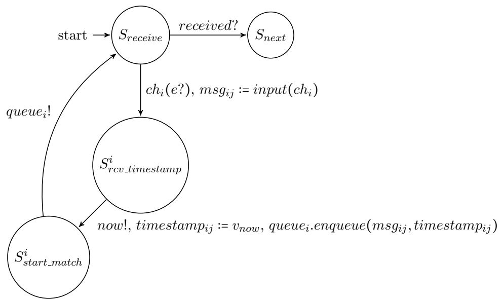
FIGURE 4.9: Receive Automaton.
