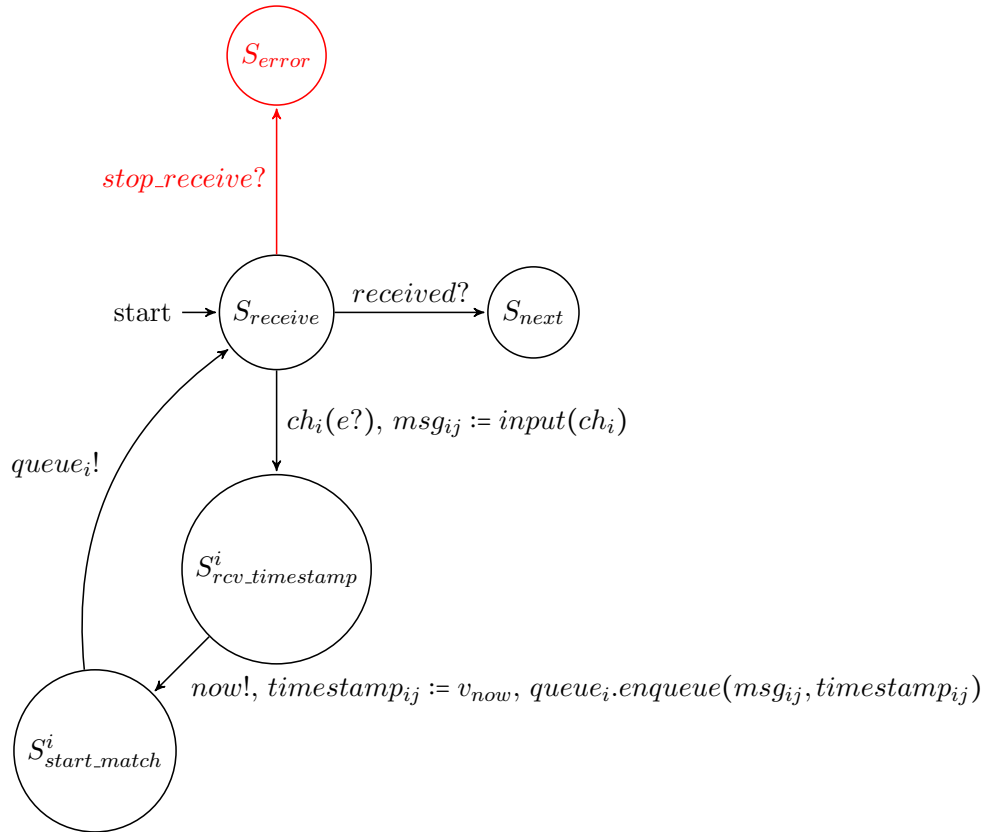
FIGURE 4.12: Receive automaton.
