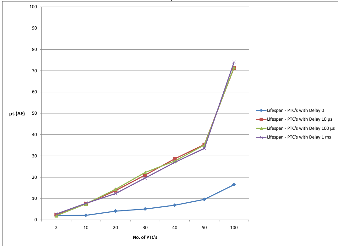
FIGURE 7.8: Latency Margins For The Lifespan Of PTC's, With An Increased Numbers Of PTC's And Variable Delays
