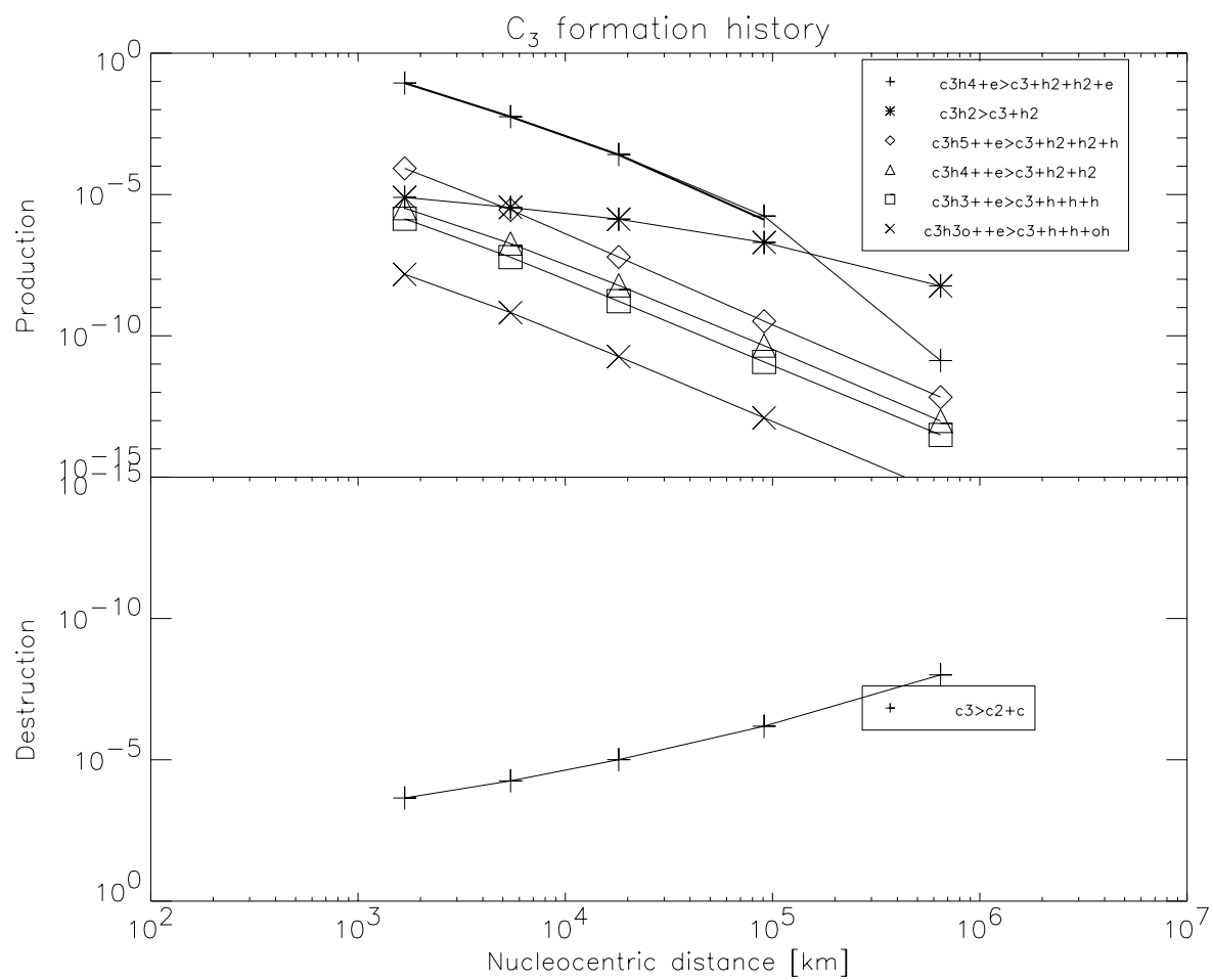
Figure D.13: C_3 formation at 4.74 AU
