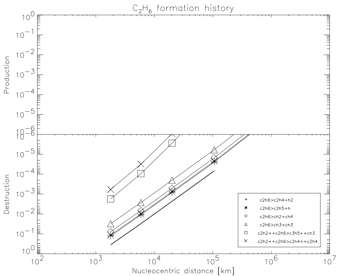
Figure D.5: C_2H_6 formation at 3.78 AU
