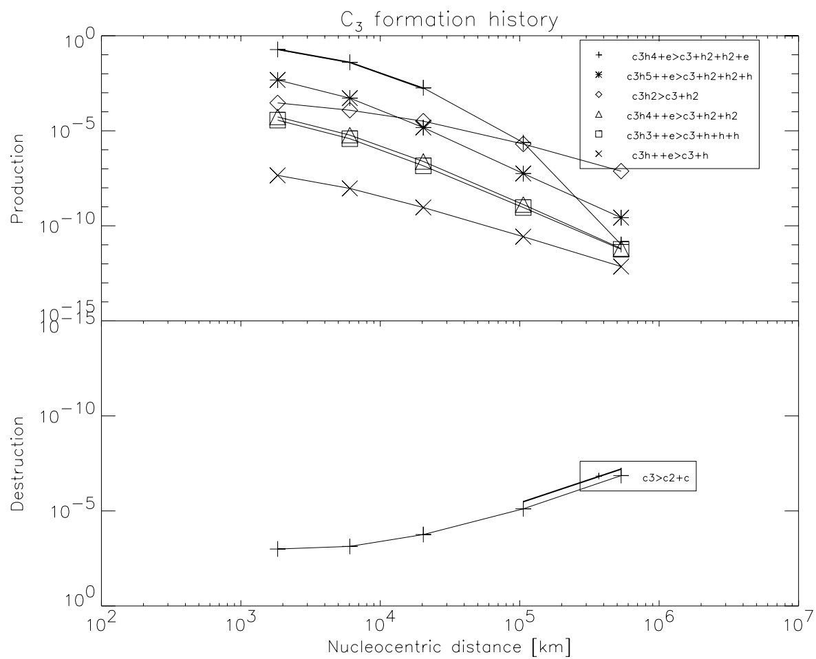
Figure D.11: C_3 formation at 2.86 AU
