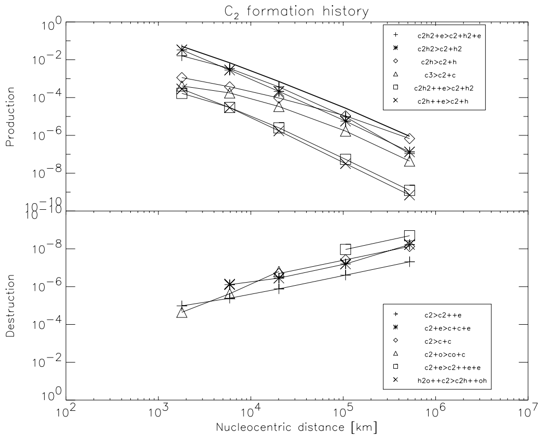
Figure D.1: C_2 formation at 3.78 AU
