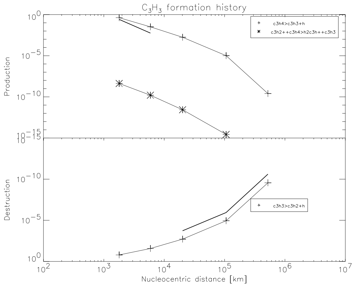
Figure D.8: C_3H_3 formation at 3.78 AU
