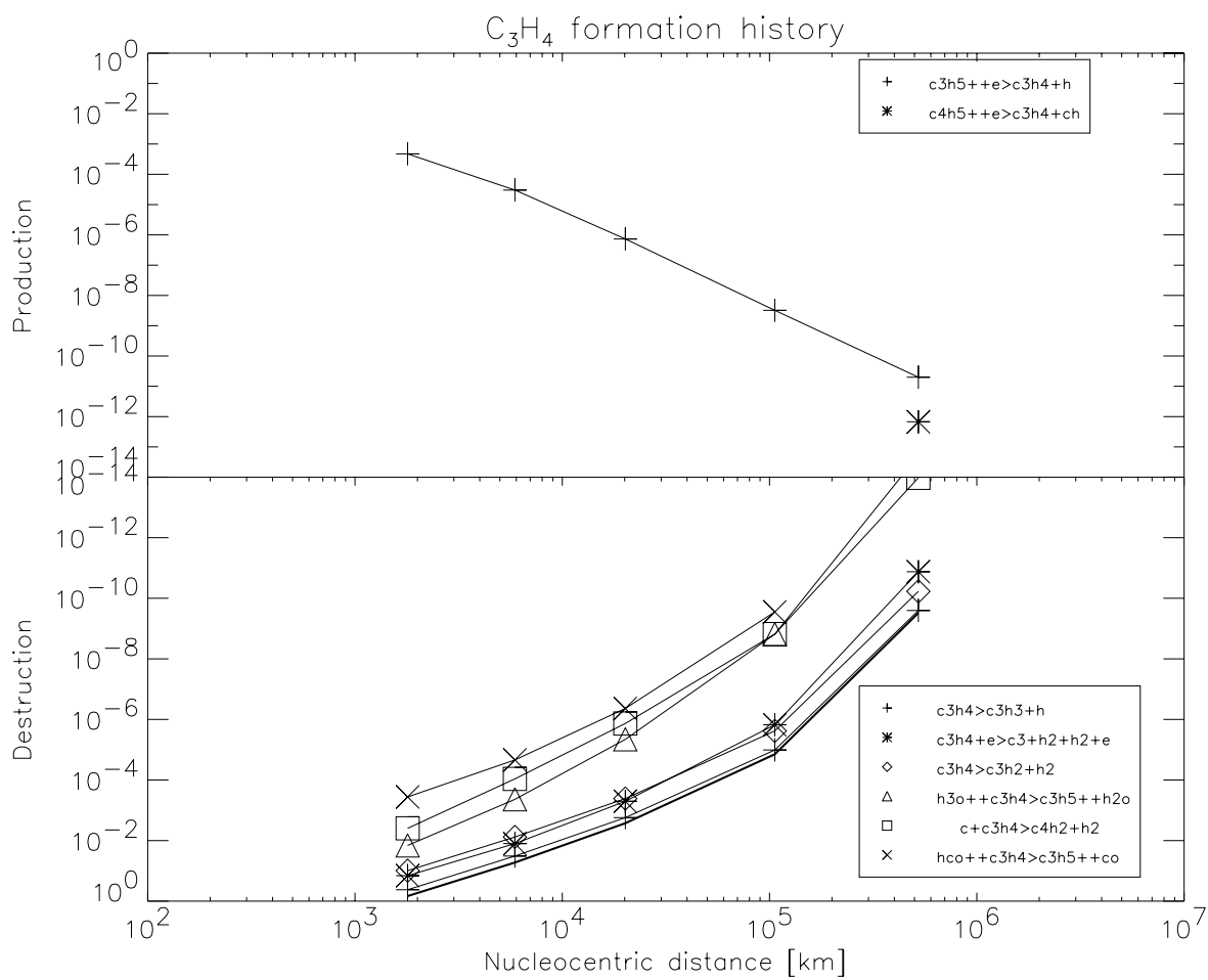
Figure D.9: C_3H_4 formation at 3.78 AU
