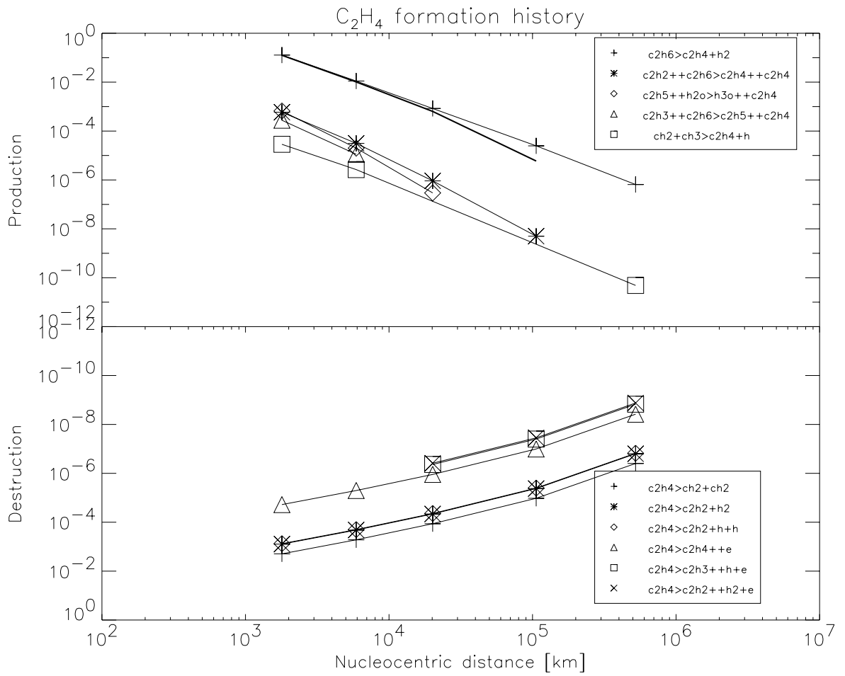
Figure D.4: C_2H_4 formation at 3.78 AU
