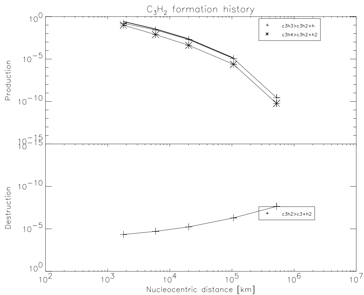
Figure D.7: C_3H_2 formation at 3.78 AU
