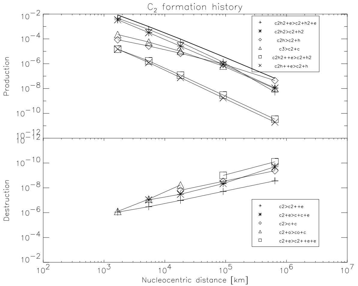
Figure D.12: C_2 formation at 4.74 AU
