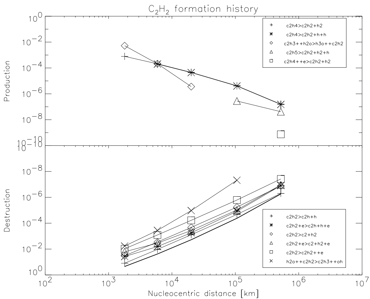
Figure D.3: C_2H_2 formation at 3.78 AU
