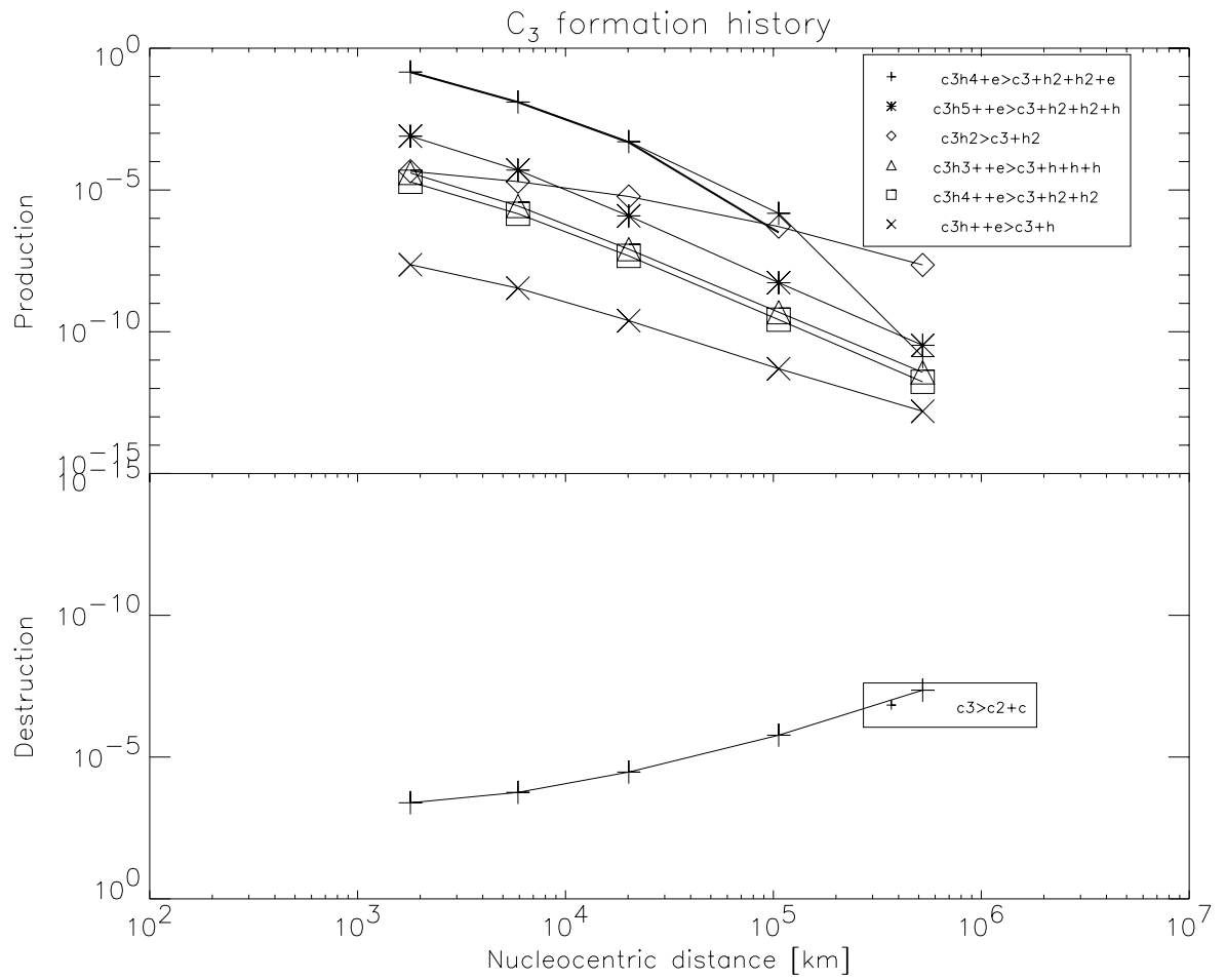
Figure D.6: C_3 formation at 3.78 AU
