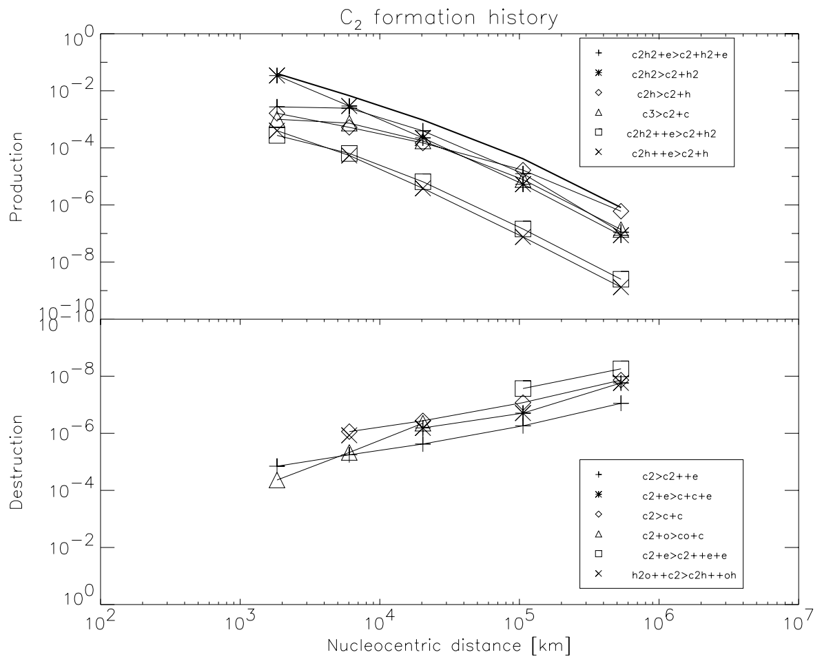
Figure D.10: C_2 formation at 2.86 AU
