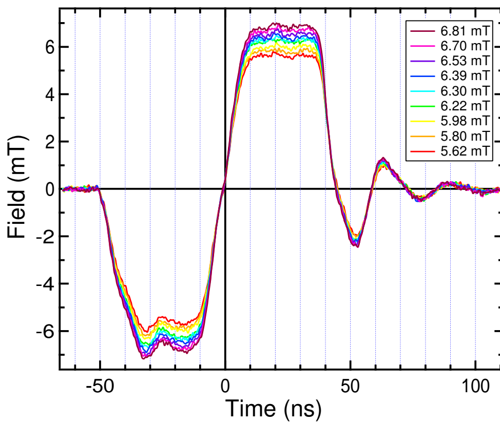
Figure 7.1: All field pulse shapes, ranging from 5.62 mT to 6.81 mT.
