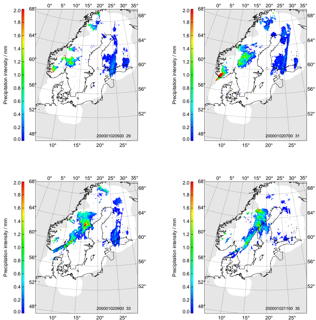
Figure 1: Precipitation rate from 2nd January 2000 05:00 UTC to 11:00 UTC (hour 29, 31, 33 and 35 of January 2000).
