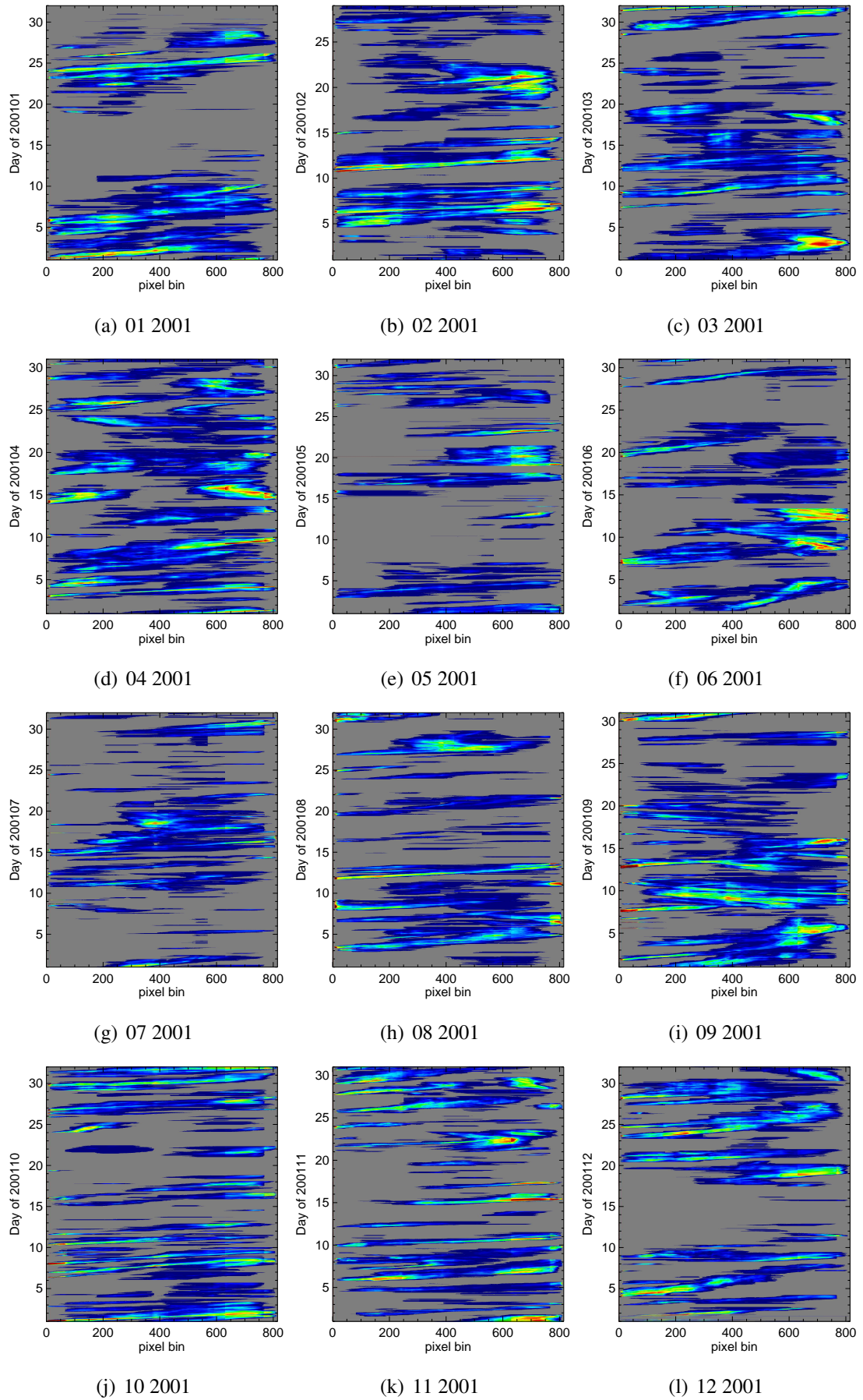
Figure 5: Same as Fig. 4, but for 2001
