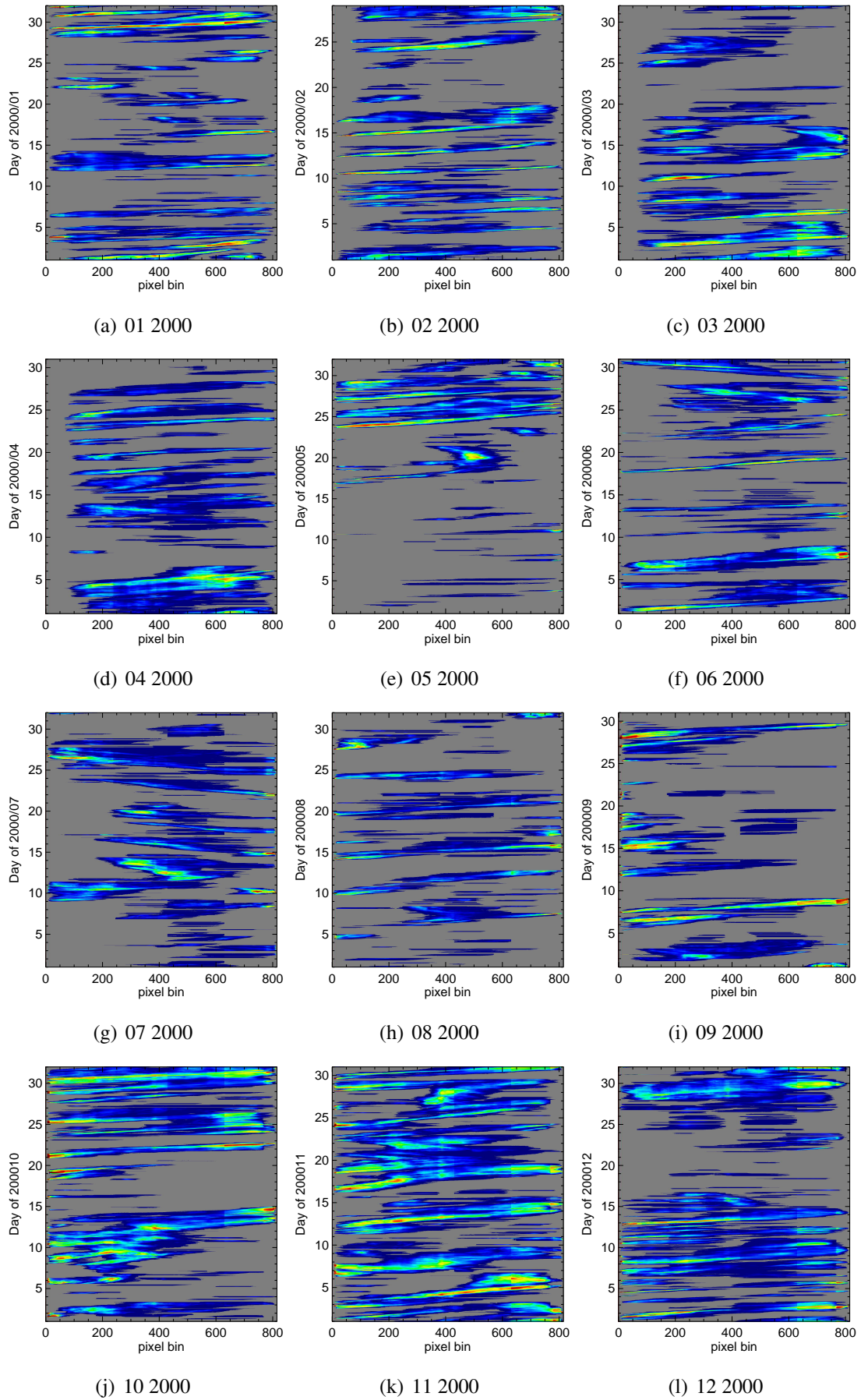
Figure 4: Hovmöller diagrams for January 2000 (a) to December 2000 (l)
