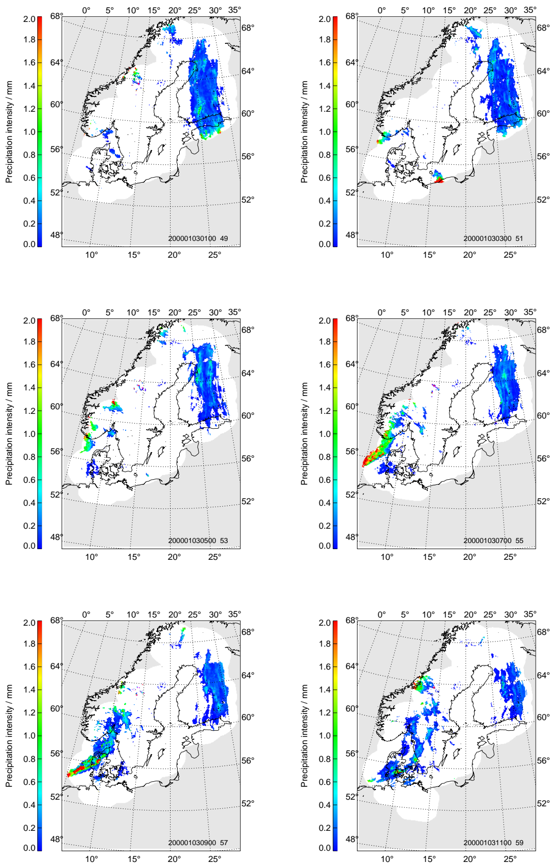
Figure 3: Same as Fig. 1, but for 3rd January 2000 01:00 to 11:00 UTC (hour 49, 51, 53, 55, 57 and 59 of January 2000)
