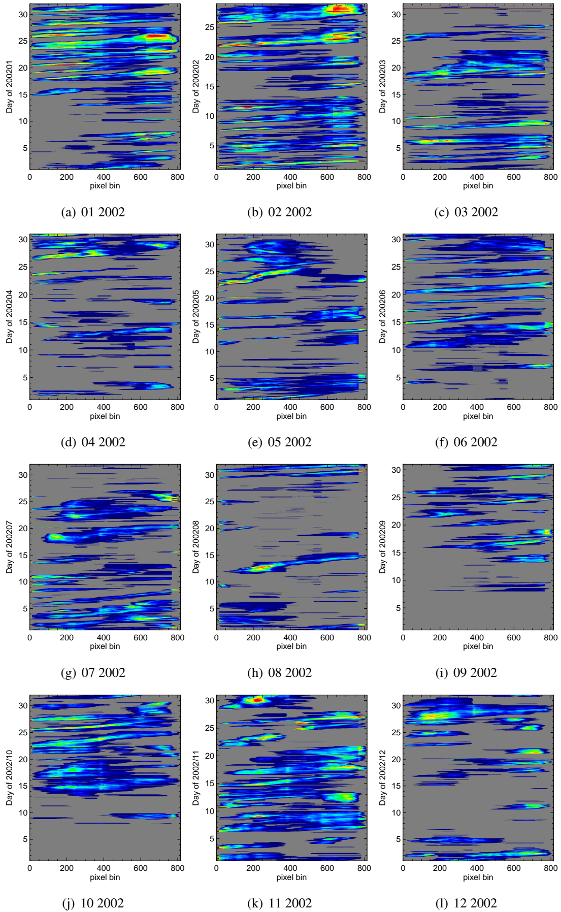
Figure 6: Same as Fig. 4, but for 2002
