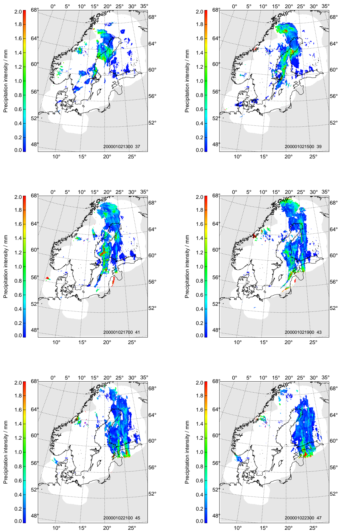
Figure 2: Same as Fig. 1, but for 2nd January 2000 13:00 to 23:00 UTC (hour 37, 39, 41, 43, 45 and 47 of January 2000).
