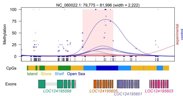
Figure 2. DMR plot displaying a DMR consisting of 13 CpGs with 23% hypomethylation in experimental samples compared to control samples. The methylation level of each CpG site in an individual sample is shown as a point, with its size directly proportional to its coverage. Smoothed methylation levels are represented by lines, separately for control and experimental samples. A track of CpG and gene annotations are additionally displayed under the plot, retrieved from the computed CGI track and org.db package, respectively.
