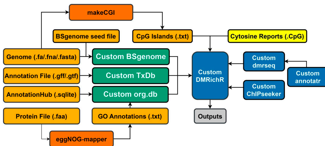
Figure 1. Steps required to adapt DMRichR to a new organism with an annotated genome. Yellow : User input files (methylation calls (.CpG) resulting from a Whole-Genome Bisulfite Sequencing (WGBS) experiment; Light-orange : User input files with information on the reference genome (BSgenome seed files, CpG islands, .fa/.fna/.fasta, .gff/.gtf, .sqlite, .faa, GO Annotations); Dark-orange : Intermediary tools for producing input files (makeCGI, eggNOGmapper); Green : Newly-computed species-specific packages (Custom BSgenome, Custom TxDb, Custom org.db); Blue : Modified versions of DMRichR and additional packages used within it (Custom DMRichR, Custom dmrseq, Custom ChIPseeker, Custom annotatr); Grey : Outputs generated by DMRichR, which include Blocks, Differentially Methylated Regions (DMRs), Smoothed Individual Methylation Values, Heatmaps.
