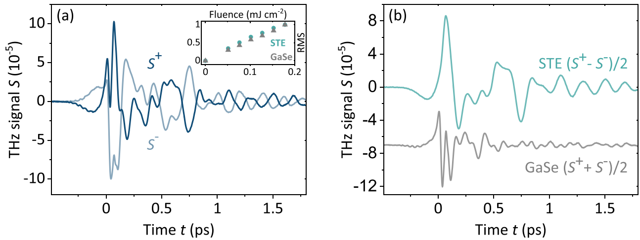
FIG. 2. Raw THz emission signals from the hybrid emitter. (a) Electro-optic signals S^\pm(t) vs time t of the THz field emitted from the hybrid emitter for magnetization directions \pm\mathbf{M} . Signals refer to the field component perpendicular to the in-plane sample magnetization \mathbf{M} . The inset shows the root mean square (RMS) of the THz emission signal vs the pump fluence. (b) Signal components even and odd in \mathbf{M} , i.e., (S^\pm \pm S^\mp)/2 . The two signals represent the signals from the GaSe and STE emitter, respectively. The GaSe signal is vertically offset for clarity.
