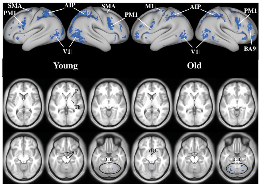
FIGURE 12 Negative fMRI-BOLD signal correlates of \beta -amplitude in left M1. Regions that significantly correlated negatively are indicated in blue (unpaired two group t -test, FDR-corrected p < .05 ). PM1, premotor cortex; M1, motor cortex; AIP, anterior intraparietal area; SMA, supplementary motor cortex; BA9, Brodmann area 9; V1, visual cortex; CB, cerebellum; Th, thalamus; vDC, ventral diencephalon
