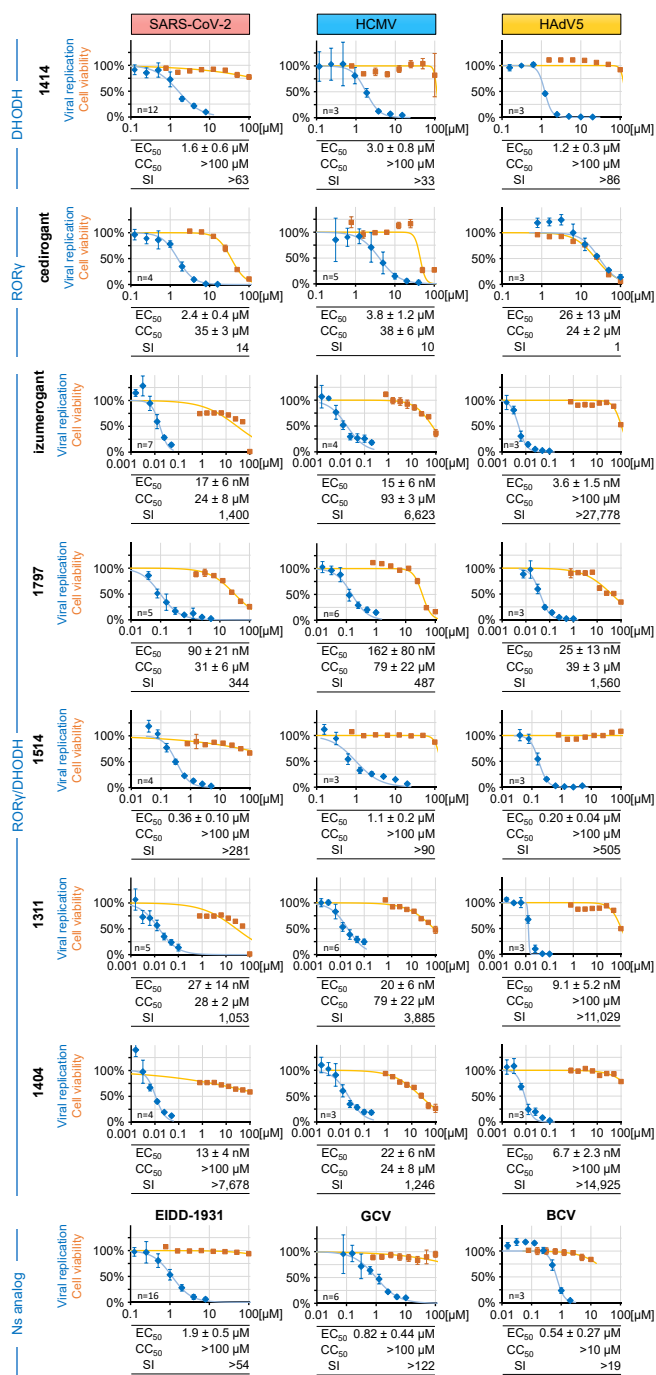
Fig. 2. Antiviral activity of DHODH- and ROR γ -modulating small molecules. Caco-2 cells infected with SARS-CoV-2 d6-YFP, or HFFs infected with HCMV AD169-GFP or A549 cells infected with HAdV5 mneogreen. Cells were subsequently treated with descending concentrations of the DHODH inhibitor 1414 , the ROR γ inverse agonist cedirogant, indicated ROR γ /DHODH dual inhibitors or an appropriate antiviral nucleoside (Ns) analog, i.e. the active metabolite of molnupiravir (EIDD-1931), ganciclovir (GCV) and brincidofovir (BCV). Viral replication was measured by quantitation of the cell-associated YFP/GFP/mNeonGreen fluorescence at 30 h p.i., 7 d p.i. or 3 d p.i. Cell viability was determined in parallel uninfected cell cultures for the equivalent duration of exposure to the compounds. Shown is one representative dataset of the total number of experimental replicates stated in the lower left of each diagram.
