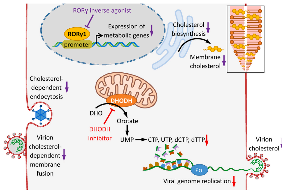
Fig. 6. Schematic representation of the antiviral targets ROR \gamma and DHODH, the associated metabolic pathways and the proposed antiviral mechanism imposed by their inhibition. The inhibition of DHODH reduces the cellular pyrimidine de novo synthesis consequently interfering with the viral genome replication (as indicated in red). In the case of ROR \gamma inhibition, the expression of multiple cholesterol synthesis enzymes is reduced by targeting ROR \gamma as the responsible transcription factor (as indicated in violet). The proposed antiviral mechanism is presented by membrane remodeling events, e.g. viral membrane fusion with target cells or viral uptake by endocytosis. DHO, dihydroorotate; UMP, uridine monophosphate; CTP, cytidine triphosphate; UTP, uridine triphosphate; dCTP, deoxycytidine triphosphate; dTTP, deoxythymidine triphosphate.
