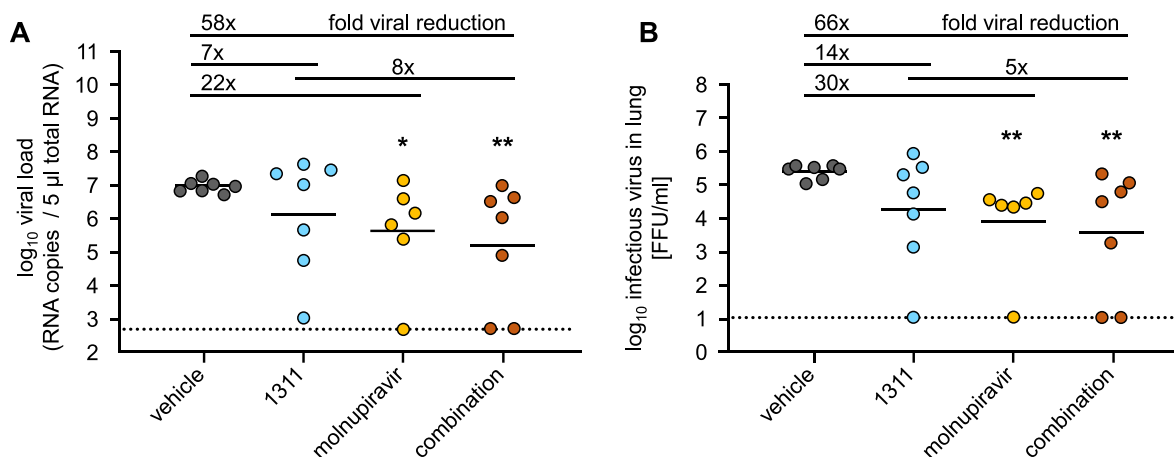
Fig. 5. The ROR \gamma /DHODH dual inhibitor 1311 enhances the antiviral activity of molnupiravir in vivo . Female K18-hACE-2 mice received either vehicle (grey), 1311 (blue), molnupiravir (orange) or a combination of 1311 and molnupiravir (red) via oral gavage and were infected with SARS-CoV-2 (Wuhan strain). At day 4 after virus inoculation, the lungs were removed. (A) RNA was isolated from lung homogenates and viral genome copies were quantified via RT-qPCR. Data points shown represent viral copy numbers with the geometric mean of each group. The fold reduction in viral load of the vehicle control to the three compound-treated groups as well as 1311 to the combination treatment group is indicated. Statistical evaluation of the data was performed by Mann-Whitney U test in comparison to vehicle control (*: p \leq 0.05 ; **: p \leq 0.01 ). (B) Lung homogenate was titrated on Vero cells and SARS-CoV-2 infected cells were visualized after 30 h using spike-specific immunochemistry staining. Data points shown represent infectious units/mL of each animal with geometric mean of each group. Each point represents one mouse. Calculated reduction is shown in comparison to vehicle control. Statistical evaluation of the data was performed by Mann-Whitney U test in comparison to vehicle control (**, p \leq 0.01 ).
