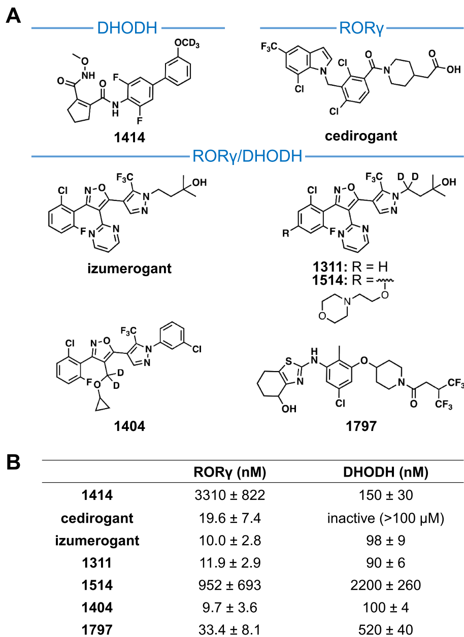
Fig. 1. Chemical structures and single target activities of selected compounds. (A) Chemical structures of the ROR \gamma inverse agonist cediogant, the DHODH inhibitor 1414 , and ROR \gamma /DHODH dual inhibitors izumerogant, 1797 , 1514 , 1311 and 1404 . (B) Single target IC 50 values for DHODH inhibition measured by a cell-free enzyme activity assay and for ROR \gamma determined by a reporter cell-based luciferase assay. Mean values ± standard deviation from at least three independent experiments are depicted.
