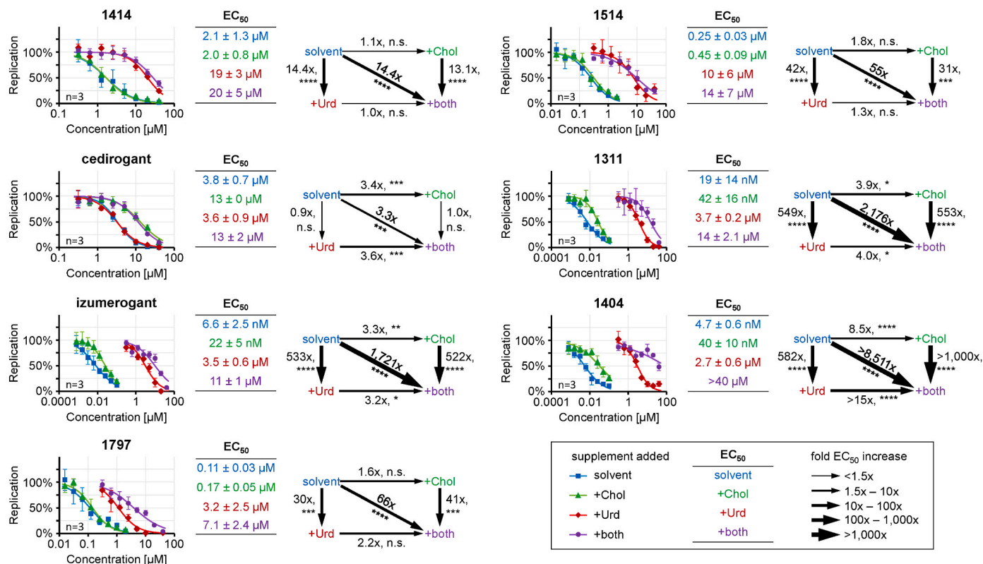
Fig. 3. Partial reversal of the antiviral effects by the supplementation with exogenously added cholesterol or uridine. Caco-2 cells infected with SARS-CoV-2 d6-YFP were treated with descending concentrations of the DHODH inhibitor 1414 , the ROR \gamma inverse agonist cediogant or indicated ROR \gamma /DHODH dual inhibitors. For each setting, one of four parallel titrations was either supplemented with solvent (blue), cholesterol-PEG600 equivalent to 300 \mu M free cholesterol (+Chol, green), 100 \mu M uridine (+Urd, red) or a combination of Chol and Urd (+both, violet). EC 50 values were determined from the dose responses for three independent experiments. The mean increases of EC 50 in response to metabolite supplementation were determined and graphed in an arrow diagram. The direction of the arrow indicates the nature of the change. An arrow pointing right indicates an increase mediated by the addition of cholesterol, whereas an arrow pointing downwards indicates the effect of uridine. The diagonal arrow indicates the change induced by both supplements. The fold change values are depicted adjacent to the arrows and are additionally represented by the line thickness of the arrows. Statistical evaluation was performed using the one-way ANOVA with the Tukey's multiple comparison post-hoc test on the log 10 -transformed EC 50 values. n.s., not significant; *, p < 0.05 ; **, p < 0.01 ; ***, p < 0.001 ; ****, p < 0.0001 .
