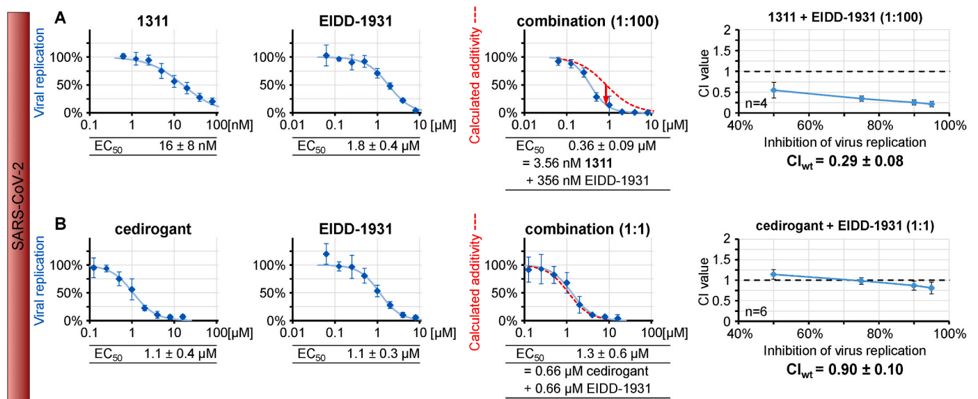
Fig. 4. The ROR \gamma /DHODH dual inhibitor 1311 exhibits a synergistic drug interaction with EIDD-1931. (A) Caco-2 cells were infected with SARS-CoV-2 d6-YFP and treated with the dual ROR \gamma /DHODH inhibitor 1311, EIDD-1931 or a combination of both in a 1:100 ratio. (B) In parallel, cells were treated with either the ROR \gamma inverse agonist cedirogant, EIDD-1931, or a combination of both drugs in a 1:1 ratio. Combination indices (CI) were calculated for 50, 75, 90, and 95% virus inhibition using the CompuSyn algorithm. Values represent mean \pm SD for independent biological replicates. CI wt < 0.3, strongly synergistic; 0.3–0.7, synergistic; 0.7–0.85, moderately synergistic; 0.85–0.9, slightly synergistic; 0.90–1.10, (nearly) additive; 1.10–1.20, slightly antagonistic; 1.20–1.45, moderately antagonistic; 1.45–3.3, antagonistic; >3.3, strongly antagonistic (Chou, 2006).
