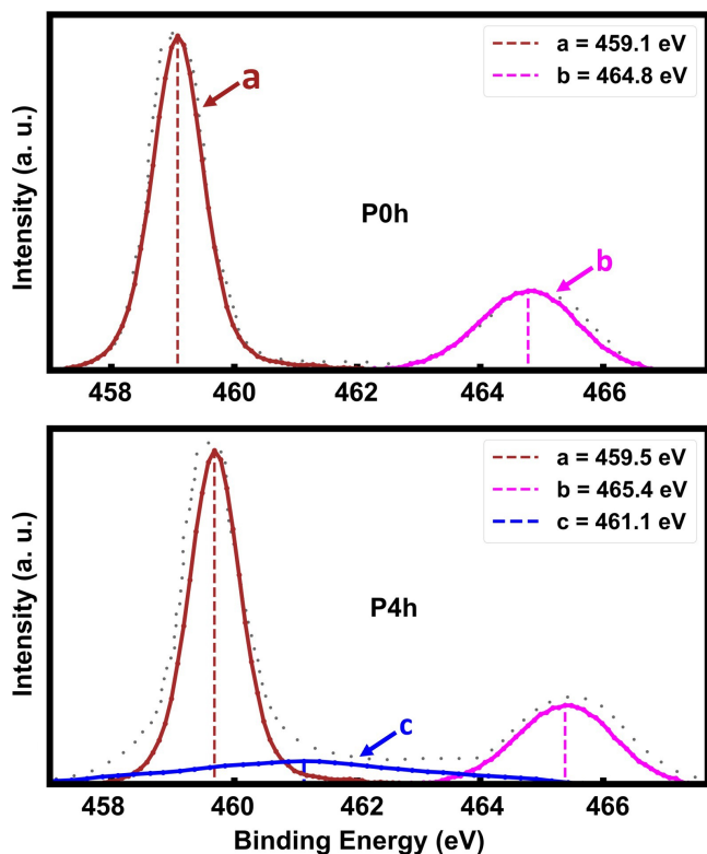
FIGURE 4 X-ray photoelectron spectroscopy data showing the (a) Ti^{4+}2p_{3/2} , (b) Ti^{4+}2p_{1/2} , and (c) Ti^{3+}2p_{3/2} states of P0h and P4h samples.
