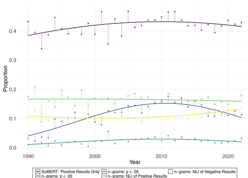
Figure 4. Comparison of predicted proportions of positive and negative results in psychotherapy RCTs (1990–2022): rule-based approaches versus SciBERT model. n = 20,212 ; NLI = natural language indicator; dots represent observed values. Bent lines correspond to predicted proportions of PRO per year by SciBERT (M3b), p < .05 (M4a), p > .05 (M4b), natural language indicators of positive results (M4c), and natural language indicators of negative results (M4d).
