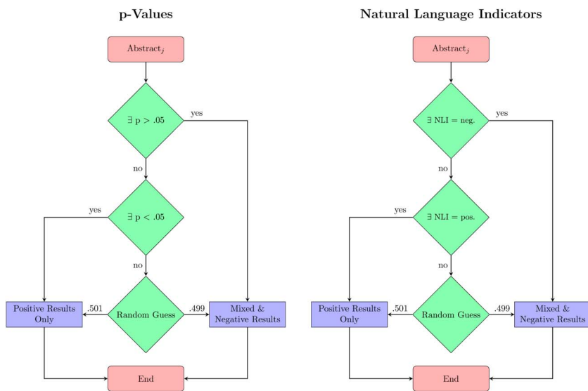
Figure 2. Algorithms for rule-based classification based on p -values and natural language indicators of positive and negative results. NLI = natural language indicators; \exists = "At least one..."; .501 = proportion of positive results only in training data; .499 = proportion of mixed or negative results in the training data.
