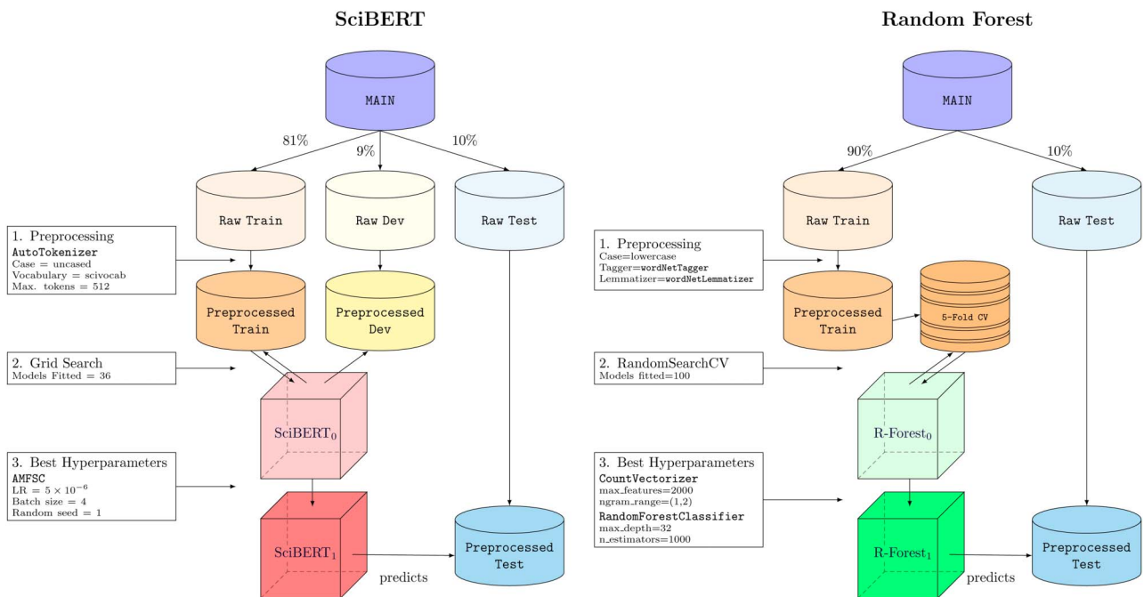
Figure 1. Flowchart of the SciBERT and random forest pipelines. LR = learning rate; AMFSC = AutoModelForSequenceClassification; CV = cross-validation; cylinders represent data sets and cubes represent models; SciBERT train data: n = 1,602 ; SciBERT dev data: n = 178 ; random forest train data: n = 1,780 ; test data for both models: n = 198 .
