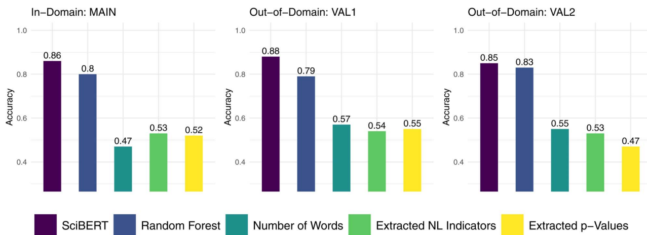
Figure 3. Comparing model performances across in-domain and out-of-domain data. Colored bars represent different model types. Samples: MAIN test: n = 198 abstracts; VAL1: n = 150 abstracts; VAL2: n = 150 abstracts.
