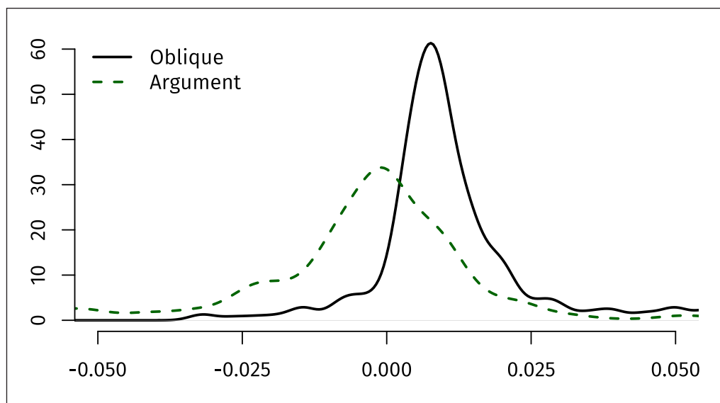
Figure 1: Density estimate of the distributions of the association scores, separately for the two semantic relations; the x-axis was truncated at -0.05 and 0.05 where the curves are essentially flat.
