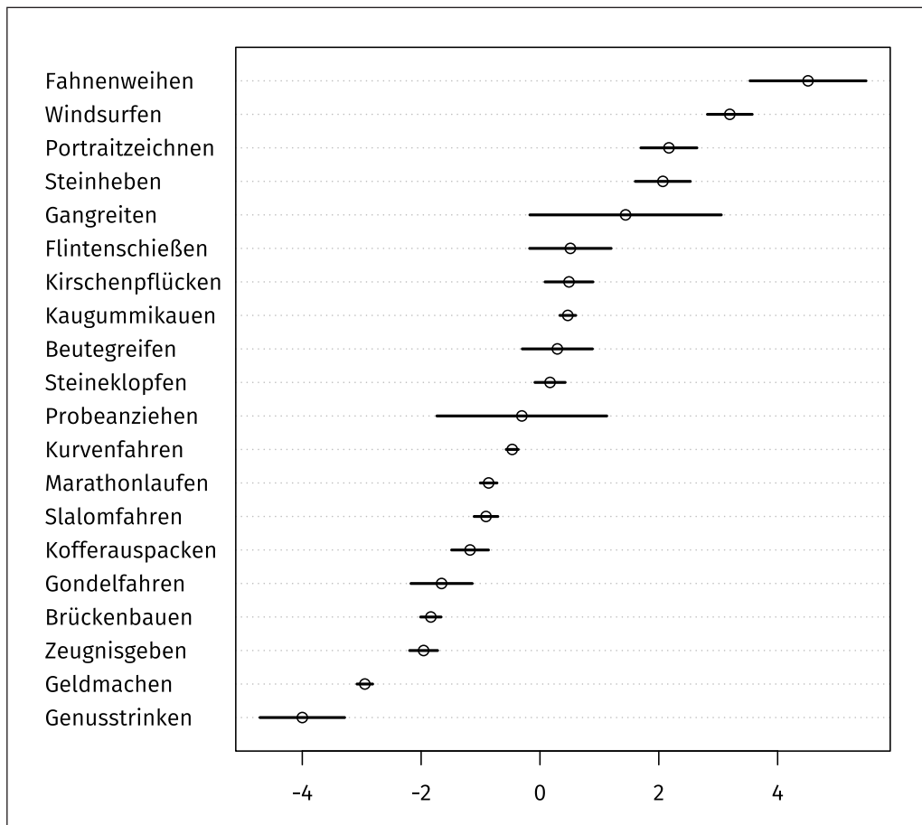
Figure 3: A random selection of conditional modes with 95% prediction intervals for the levels of the random effect in the GLMM modelling the corpus data.
