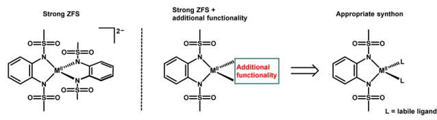
Scheme 1 Conceptual approach: a modular route to functional heteroleptic structures requires appropriate synthons.
