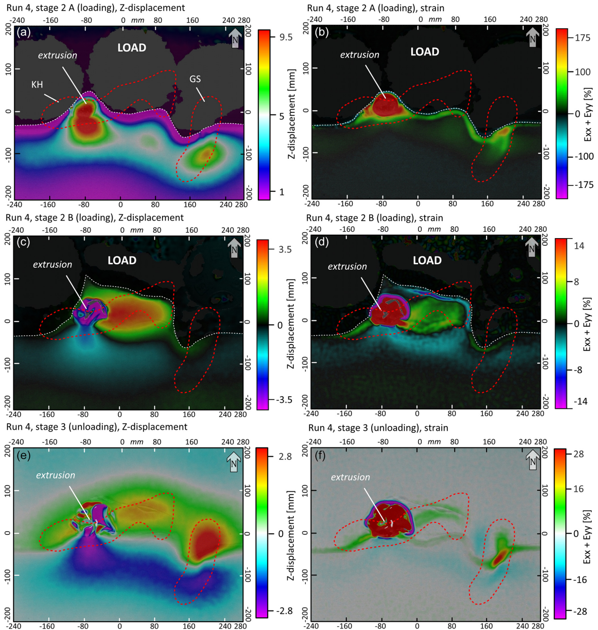
Figure 10. Summarizing DIC imagery of run 4. In stage 2A and 2B, the load was applied to the north of the dotted white line. (a) Z map showing total vertical displacement (in mm) of stage 2A. (b) Strain (%) map of the total strain of stage 2A. (c) Z map showing total vertical displacement (in mm) of stage 2B. (d) Strain (%) map of the total strain of stage 2B. (e) Z map showing total vertical displacement (in mm) of stage 3. (f) Strain (%) map of the total strain of stage 3. Dashed red outlines depict the approximate position of the salt structures.
