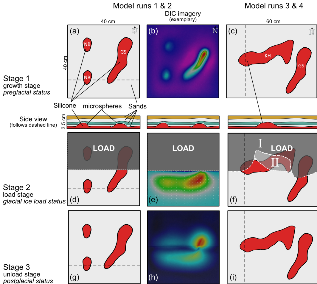
Figure 5. Sketch illustrating the general physical model setup and the three model stages. The left column (a, d, g) depicts the setup of model runs 1 and 2; the middle column (b, e, h) shows exemplary DIC imagery of these runs. The right column (c, f, i) depicts the setup of model runs 3 and 4, where the two domes were replaced by the KH salt pillow, which was parallel to the load margin. Panel (f) shows the load margin; in model run 4, first the areas “I” and “II” were loaded for 24 h, and then area “II” was unloaded, and area “I” was kept under load for another 24 h. The dashed light gray line in left and right columns (a, d, g, c, f, i) depicts the orientation of the sections (Fig. 8).
