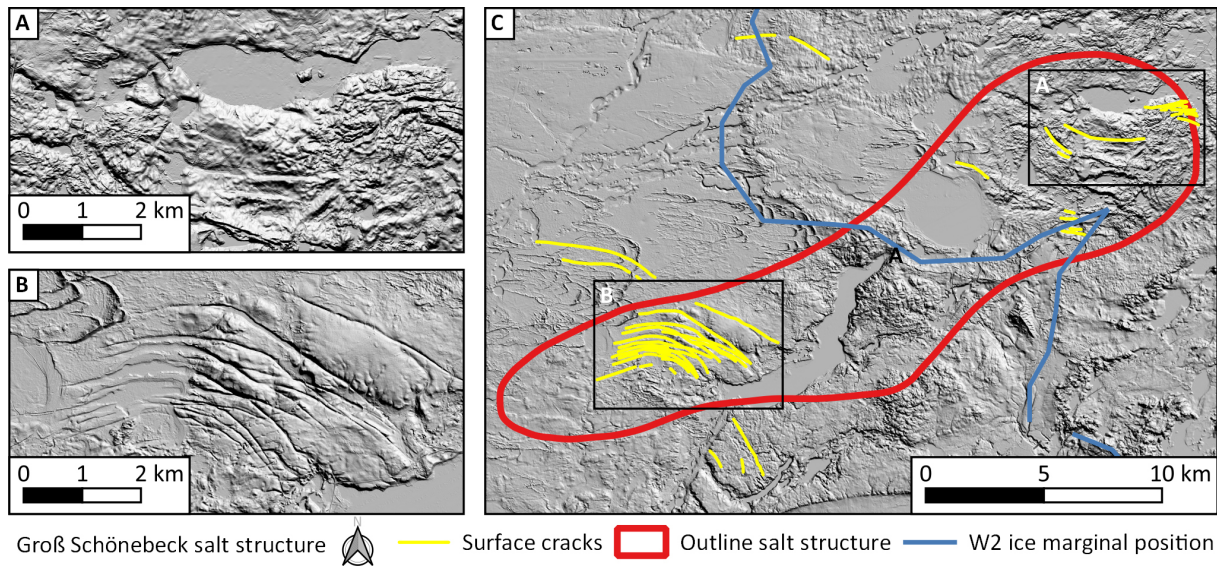
Figure 2. Hillshade maps of the Groß Schönebeck salt pillow region. (a) Detailed view of the surface cracks found at the land surface atop the salt pillow in the Altkünkendorf area. (b) Detailed view of the surface cracks found at the land surface atop the salt pillow in the Schorfheide area. (c) Location of the surface cracks with relation to the outline of the buried salt structure. Hillshade with 5× vertical exaggeration based on 1 m lidar digital terrain model (GeoBasis-DE/LGB, 2020).
