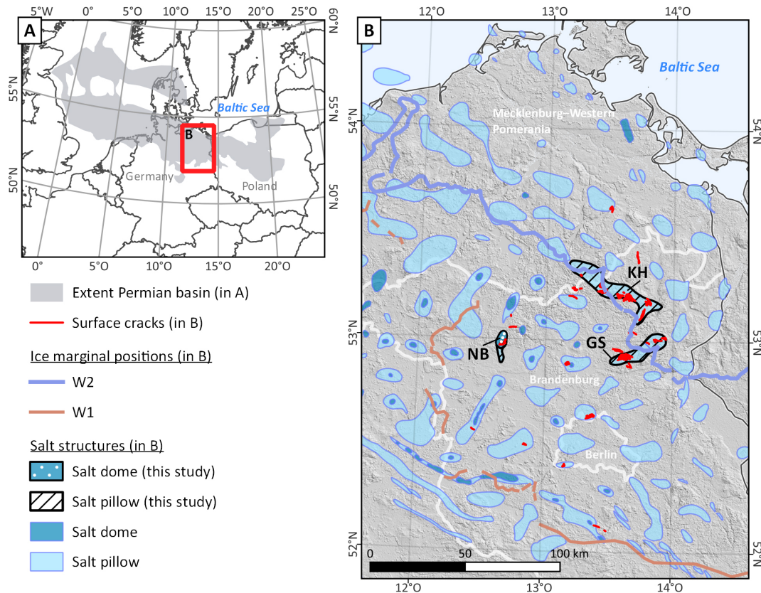
Figure 1. Overview map. Bright blue polygons are salt pillows; dark blue polygons are salt domes (InSpEE, 2015). Polygons with a black outline show salt structures investigated in this study (see Figs. 2–5 for detailed maps). GS – Groß Schönebeck study site; KH – Klaushagen study site; NB – Netzeband study site. Brown line is the W1 ice extent; blue line is the W2 ice extent (Lüthgens and Hardt, 2022; Lüthgens et al., 2020). White lines in panel (b) are German administrative borders plotted for orientation. Hillshade map in panel (b) is based on the Shuttle Radar Topography Mission (SRTM) digital elevation model (Jarvis et al., 2008).
