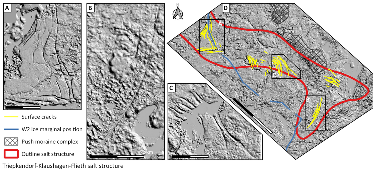
Figure 3. Hillshade maps of the Triepkendorf–Klaushagen–Flieth salt structure region. (A) Detailed view of the surface cracks found at the land surface atop the salt pillow in the Thomsdorf area. (B) Detailed view of the surface cracks found at the land surface atop the salt pillow in the Friedrichswalde area. (C) Detailed view of the surface cracks found at the land surface atop the salt pillow in the lake Kuhzer See area. (D) Location of the surface cracks with relation to the outline of the salt structure. Hillshade with 5× vertical exaggeration based on 1 m lidar digital terrain model (GeoBasis-DE/LGB, 2020).
