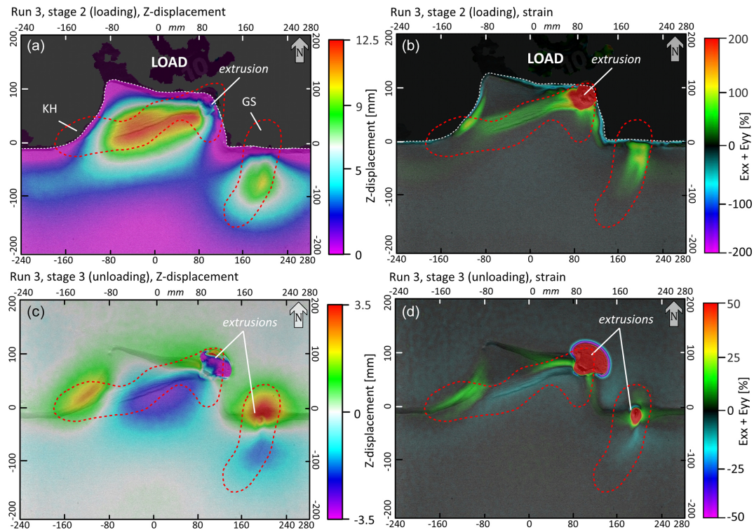
Figure 9. Summarizing DIC imagery of run 3. In stage 2, the load was applied to the north of the dotted white line. (a) Z map showing total vertical displacement (in mm) of stage 2. (b) Strain (%) map of the total strain of stage 2. (c) Z map showing total vertical displacement (in mm) of stage 3. (d) Strain (%) map of the total strain of stage 3. Dashed red outlines depict the approximate position of the salt structures.
