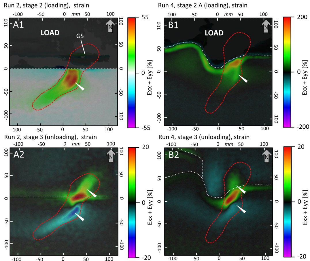
Figure 12. Comparison of strain patterns above GS pillow using different load geometries (dashed white line). (a1, a2) Straight load margin. (b1, b2) Lobate load margin. Dashed red outlines depict the approximate position of the salt structures. White arrows indicate the position of the crestal graben structures.
