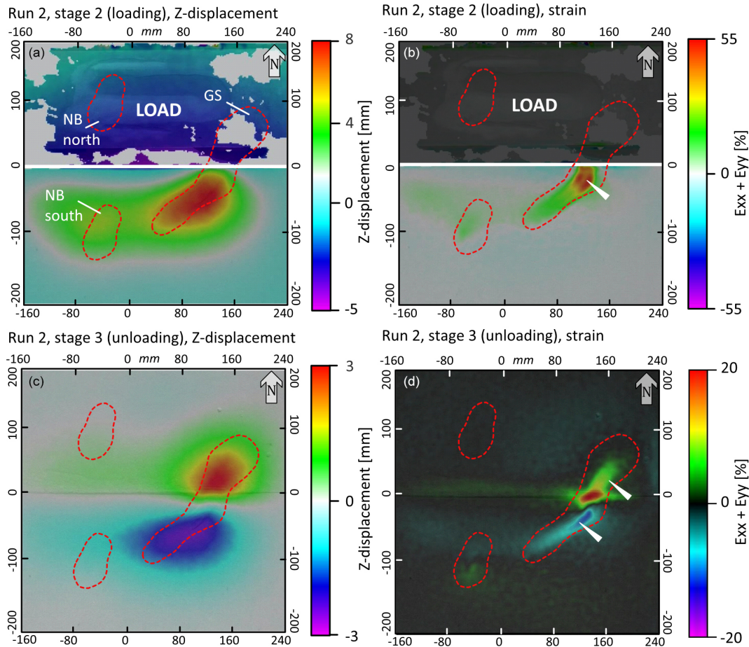
Figure 6. Summarizing DIC imagery of run 2. In stage 2, the load was applied to the north of the horizontal white line. (a) Z map showing total vertical displacement (in mm) of stage 2. The gray colors in the upper half of the figure are “no data” areas. (b) Strain (%) map of the total strain of stage 2. (c) Z map showing total vertical displacement (in mm) of stage 3. (d) Strain (%) map of the total strain of stage 3. Dashed red outlines depict the approximate position of the salt structures. White arrows indicate the position of the crestral graben structure.
