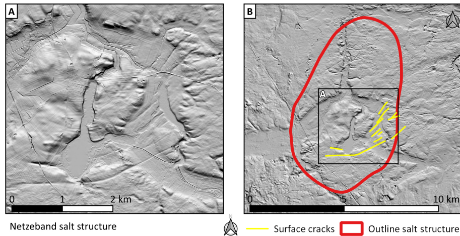
Figure 4. Hillshade maps of the Netzeband salt dome region. (a) Detailed view of the surface cracks found at the land surface atop the salt dome. (b) Location of the surface cracks with relation to the outline of the salt structure. Hillshade with 5\times vertical exaggeration based on 1 m lidar digital terrain model (GeoBasis-DE/LGB, 2020).
