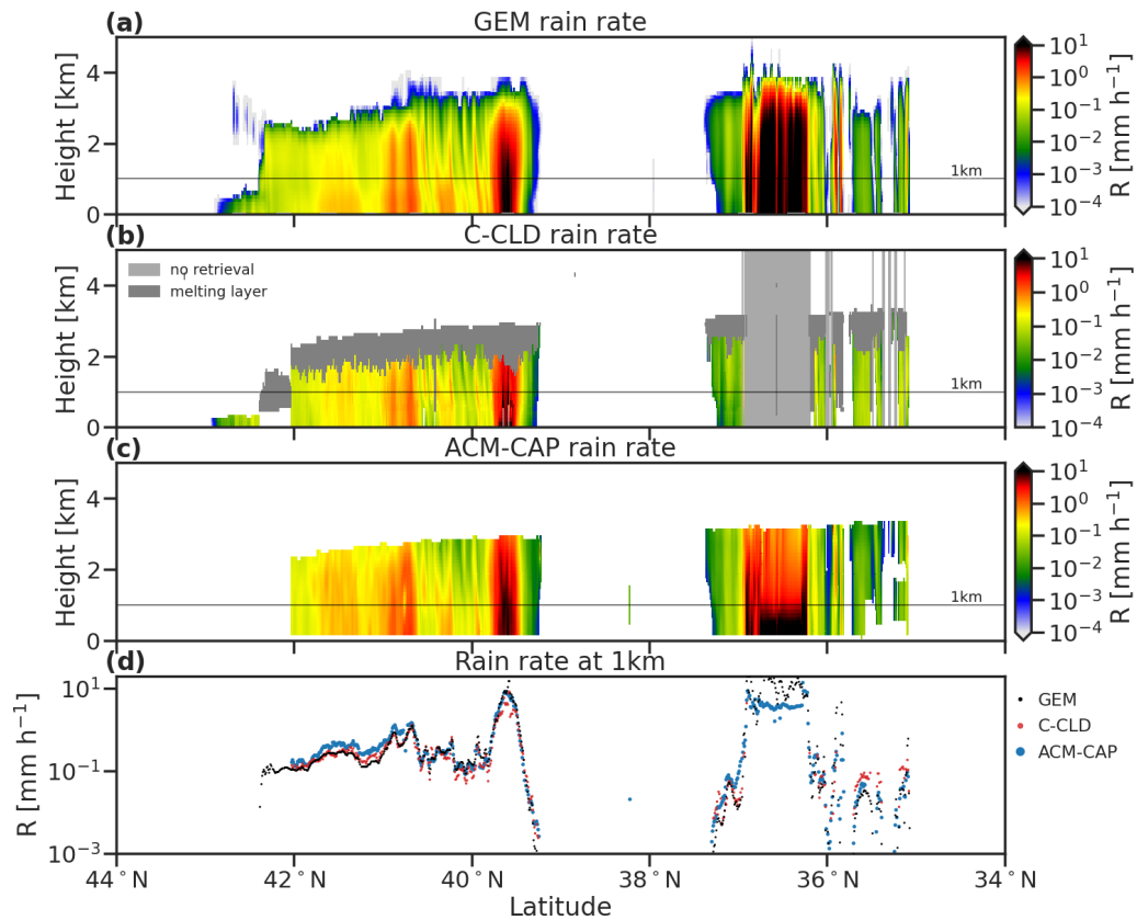
Figure 11. GEM (a), C-CLD (b), and ACM-CAP (c) profiles of rain rate for the Halifax scene. A comparison of GEM and retrieved rain rates at 1 km are shown in panel (d). Shading in panel (b) indicates that C-CLD does not retrieve profiles that are strongly affected by multiple scattering and/or extinction of the CPR signal, and all melting snow is treated separately from the rain retrieval.
