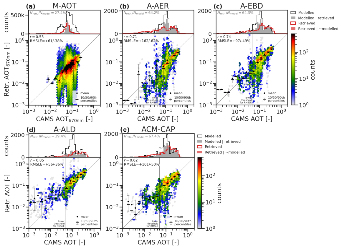
Figure 14. The same as Fig. 2, showing retrieved total aerosol optical thickness (AOT) from (a) M-AOT at 670 nm, (b) A-AER, (c) A-EBD, (d) A-ALD, and (e) ACM-CAP at 355 nm across all simulated test scenes. Due to the need to avoid contamination from cloud in aerosol-only profiles and increase the number of samples, the M-AOT evaluation (a) uses data from across the MSI swath rather than just nadir pixels, drastically increasing the number of samples used in this panel.
