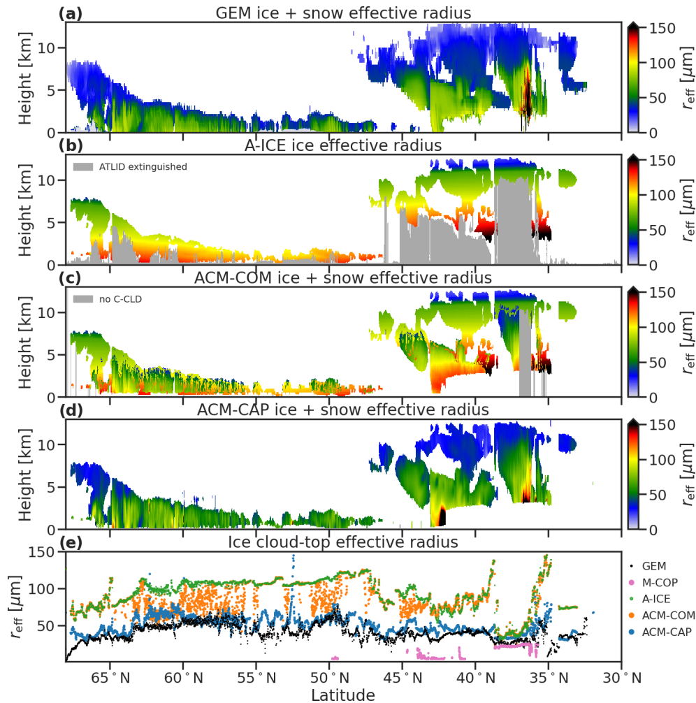
Figure 4. Profiles of ice cloud effective radius from (a) GEM, (b) A-ICE, (c) ACM-COM, and (d) ACM-CAP for the Halifax scene. Panel (e) intercompares GEM and retrieved cloud-top effective radius (averaged where optical thickness is less than 1). Shading in panel (b) indicates where A-ICE cannot retrieve the ice cloud effective radius due to the extinction of ATLID signal, and shading in panel (c) indicates where ACM-COM has no information due to C-CLD not retrieving in profiles strongly affected by multiple scattering or attenuation of CPR signal. Note that C-CLD does not report ice cloud effective radius, so that product is not included in this comparison.
