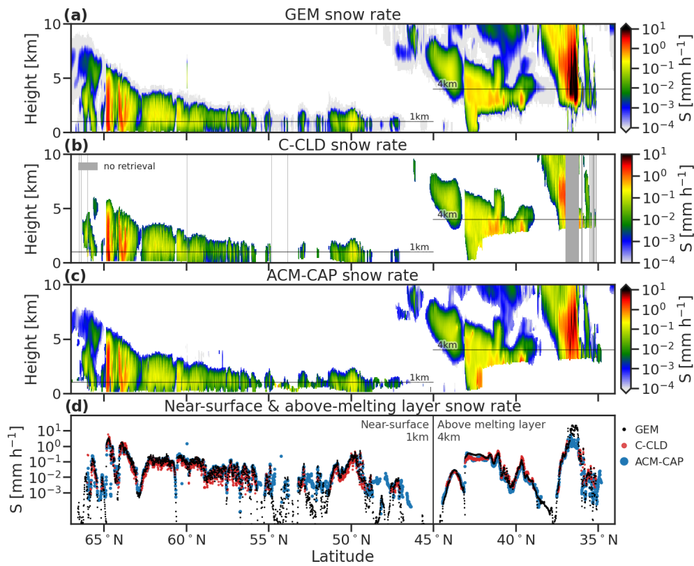
Figure 5. Snow rate from (a) GEM, (b) C-CLD, and (c) ACM-CAP and (d) an intercomparison at selected levels over the Halifax scene. Shading in panel (b) indicates where C-CLD does not retrieve profiles where CPR is affected by multiple scattering and/or attenuation.
