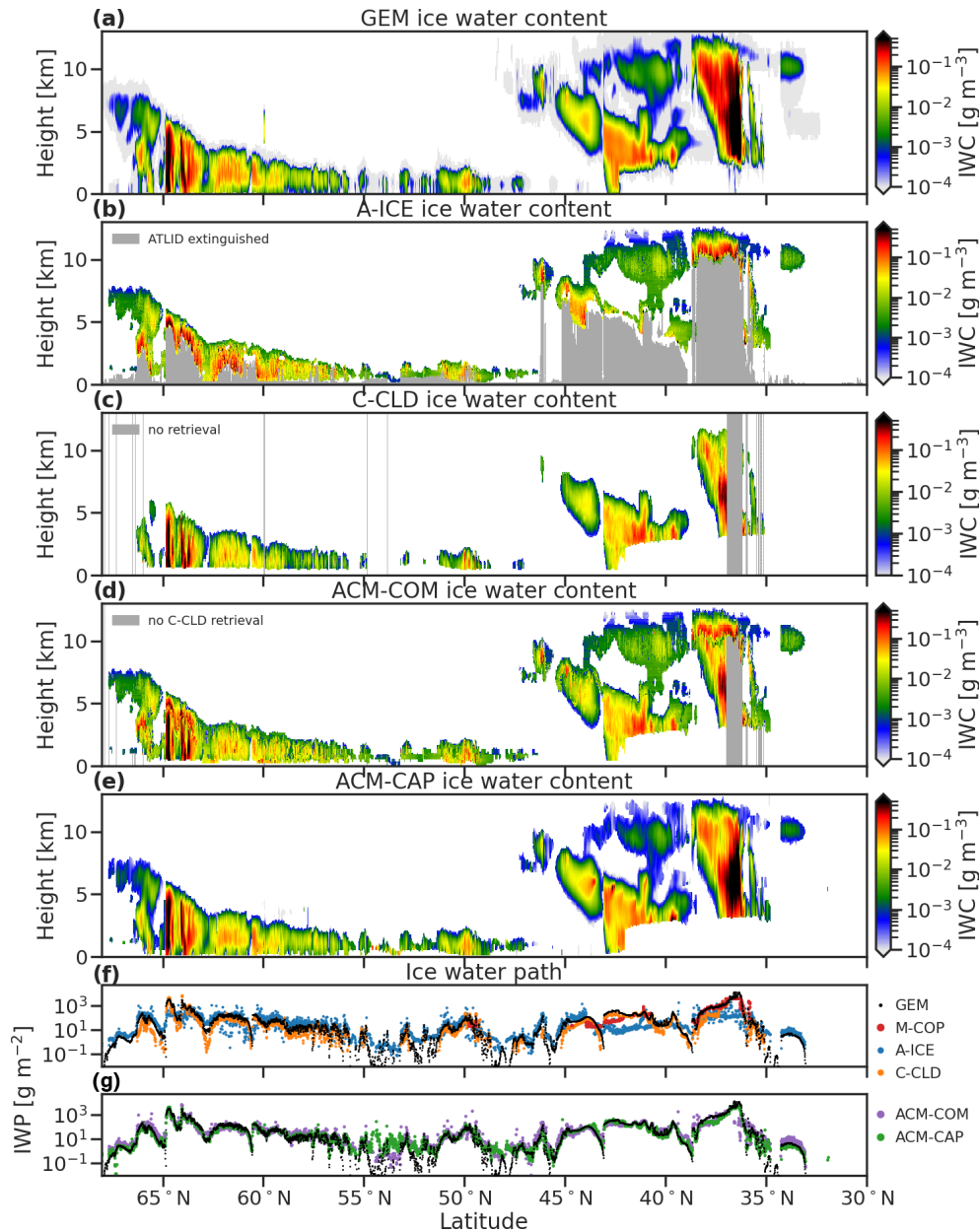
Figure 1. Ice water content from (a) GEM, (b) A-ICE, (c) C-CLD, (d) ACM-COM, and (e) ACM-CAP for the Halifax scene. (f) The corresponding intercomparison of retrieved ice water paths, including M-COP, presented over duplicated axes for clarity. Shading in panel (b) indicates where A-ICE cannot retrieve ice clouds due to the extinction of the ATLID signal; shading in panels (c) and (d) indicates profiles not retrieved by C-CLD due to multiple scattering or attenuation of CPR signal.
