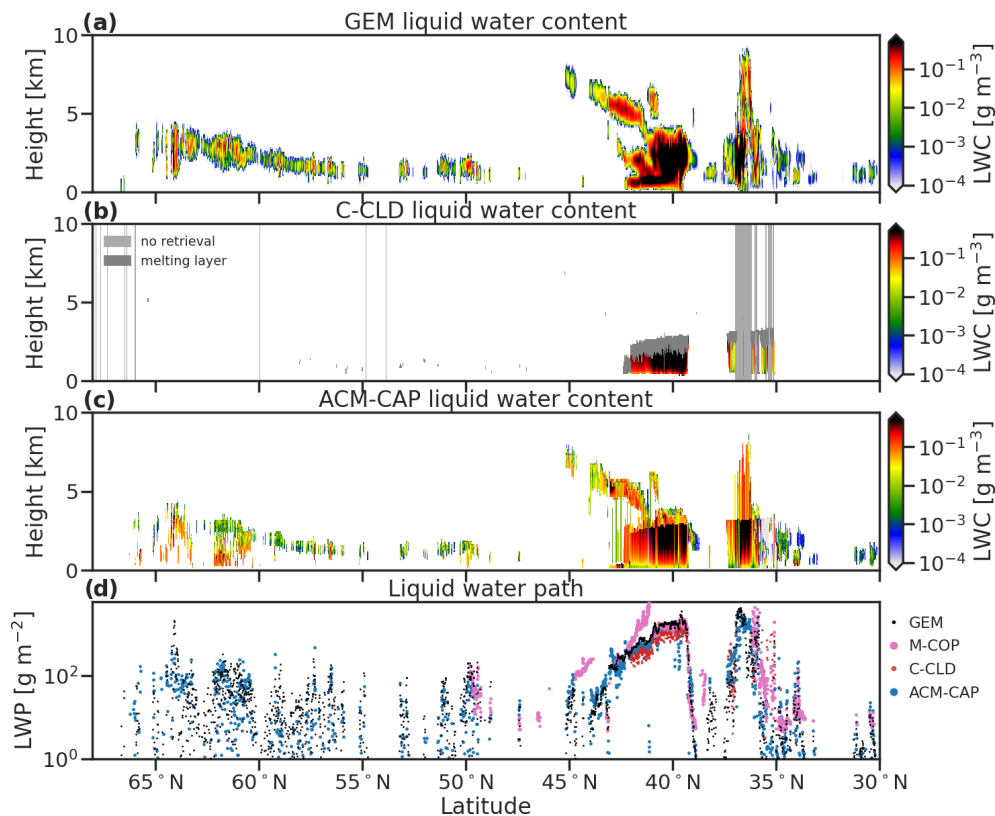
Figure 7. Liquid water content profiles for the Halifax scene from (a) GEM, (b) C-CLD, and (c) ACM-CAP. Panel (d) compares the liquid water paths retrieved by C-CLD, ACM-CAP, and M-COP at the nadir pixel. Shading in panel (b) indicates that C-CLD does not retrieve profiles that are strongly affected by multiple scattering and/or extinction in the CPR signal; liquid water is only retrieved where coincident with rain and not the melting layer.
