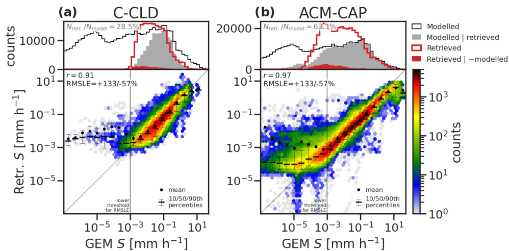
Figure 6. As for Fig. 2 but for snow rate (i.e. ice mass flux) from (a) C-CLD and (b) ACM-CAP for all test scenes against that from the combination of all ice species in GEM.
