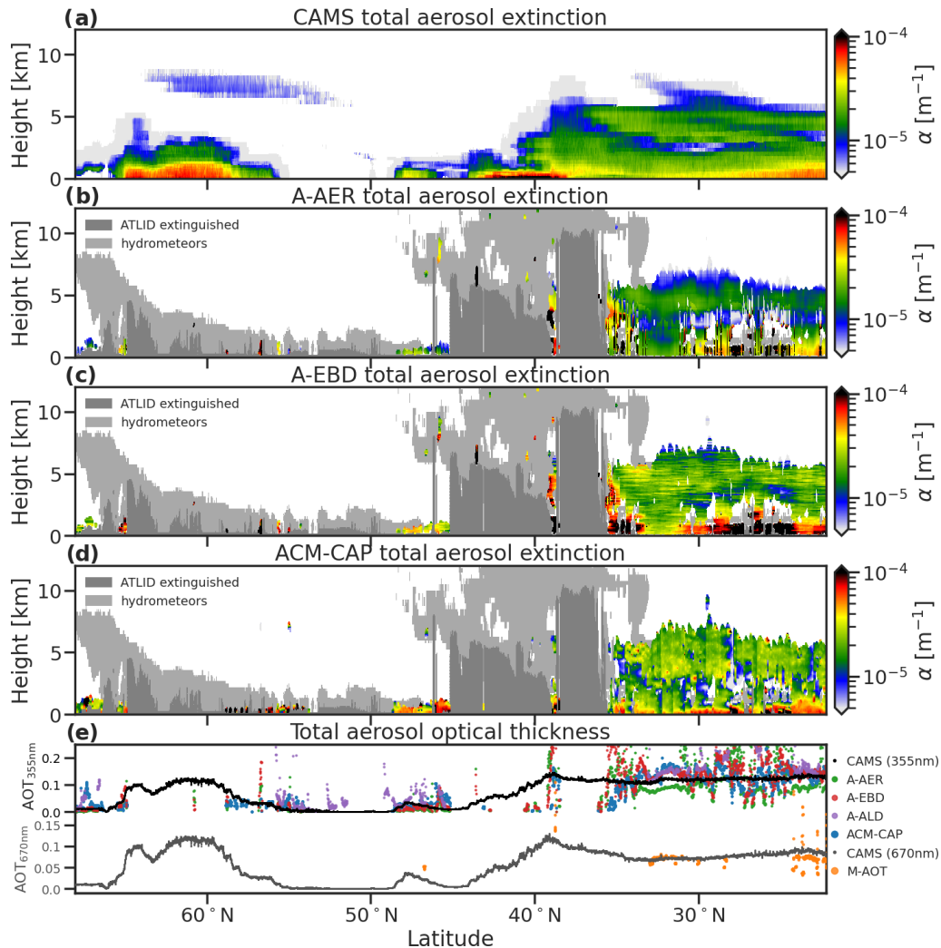
Figure 13. Profiles of total aerosol extinction from (a) the CAMS model, (b) A-AER, (c) A-EBD, and (d) ACM-CAP, and (e) the total aerosol optical thickness from A-EBD, A-AER, A-ALD and ACM-CAP (at 355 nm), and the passive M-AOT (at 670 nm), for the Halifax scene. Shading over the A-EBD, A-AER, and ACM-CAP profiles indicates where aerosol retrievals are not available due to the complete extinction of ATLID signal and the presence of other targets.
