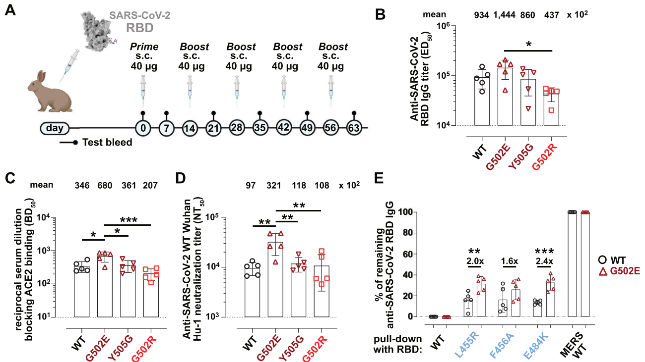
Figure 6. SARS-CoV-2 RBD G502E improves neutralizing antibody titers. (A) Scheme representing the RBD immunization regimen. s.c., subcutaneous. (B) Anti-RBD WT IgG depicted as ED 50 , (C) reciprocal serum dilution to block 50% of ACE2 binding to the RBD WT (BD 50 ), and (D) neutralization of virus particles pseudotyped (PsV) with SARS-CoV-2 spike WT (NT 50 ) determined at day 35 after prime for animals immunized with recombinant RBD WT, G502E, Y505G, G502R ( n = 5 rabbits per condition). Samples were subjected to ordinary one-way ANOVA with Tukey's multiple comparison test. (E) Rabbit sera ( n = 5 rabbits per condition) were depleted via RBD pull-down as shown in Fig. 5F and Supporting information Fig. S4B. One-tailed unpaired t-test was applied. In (B–E), mean \pm SD is shown. * p < 0.05; ** p < 0.01; *** p < 0.001. RBD, receptor binding domain.
