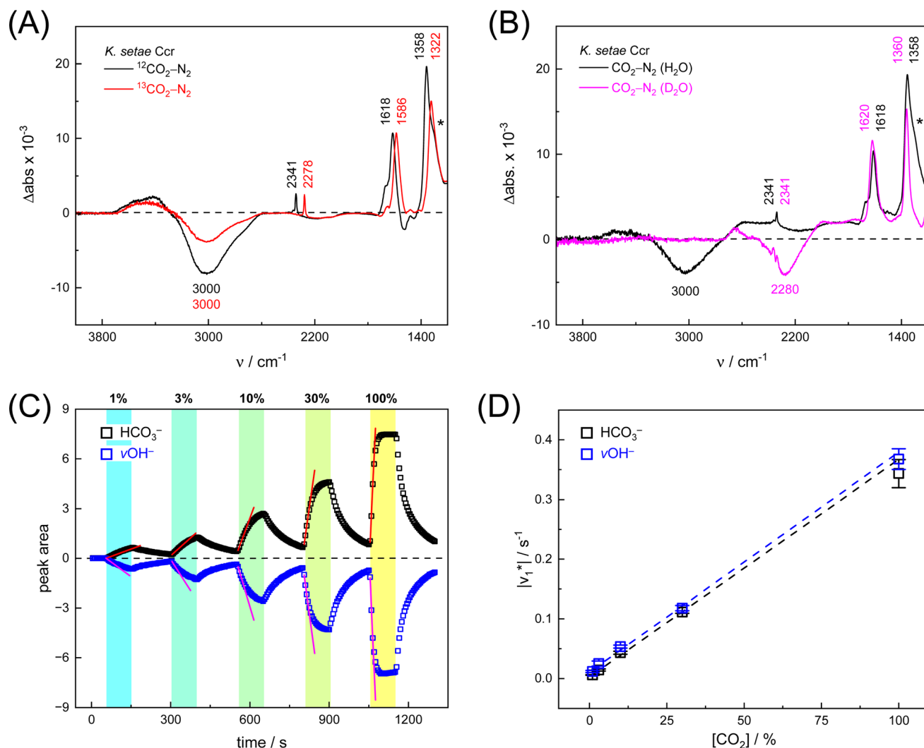
Fig. 2 Infrared characterization of the reaction of KsCcr with \text{CO}_2 . (A) ' \text{CO}_2 - \text{N}_2 ' ATR FTIR difference spectra for the reaction with ^{12}\text{CO}_2 (black) or ^{13}\text{CO}_2 (red). Positive signals are assigned to \text{CO}_2 (2341 or 2278 \text{cm}^{-1} ) and \text{HCO}_3^- . The COH vibration ( \nu_4 ) appears as a shoulder at 1298 \text{cm}^{-1} (*). (B) ' \text{CO}_2 - \text{N}_2 ' ATR FTIR difference spectra in the presence of \text{H}_2\text{O} (black) or \text{D}_2\text{O} (magenta). The broad negative bands are assigned to 'local' water with \text{vOH}^- = 3000 \text{ cm}^{-1} and \text{vOH}^- = 2280 \text{ cm}^{-1} . (C) Evolution of the bands assigned to \text{HCO}_3^- (black) and \text{vOH}^- (blue) over time in the presence of 1–100% \text{CO}_2 or 100% \text{N}_2 . Red lines represent linear fits of the first three data points after gas exchange to calculate the initial reaction velocity v_1^* . (D) Plot of the apparent reaction velocity |v_1^*| of the initial \text{HCO}_3^- formation (black) or initial water consumption (blue) in the \text{CO}_2 hydration reaction.
