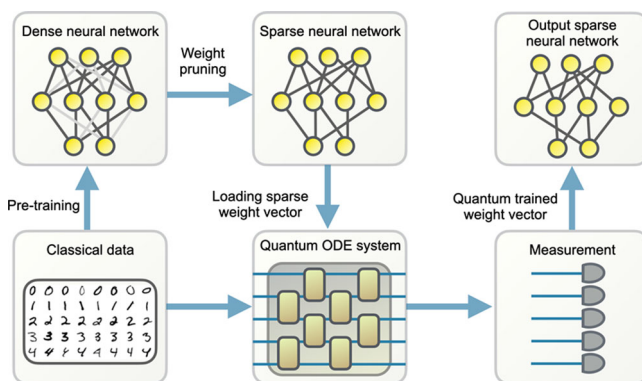
Fig. 1 | A possible learning process in large-scale models, which might use sparse training, whose early stage in learning might admit possible quantum enhancement. A dense neural network is pre-trained classically. The neural network weights are then pruned and only a small fraction is preserved. A quantum ordinary difference equation system that corresponds to the sparse training dynamics is created using the sparse network and the training data. To allow quantum enhancement, the system must be sparse and dissipative. Measurement on the solution state is performed to obtain the final trained parameters, used to construct a trained classical sparse neural network.
