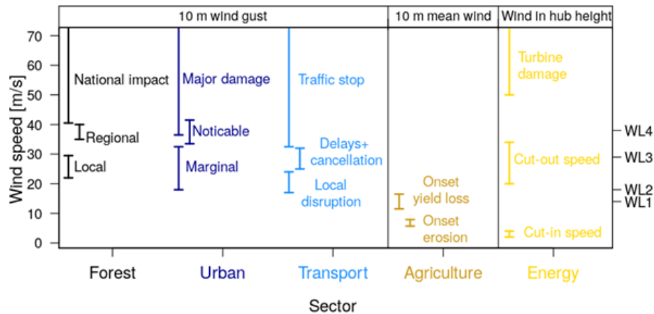
Figure 3. Critical threshold ranges of wind speed (mean wind speed (averaging interval 1 h) and wind gusts) for five affected sectors. Warning levels (WL1–4 at speeds of 14, 18, 29 and 39 m s -1 , respectively) of the DWD for wind gusts (Primo, 2016) are marked on the right axis. For each sector different ranges of critical mean wind speed from the literature are plotted, to show the mean wind speed (or gust), where impacts are expected. Thresholds in the first three sectors (forest, urban areas and transport) refer to wind gusts at 10 m height. For agriculture we present the mean wind speed at 10 m height, and the shown thresholds for the energy sector refer to the mean wind speed measured at the height of the wind turbines (wind in hub height). The upper bar (e.g. “National impact”) is left open as damage will occur also at higher wind speeds. The threshold ranges mean the following: (1) forest local – limited area of damage; forest regional – damage level is meaningful for the affected forest and short-term forest planning and timber price; forest national – damage can occur across several countries. (2) Urban marginal: light objects, tiles can be lifted or come loose. Urban noticeable: heavier objects are lifted, and first damage to individual building components is possible. Urban major: large vehicles overturn; roofs are severely damaged. (3) Transport local disruption: blocked roads through windthrow or sliding containers at ships. Transport delays: cancellation through electricity cuts and increasing number of wind-related accidents. Transport traffic stop: damage of overhead cables and longer power failures as well as airport and harbour closures. (4) Agriculture erosion: soil loss to wind erosion. Agriculture yield loss: damage to leaves and yield loss due to lodged fields. (5) Energy cut-in speed: start of energy production. Energy cut-out speed: automatic shutdown of wind turbines.
