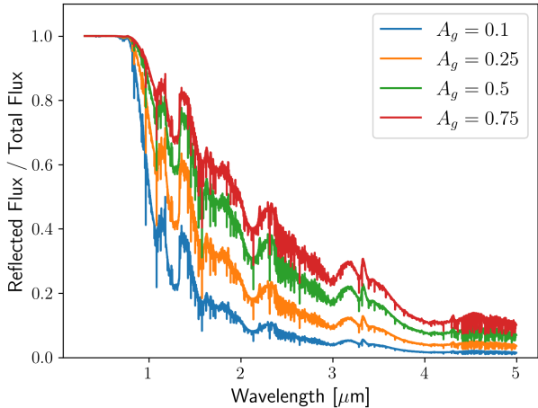
Fig. 6. Contribution of reflected light to the total planetary flux for different grey geometric albedos as a function of wavelength. For the stellar emission spectrum a PHOENIX model (Husser et al. 2013) with the parameters T_{\text{eff}} = 5000 K, [M/H] = 0.0 , and \log g = 4.5 was used. To model the planetary atmosphere an irradiated atmosphere model provided by Mollière et al. (2015) with the parameters T_{\text{eff}} = 1250 K, [Fe/H] = 0.0 , [C/O] = 0.70 , planetary \log g = 3.0 , and stellar spectral type K5 was adopted. The thermal emission from the planet was extrapolated from the dayside temperature of 1192 \pm 9 K, estimated with occultation measurements in the Spitzer 4.5 \mu\text{m} channel (Knutson et al. 2012).
