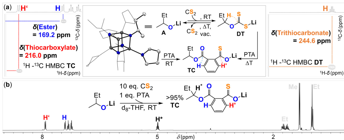
Fig. 2 (a) Reactivity and solid-state structure of model alkoxide A; 1 H- 13 C HMBC (d 8 -THF, 25 °C, 500 MHz) NMR spectra of TC and DT; (b) 1 H NMR spectrum (d 8 -THF, 25 °C, 400 MHz) of products obtained from the reaction of A with a 10 : 1 mixture of CS 2 and PTA.
