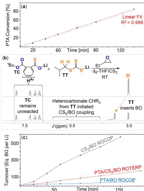
Fig. 6 (a) Linear fit of the PTA conversion vs. time at 1 eq. LiOBn: 100 eq. PTA: 800 eq. BO: 1600 eq. CS 2 at RT. (b) Competition experiment reacting a 1:1 mixture of TC and TT with 1 eq. BO at room temperature in d 8 -THF (overlaid 400 MHz 1 H NMR shown); note that the previously reported 1 Bu derivative of TC was employed to avoid signal overlap. 49 (c) Comparison of the BO turnover versus time for ROTERP and the two parent ROCOP reactions as outlined in the main text; TOF as discussed in the main text obtained by linear fitting over the entire displayed range.
