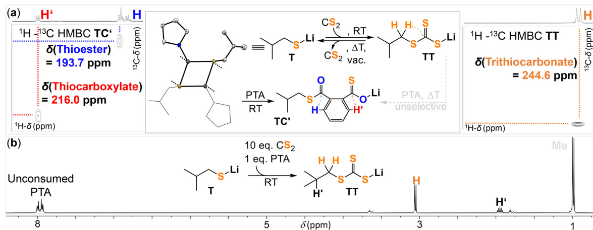
Fig. 3 (a) Reactivity and solid-state structure of model thiolate T; 1 H- 13 C HMBC (d 8 -THF, 25 °C) NMR spectra of TT and TC'; (b) 1 H NMR spectrum (d 8 -THF, 25 °C, 400 MHz) of the reaction products of T with a 10 : 1 mixture of CS 2 and PTA.
